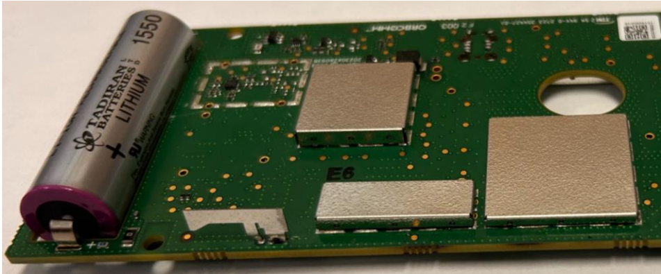
BLE Antenna on the PCB Board
