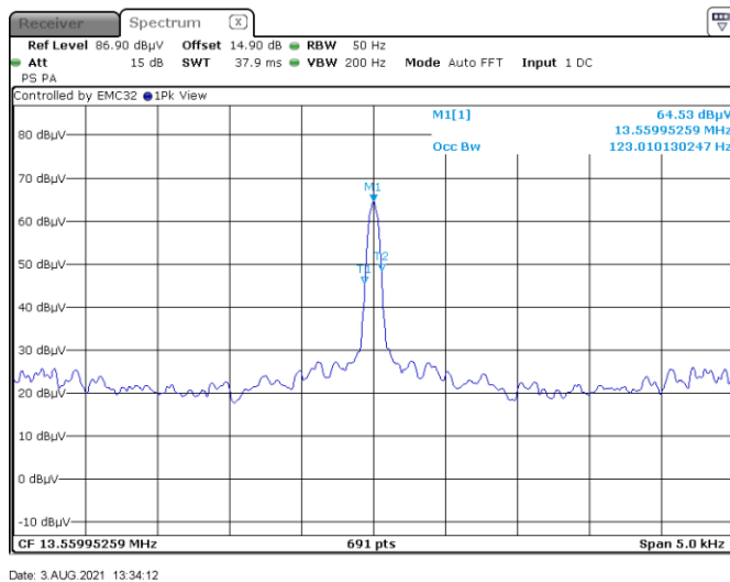
Figure 8.4-1: 99% bandwidth
