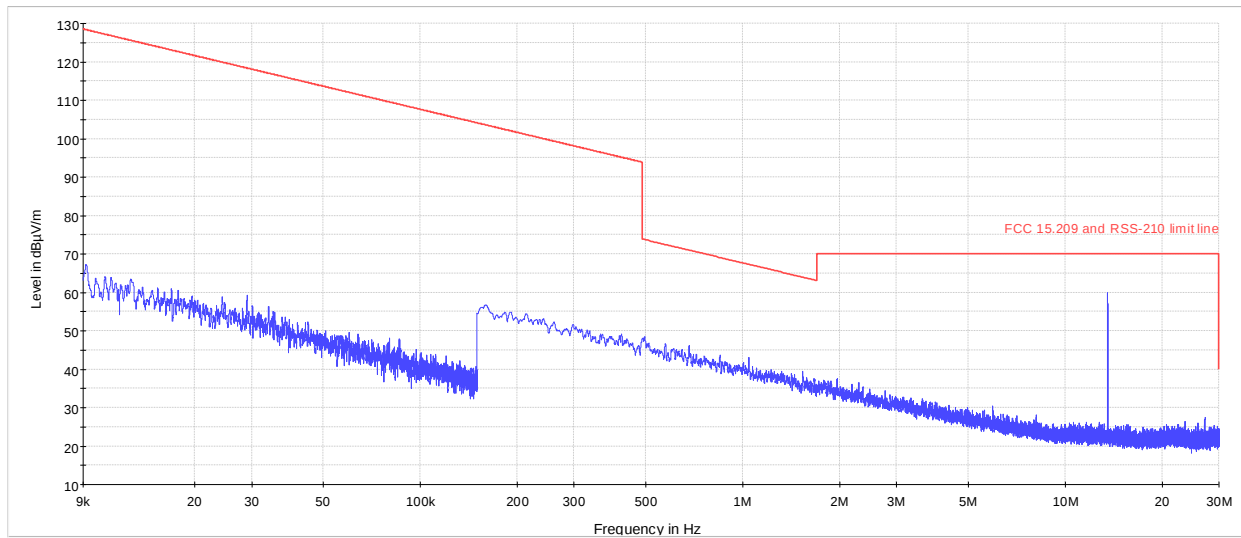
Figure 8.6-1: Field strength of spurious emissions below 30 MHz
