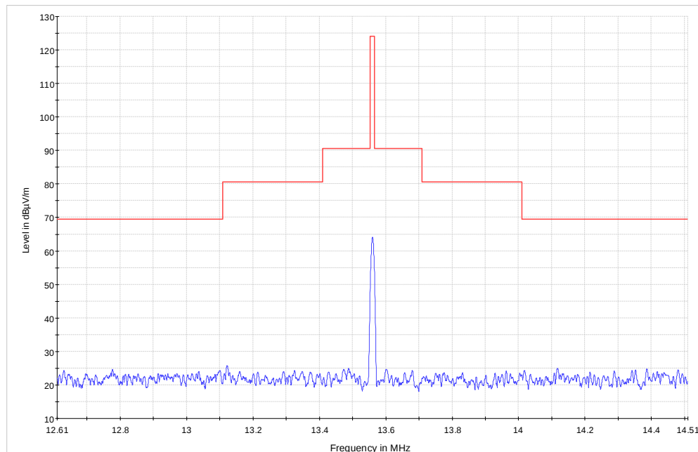
Figure 8.5-3: Field strength within 13.110–14.010 MHz band
