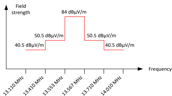
Figure 8.5-1: In-band spurious emissions limit at 30 m
