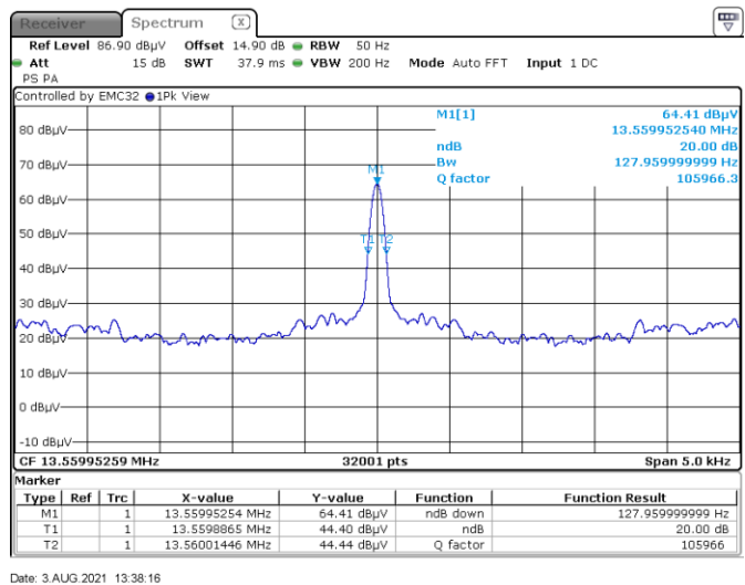
Figure 8.4-2: 20 dB bandwidth
