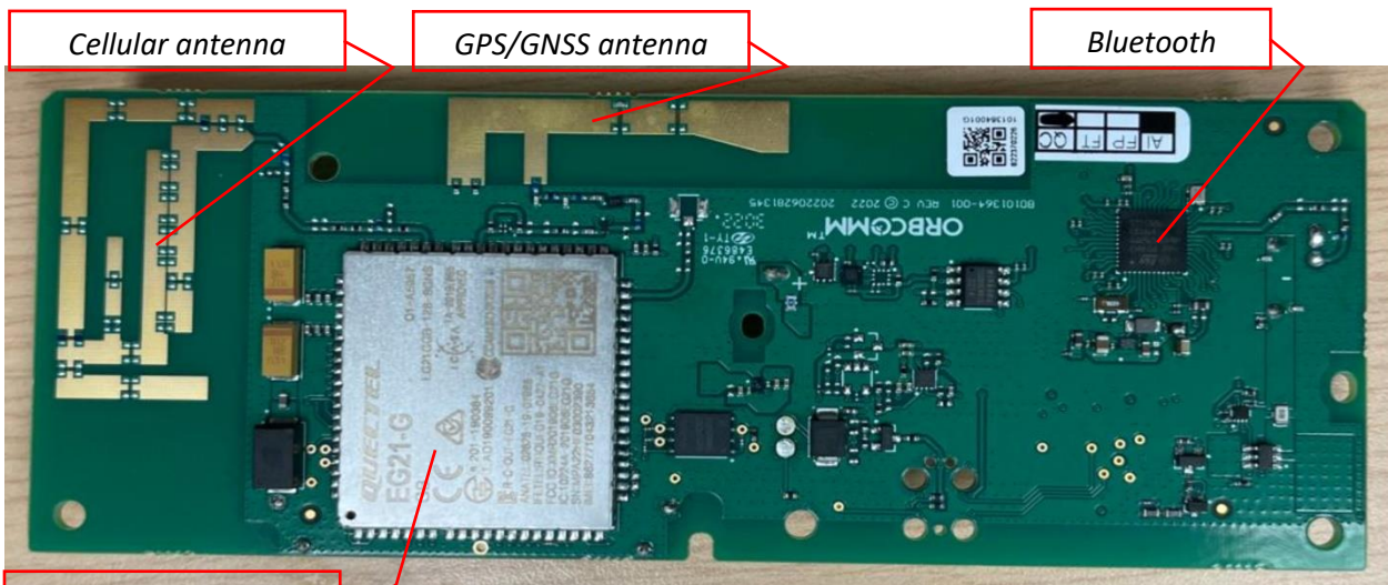
Internal circuit card top view
