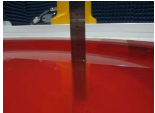
Fig. 9.8 Photo of Liquid Height for Body SAR (5000MHz~6000MHz) (depth>15cm)
