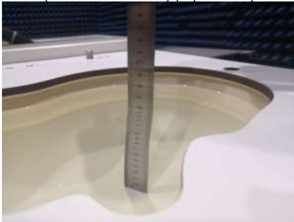
Fig. 9.7 Photo of Liquid Height for Head SAR (5000MHz~6000MHz) (depth>15cm)
