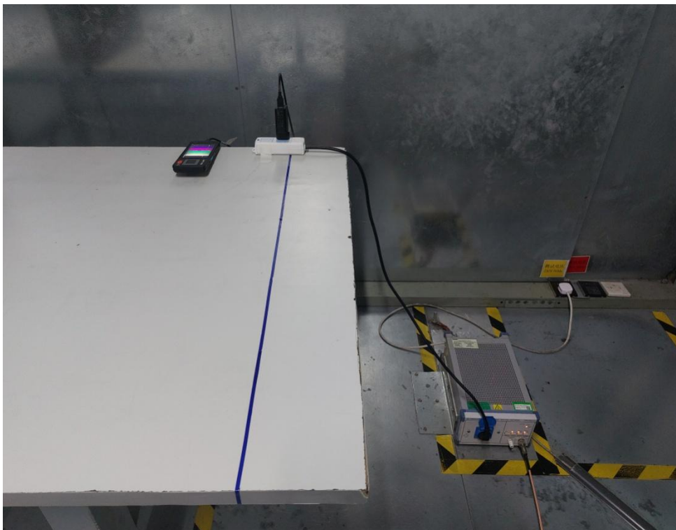
AC Conducted Measurement Photos
