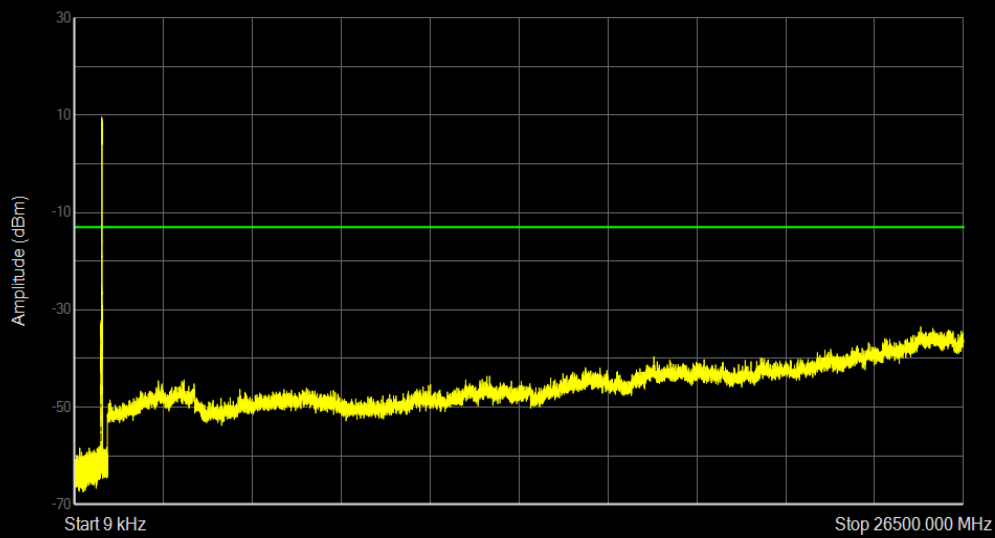
Band26(824-849) QAM16 BW=15MHz Channel=26915 RB Size=75 Position=#0
