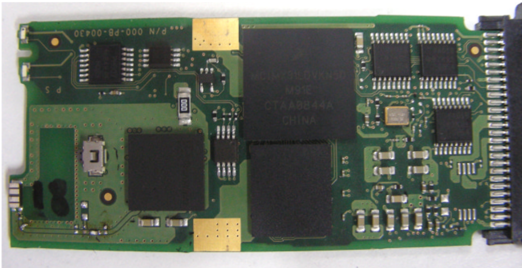
Photograph No.1 ConstantConnect and Protect card internal top view
