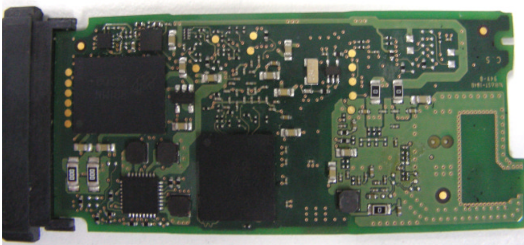
Photograph No.2 ConstantConnect and Protect card second side view
