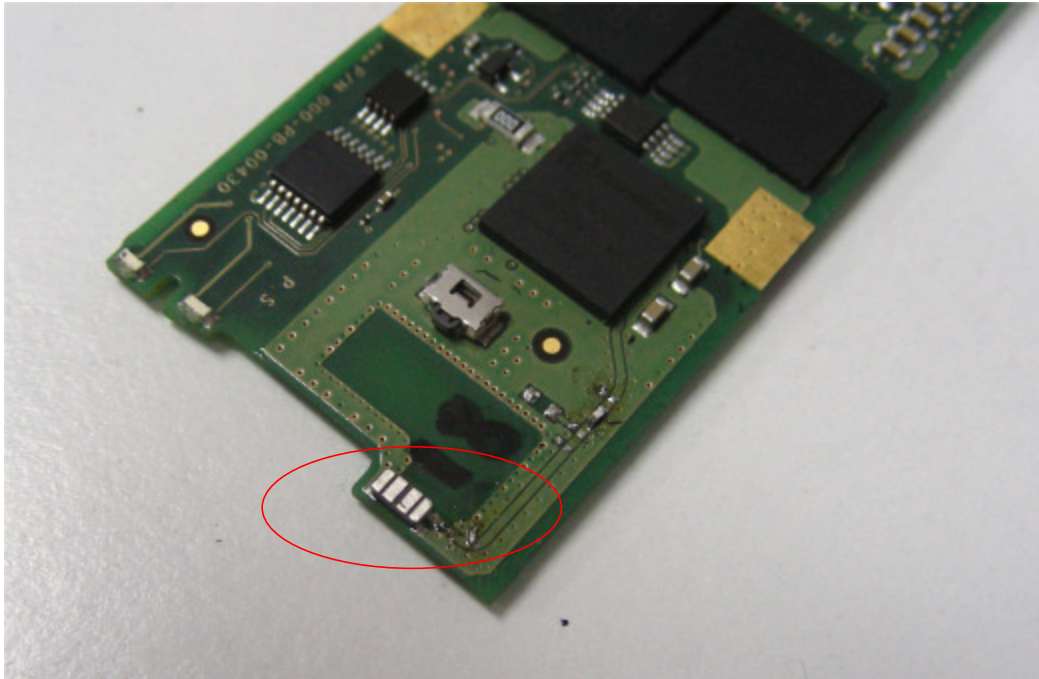
Photograph No.3 ConstantConnect and Protect card antenna
