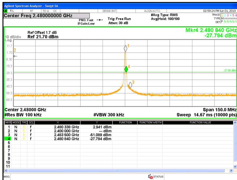
Figure 18: Conducted Band Edge-2480 MHz- Headset
