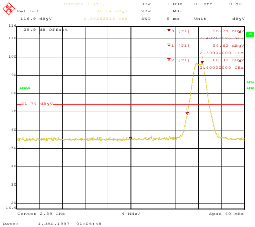
Figure 24: Band-edge-2402 MHz-H-Pk
