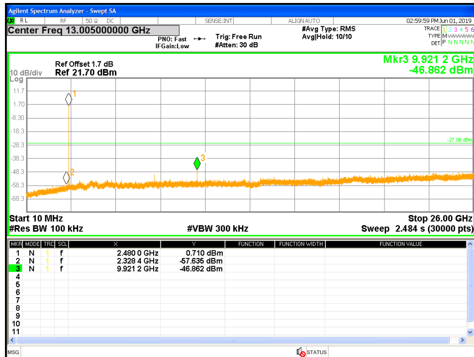
Figure 19: Out of band Emission-2480 MHz- Headset
