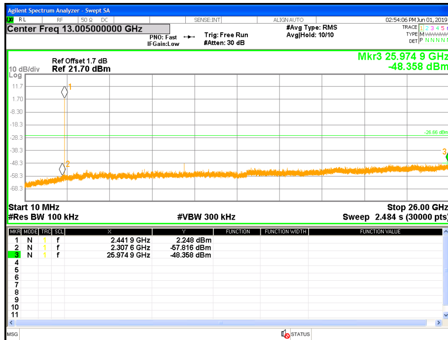
Figure 17: Out of band Emission-2442 MHz- Headset
