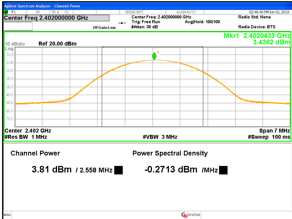
Figure 2: Maximum Conducted Output Power, 2402 MHz- Wireless Headset
