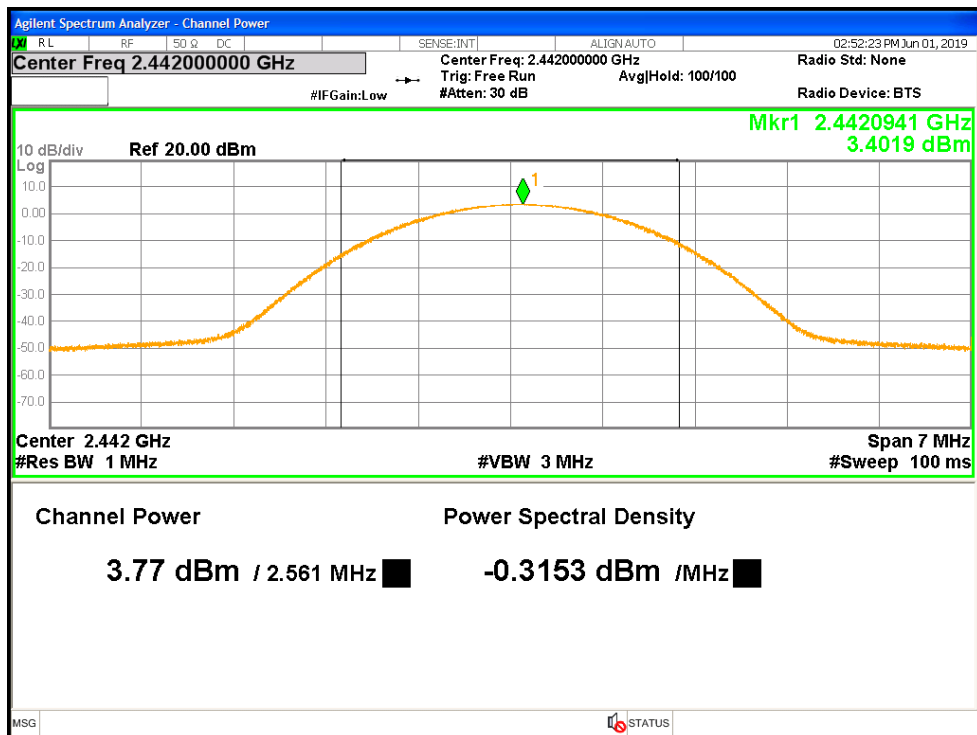
Figure 3: Maximum Conducted Output Power at 2442 MHz - Wireless Headset
