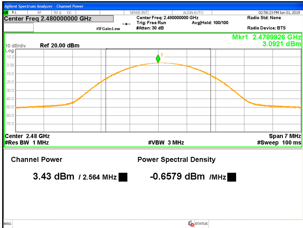
Figure 4: Maximum Conducted Output Power at 2480 MHz - Wireless Headset
