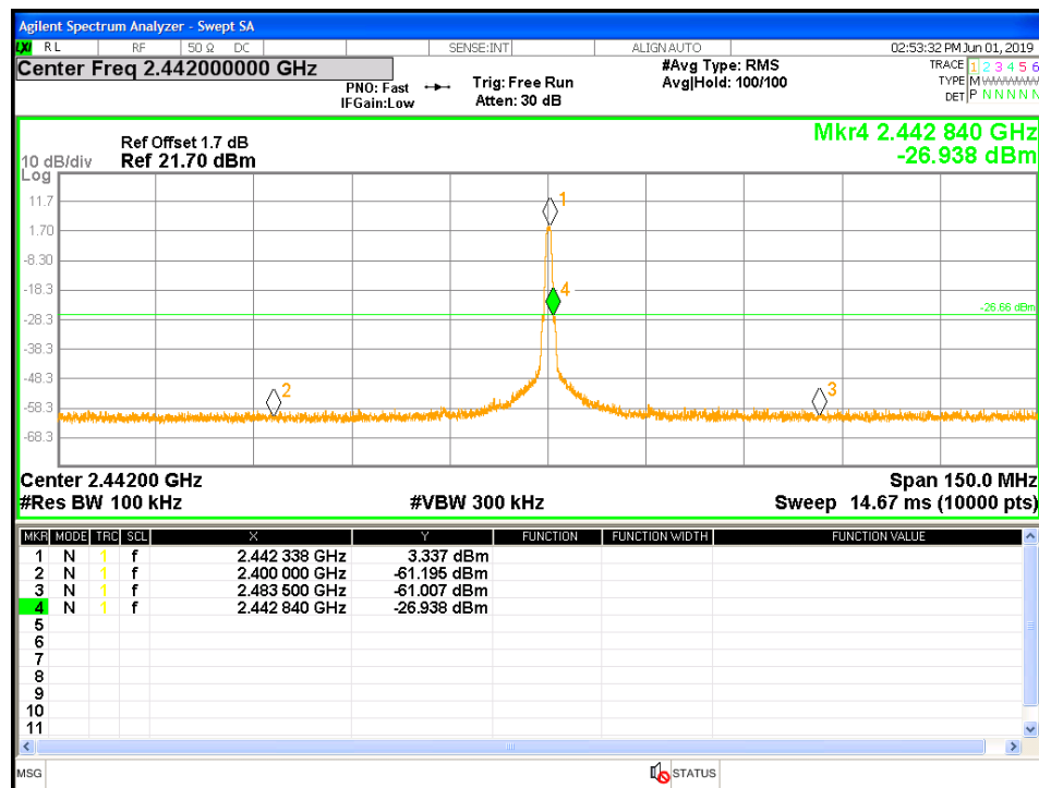
Figure 16: Conducted Band Edge-2442 MHz- Headset
