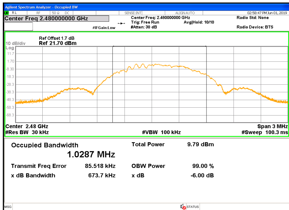
Figure 10: 99% Bandwidth-Transmitter -2480 MHz
