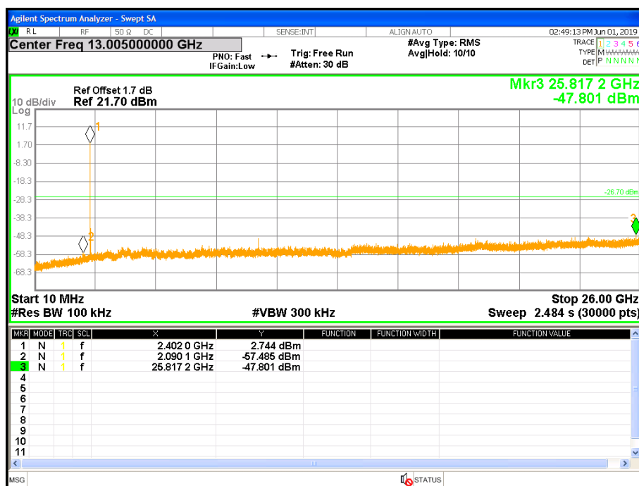
Figure 15: Out of band Emission-2402 MHz- Headset
