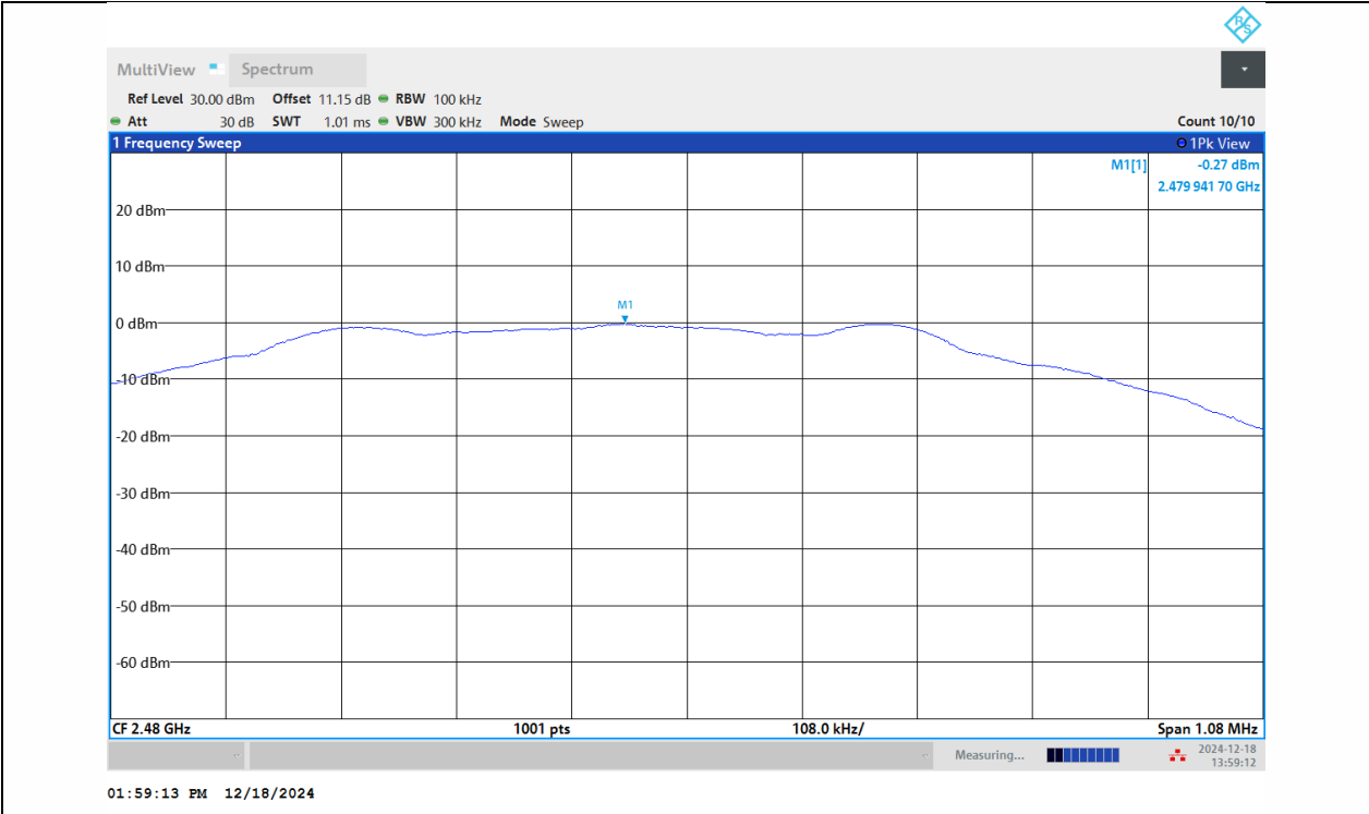
BLE_1M-Ant1-2480-PASS
