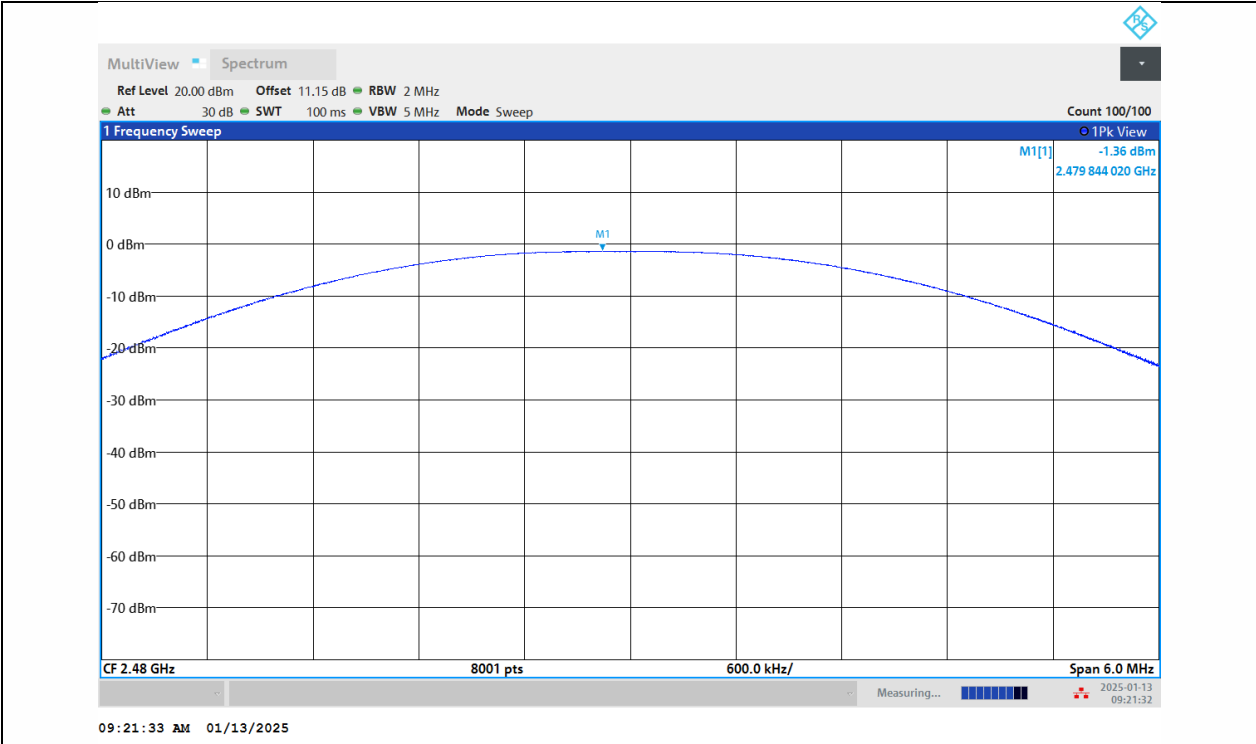
BLE_1M-Ant1-2480-PASS
