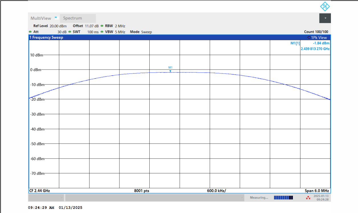
BLE_2M-Ant1-2440-PASS
