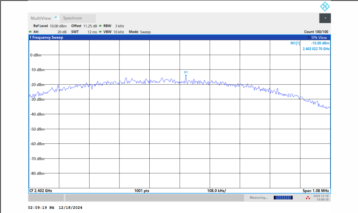
BLE_1M-Ant1-2402-PASS
