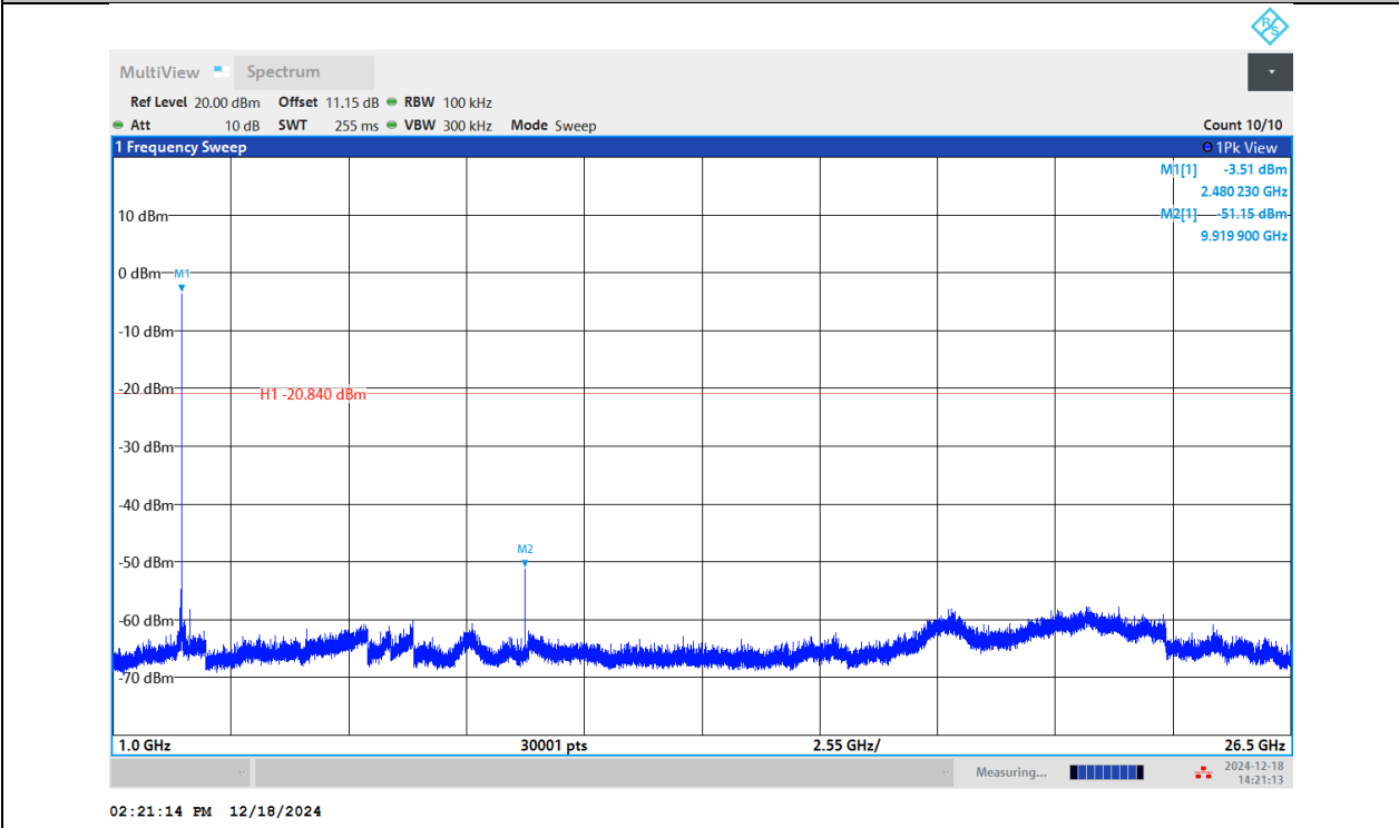
BLE_2M-Ant1-2480-1000~26500-PASS
