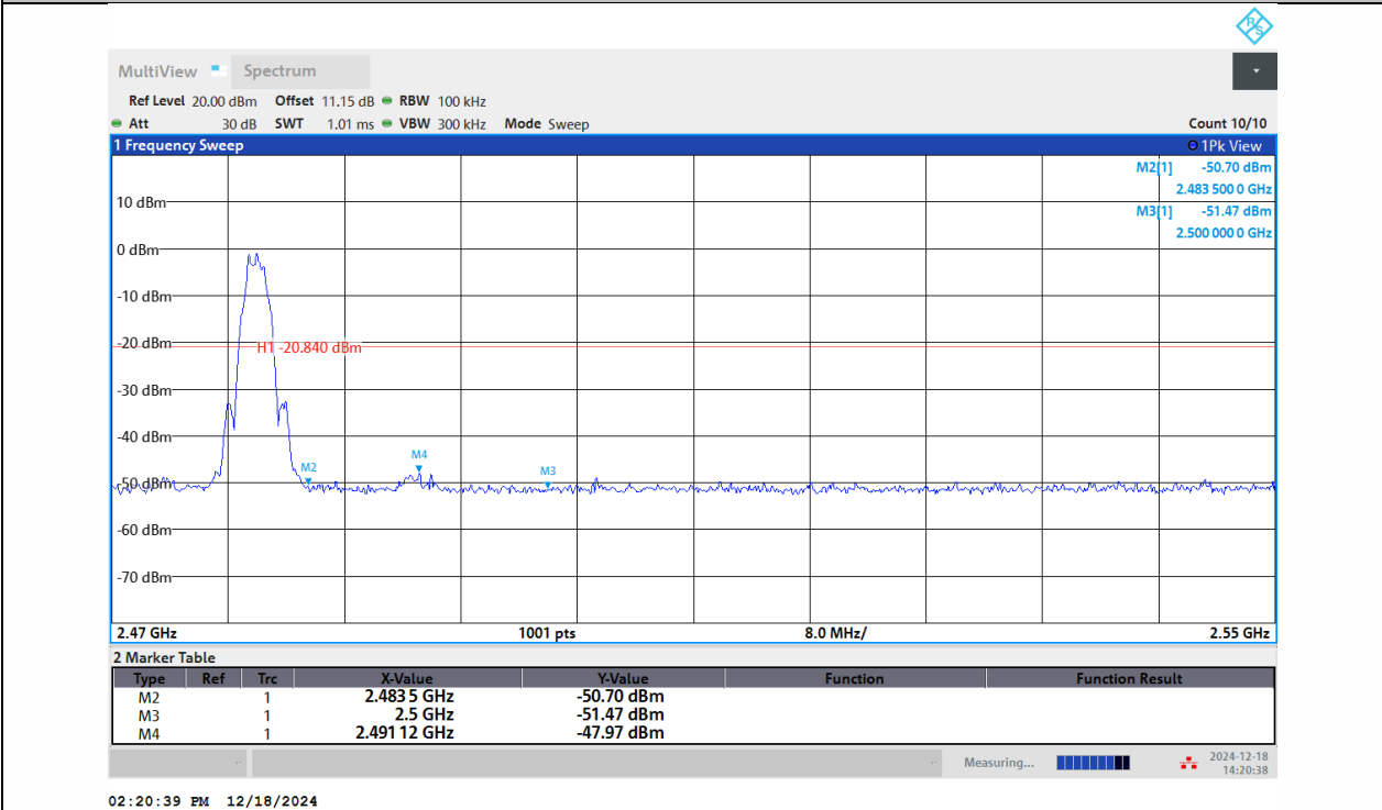
BLE_2M-Ant1-2480-PASS
