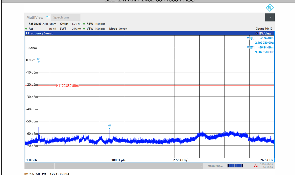
BLE_2M-Ant1-2402-1000~26500-PASS
