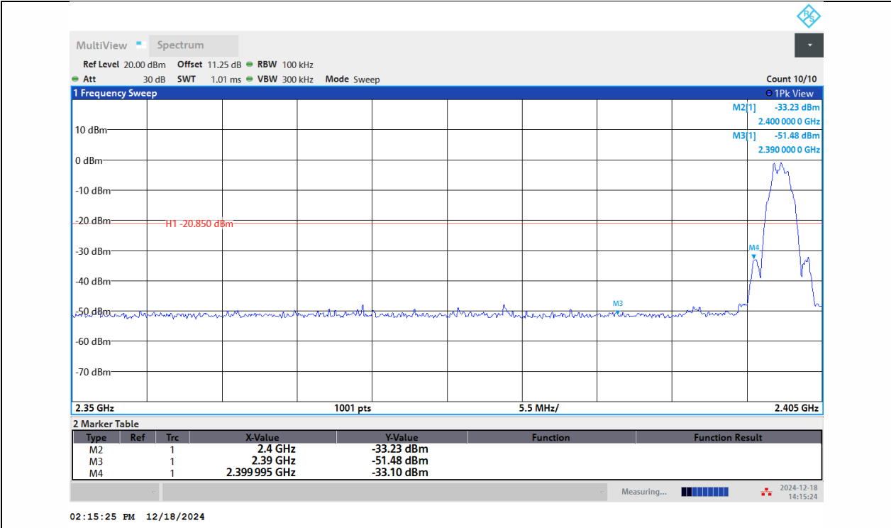
BLE_2M-Ant1-2402-PASS
