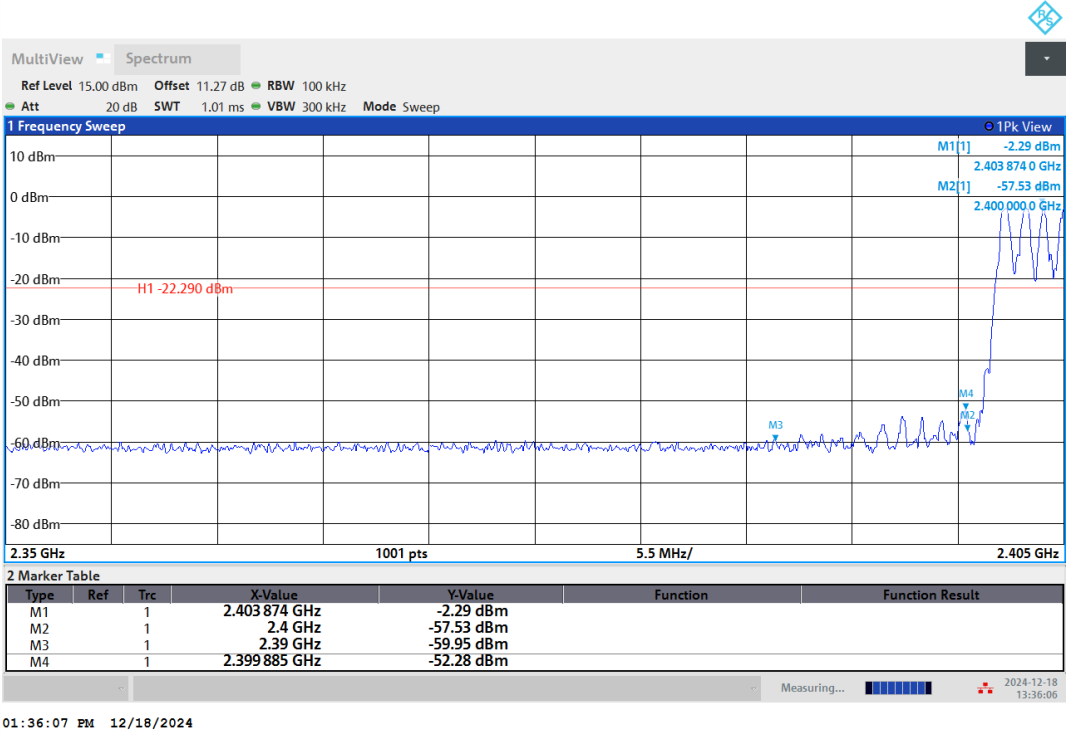
SRD-Ant1-Hop_2402-PASS
