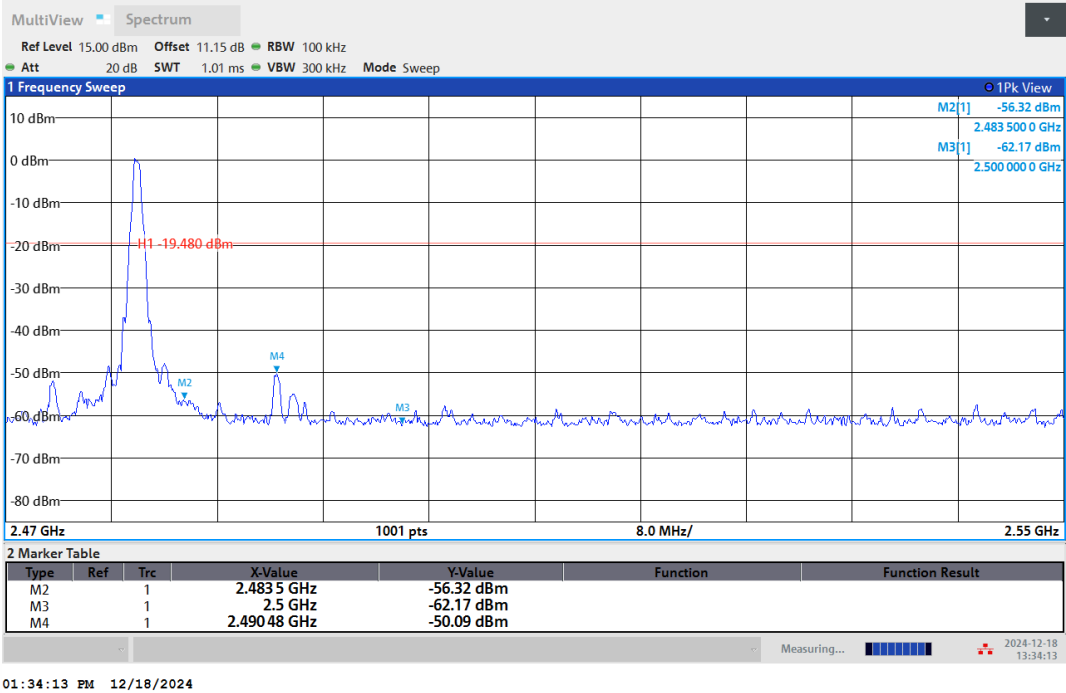
SRD-Ant1-2480-PASS
