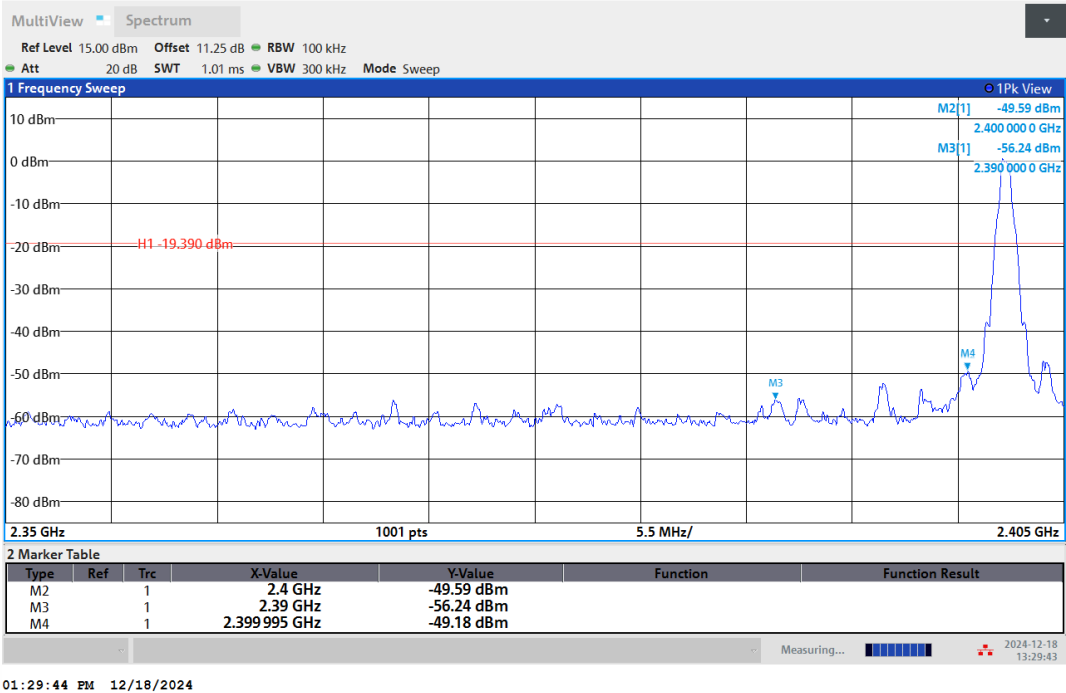
SRD-Ant1-2402-PASS
