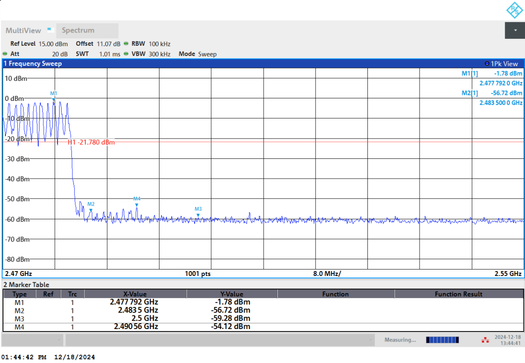
SRD-Ant1-Hop_2480-PASS
