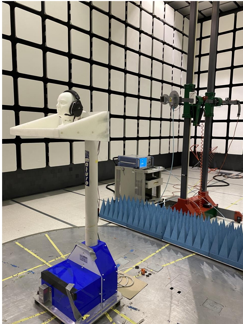
Figure 7: Test Setup for 18 GHz to 40 GHz (Front View)
