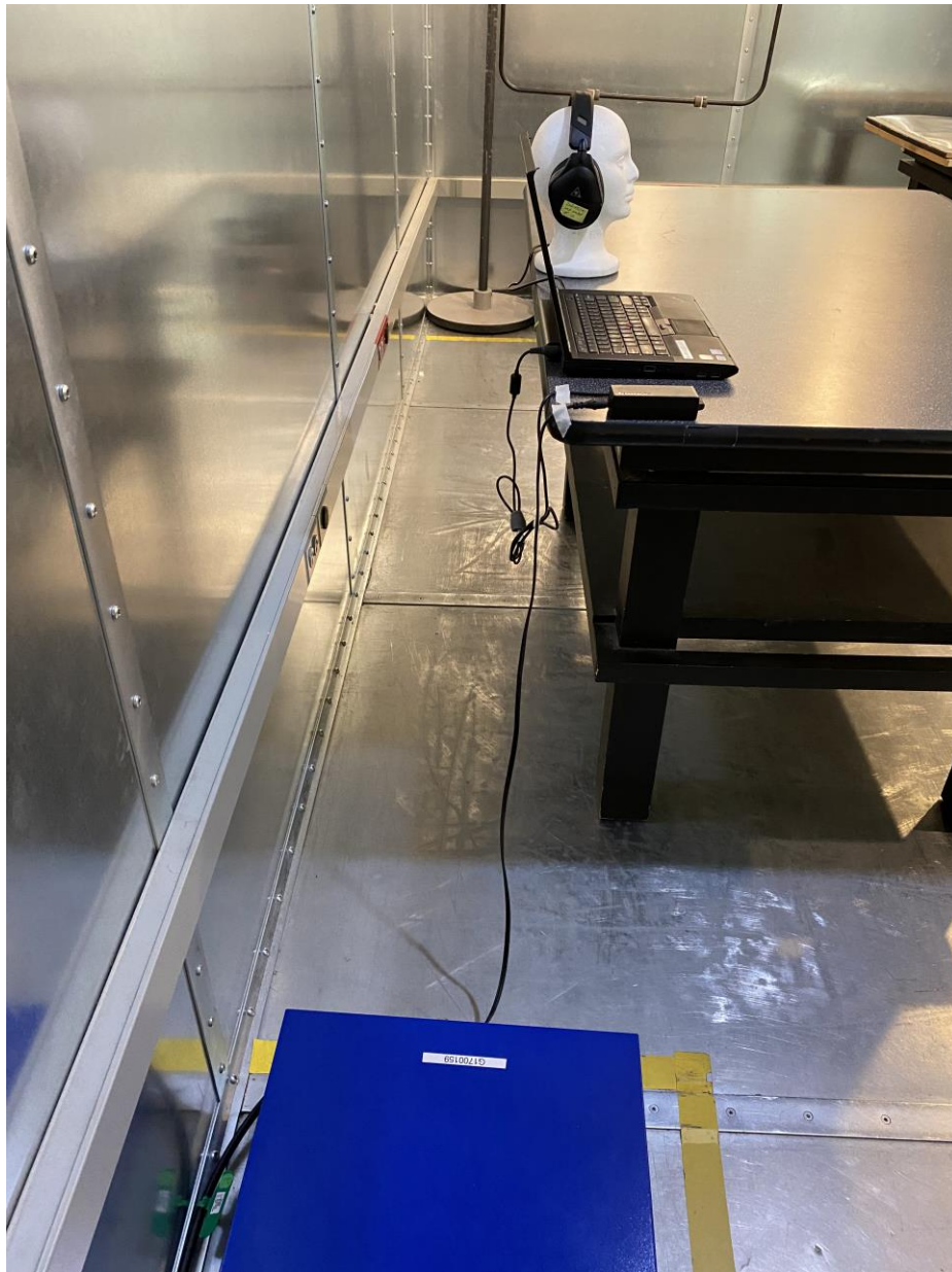
Figure 11: AC Conducted Emission Test Setup (Side View)
