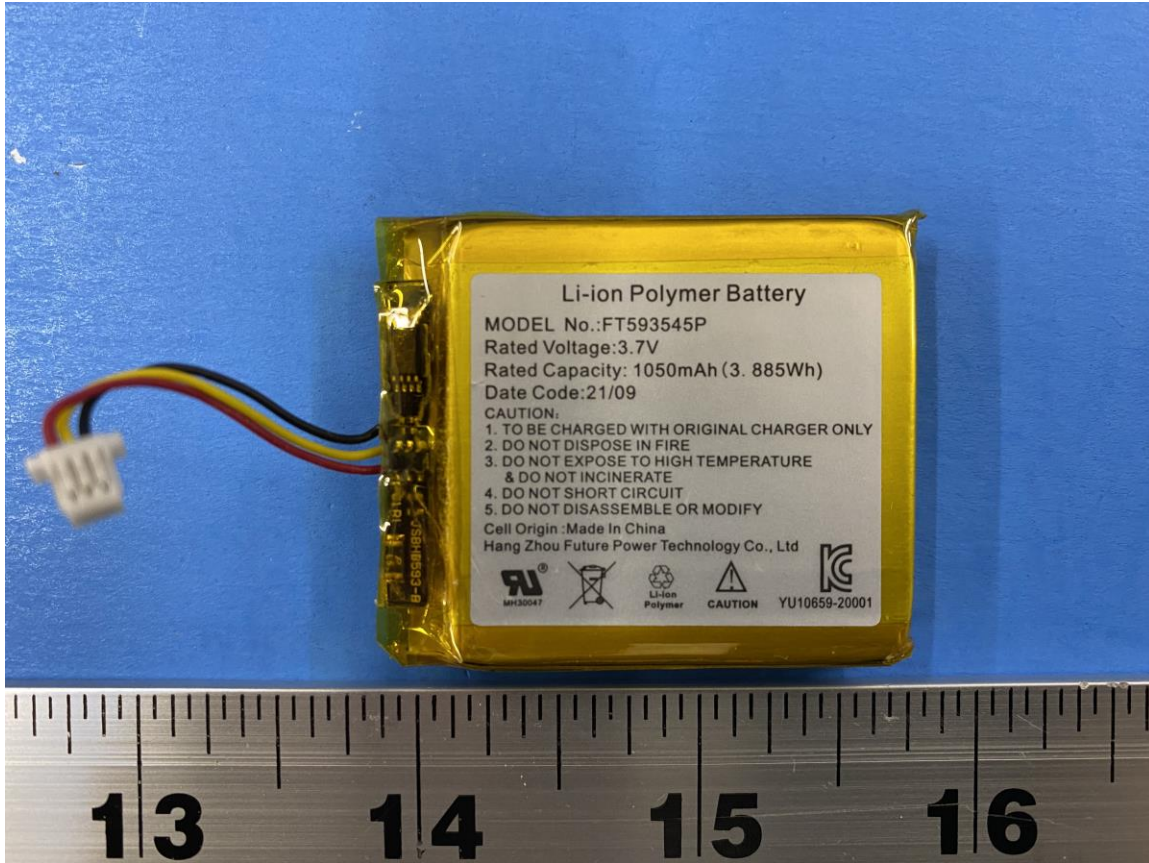
Figure 8: Internal Photo of Stealth 700P Gen 2 RX2 (1050 mAh Battery, Top)
