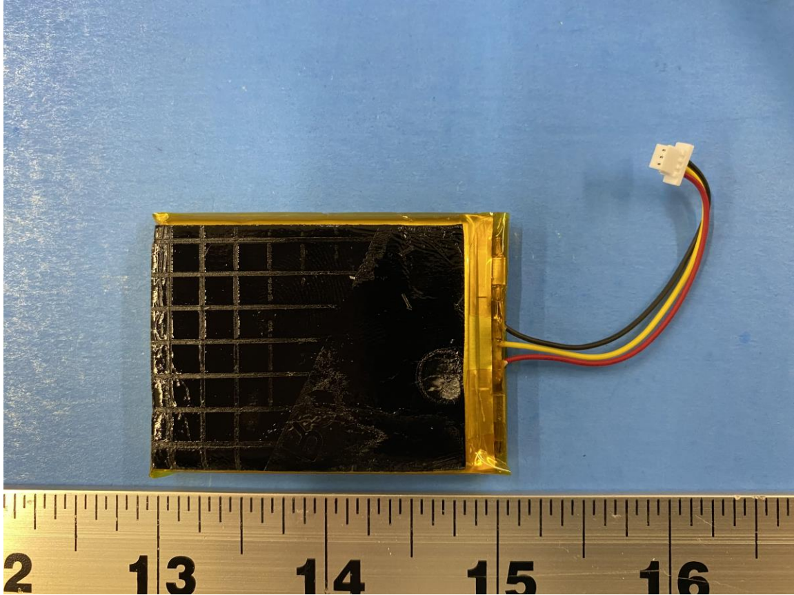
Figure 7: Internal Photo of Stealth 700P Gen 2 RX2 (1400 mAh Battery, Bottom)
