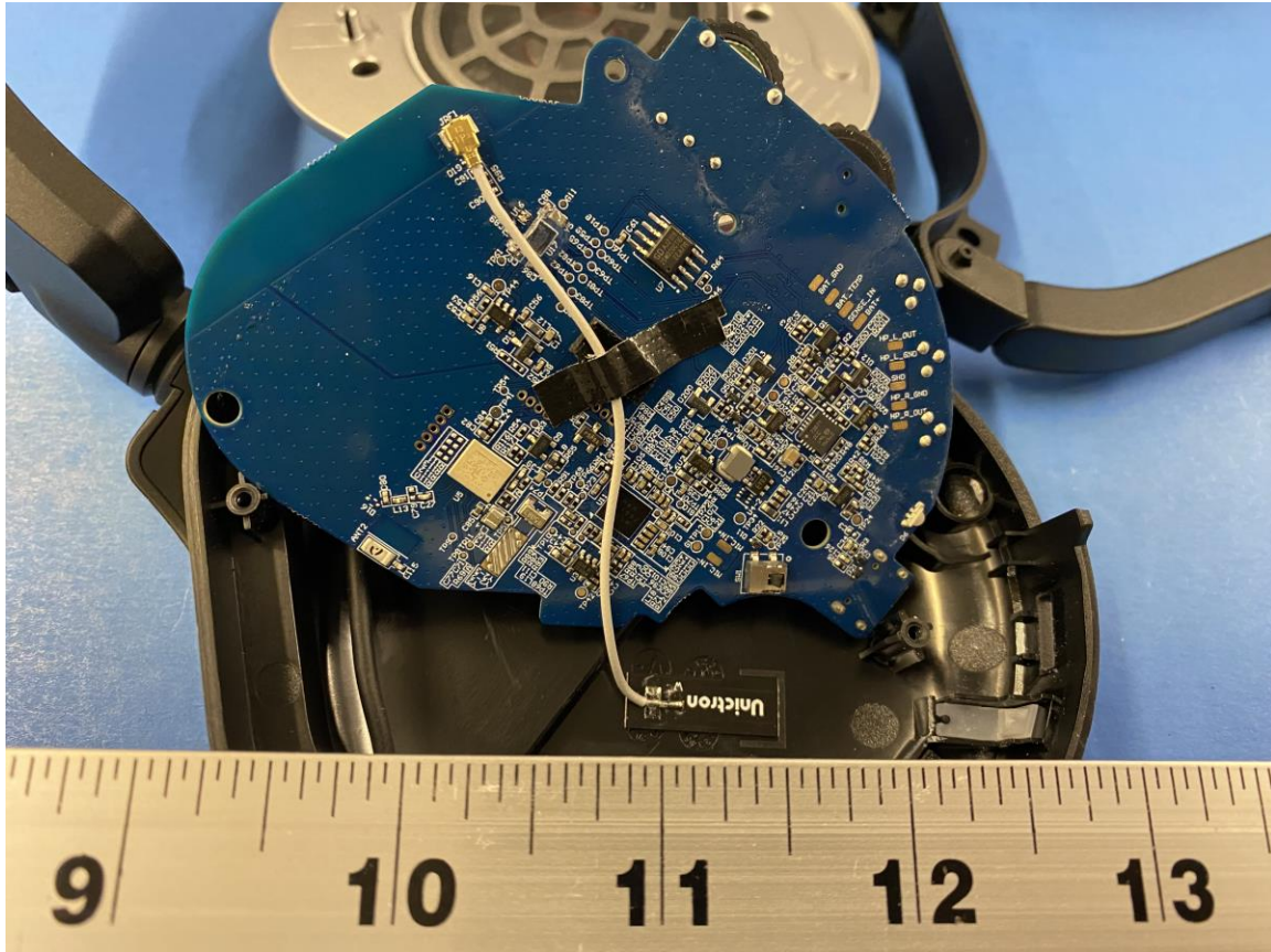
Figure 3: Internal Photo of Stealth 700P Gen 2 RX2 Main PCB (Bottom)
