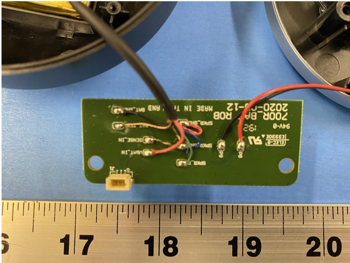
Figure 4: Internal Photo of Stealth 700P Gen 2 RX2 (Right Ear PCB, Top)
