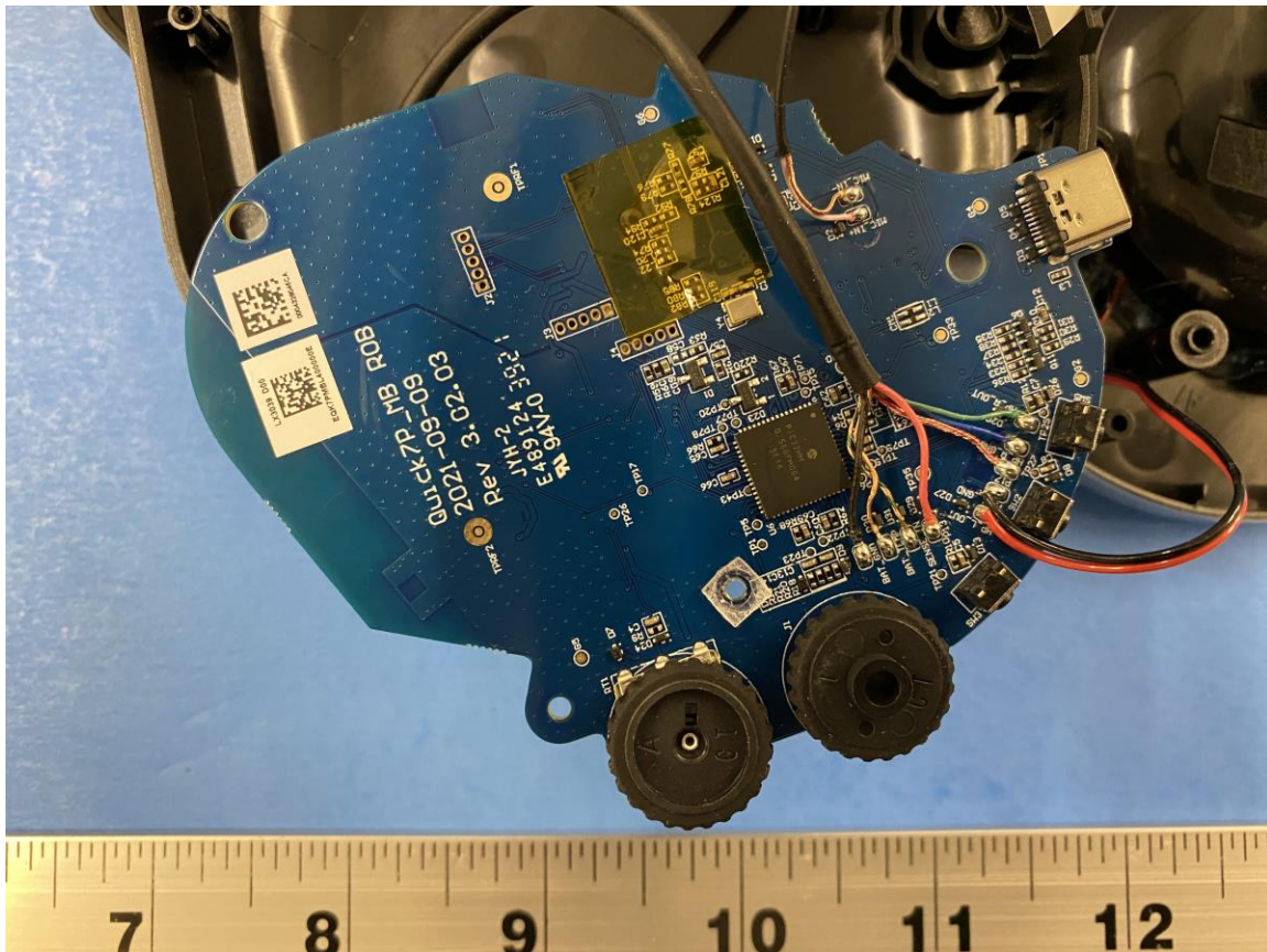
Figure 2: Internal Photo of Stealth 700P Gen 2 RX2 Main PCB (Top)
