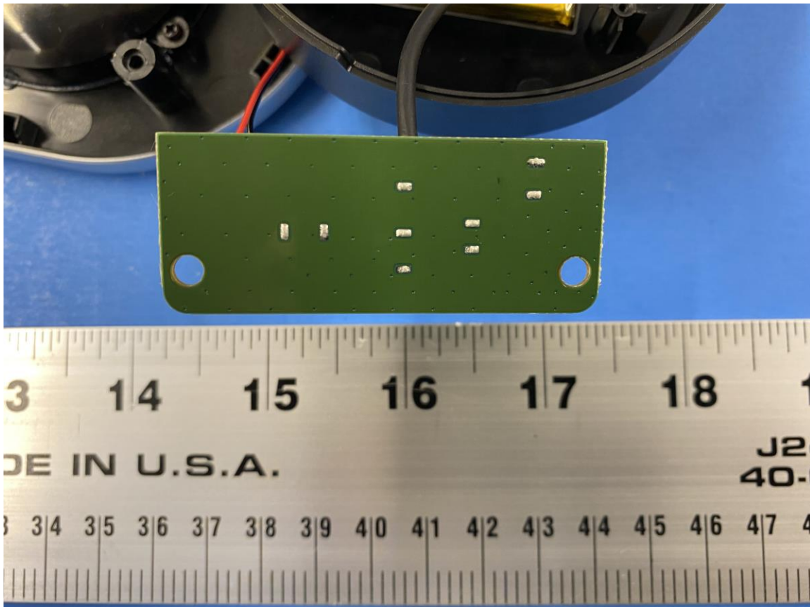
Figure 5: Internal Photo of Stealth 700P Gen 2 RX2 (Right Ear PCB, Bottom)
