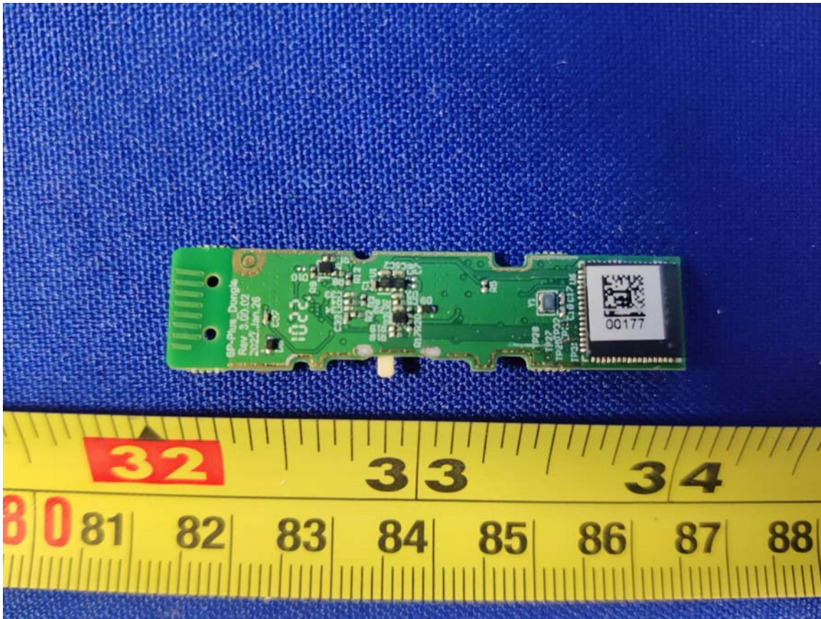
Figure 3: Internal Photo of Stealth600P-MAX-TX – Bottom PCB
