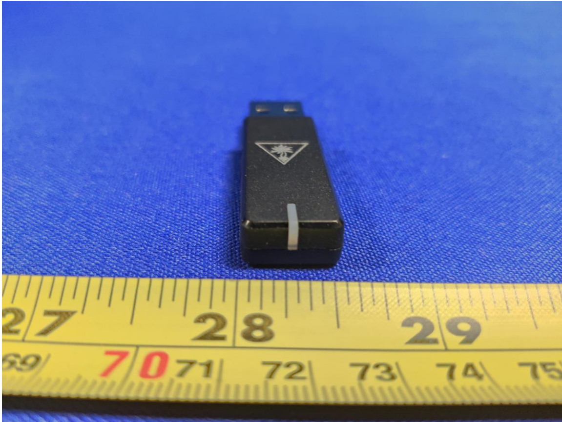
Figure 1: External Photo of Stealth600P-MAX-TX – Front (Black Version)
