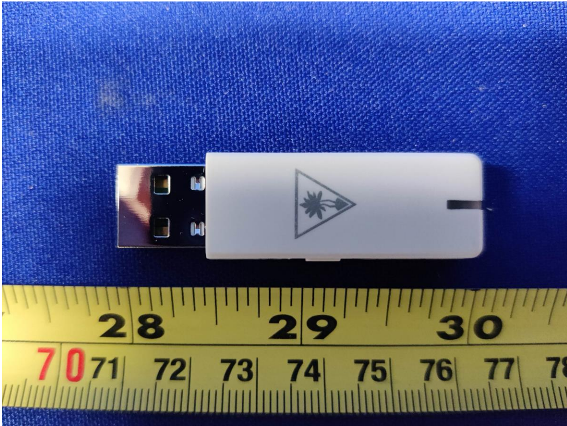
Figure 12: External Photo of Stealth600P-MAX-TX – Top (Artic Camo Version)
