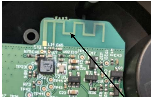
PCB Antenna Trace
