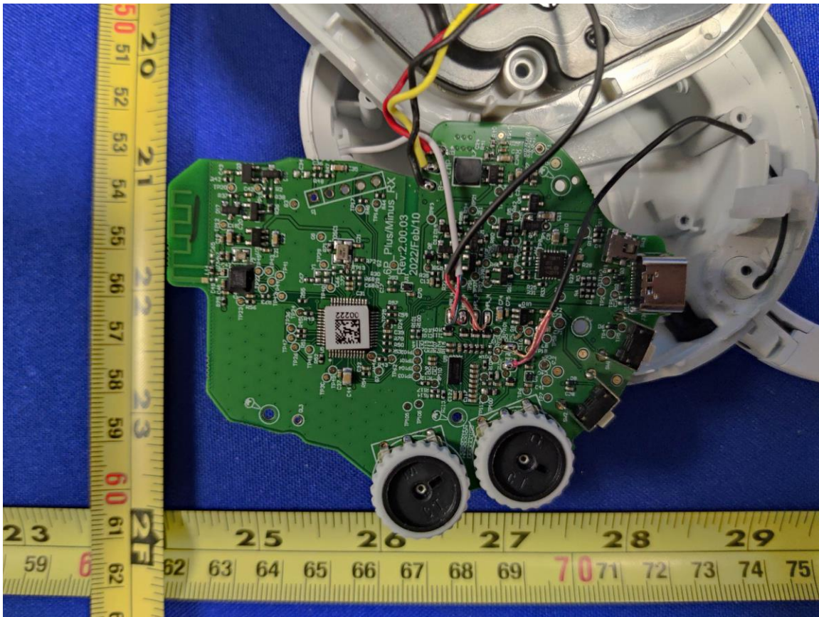
Figure 2: Internal Photo of Stealth600P-MAX-RX – Top PCB
