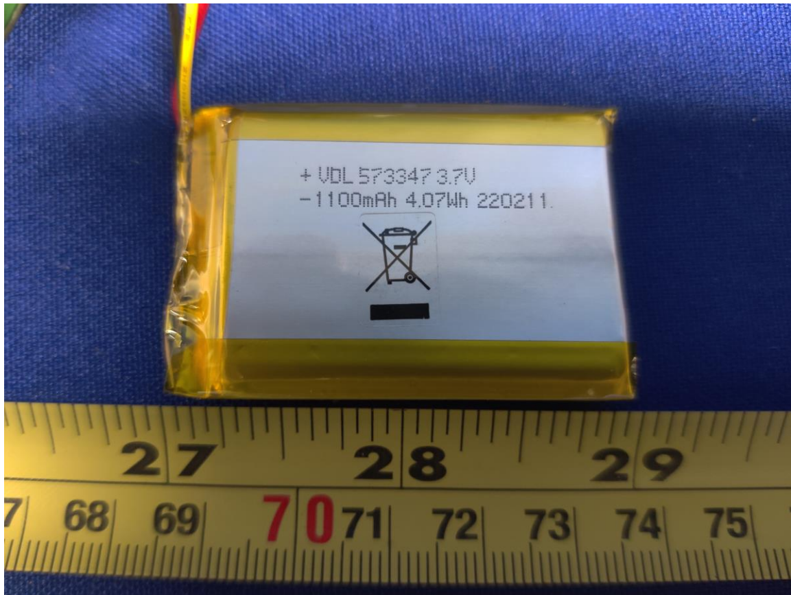
Figure 4: Internal Photo of Stealth600P-MAX-RX – Battery
