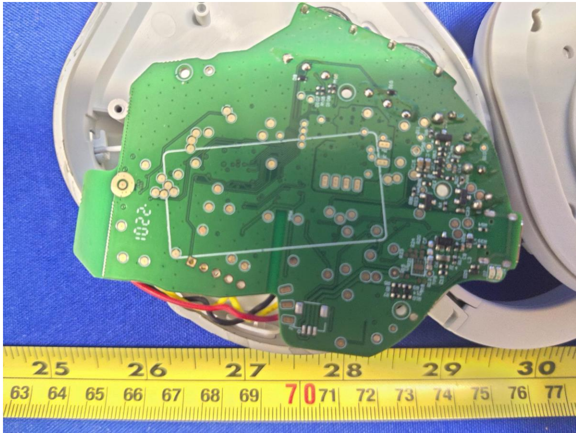
Figure 3: Internal Photo of Stealth600P-MAX-RX – Bottom PCB
