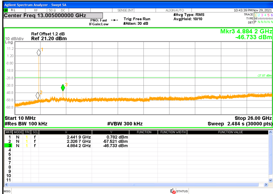
Figure 17: Out of band Emissions at 2442 MHz
