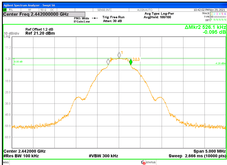
Figure 6: DTS Bandwidth - 2442 MHz
