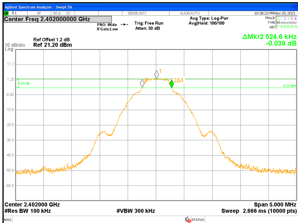
Figure 5: DTS Bandwidth - 2402 MHz
