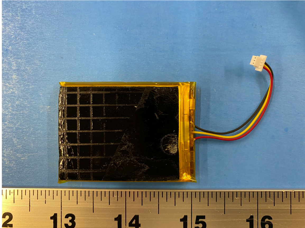
Figure 7: Internal Photo of Stealth700X-MAX-RX (1400 mAh Battery, Bottom)
