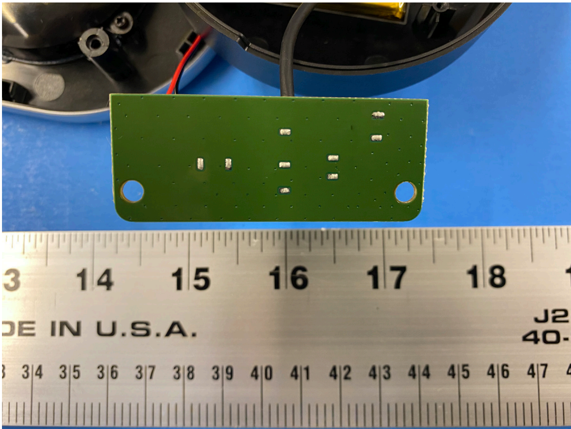
Figure 5: Internal Photo of Stealth700X-MAX-RX (Right Ear PCB, Bottom)
