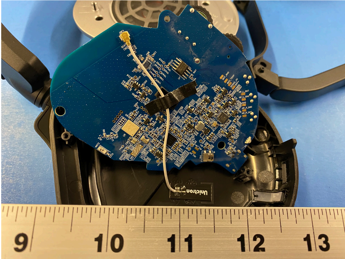
Figure 3: Internal Photo of Stealth700X-MAX-RX (left Ear Main PCB, Bottom)
