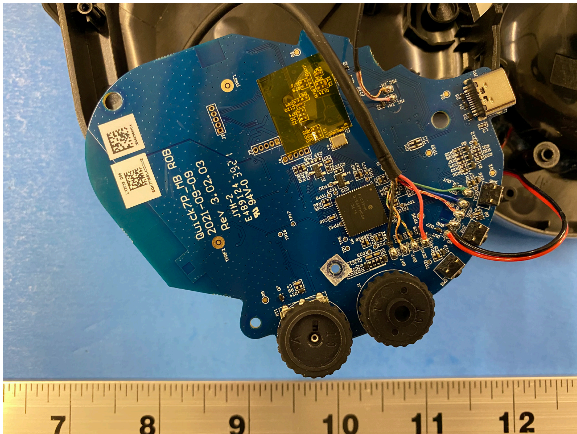
Figure 2: Internal Photo of Stealth700X-MAX-RX (Left Ear Main PCB, Top)
