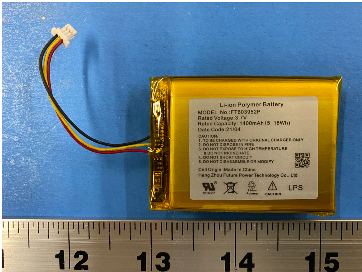
Figure 6: Internal Photo of Stealth700X-MAX-RX (1400 mAh Battery, Top)
