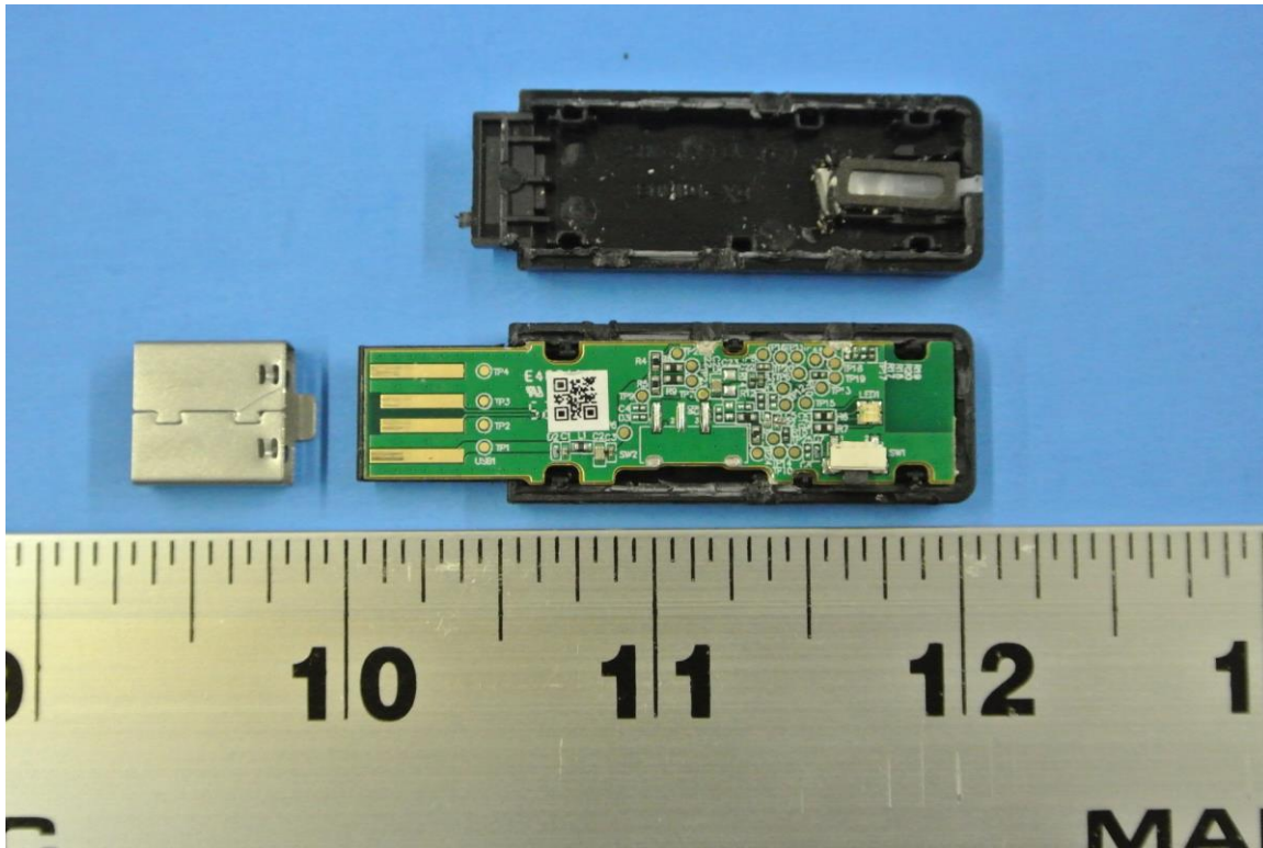
Figure 1: Internal Photo of Stealth600X-USB-TX with Plastic Cover Removed
