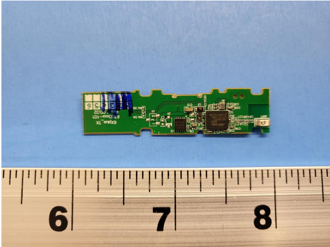
Figure 3: Internal Photo of Stealth600X-USB-TX – Bottom PCB
