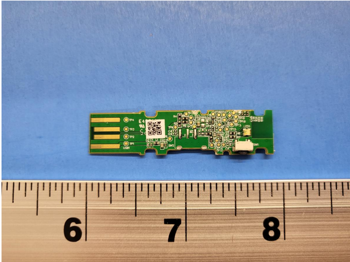
Figure 2: Internal Photo of Stealth600X-USB-TX – Top PCB
