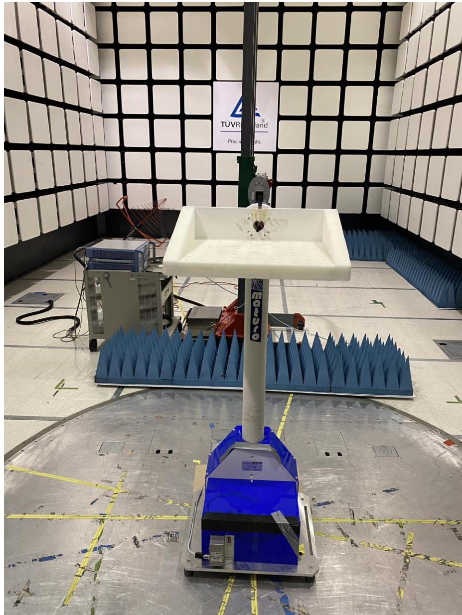
Figure 7: Test Setup for 18 GHz to 26 GHz (Front View)
