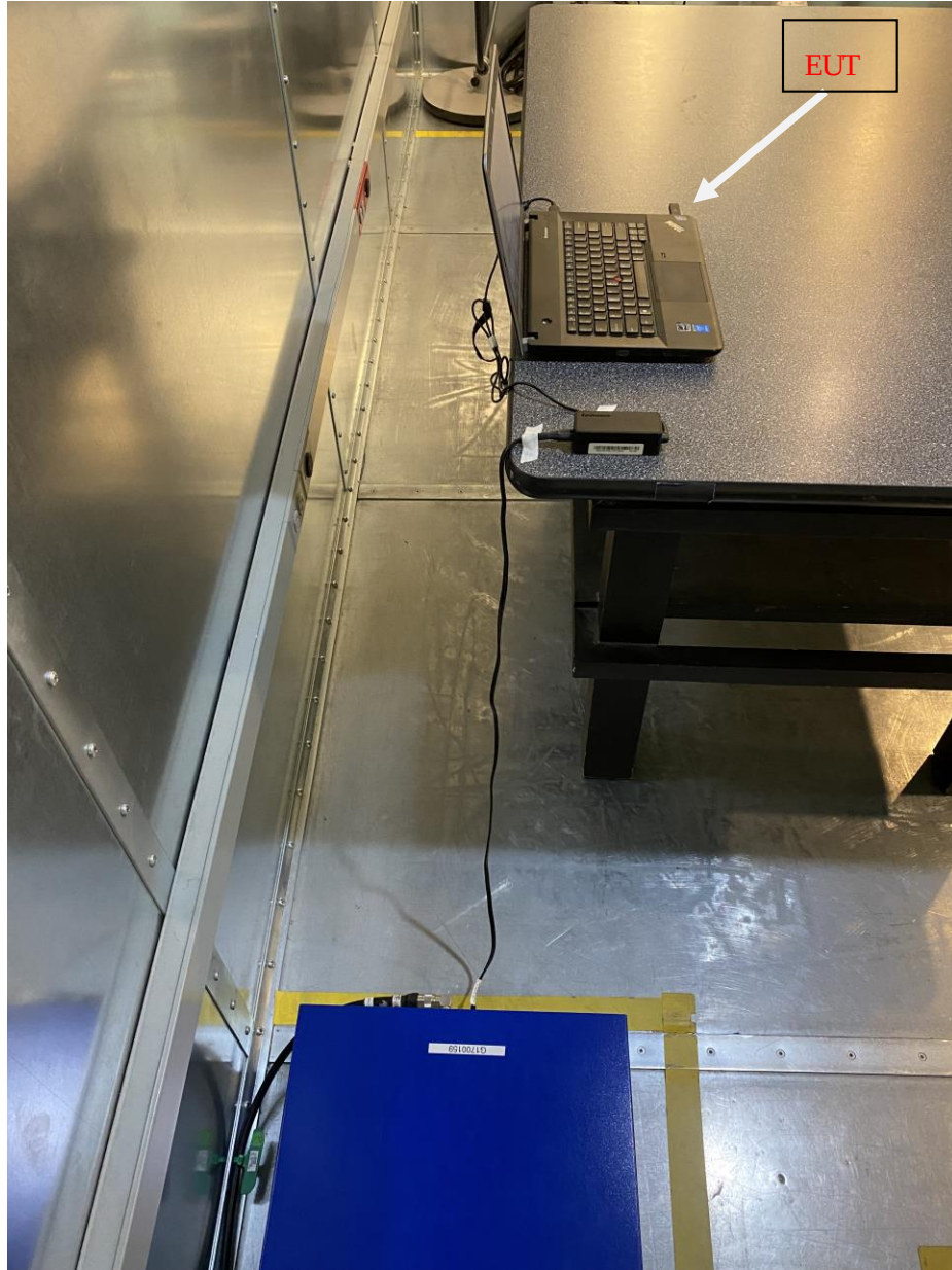
Figure 11: AC Conducted Emission Test Setup (Side)
