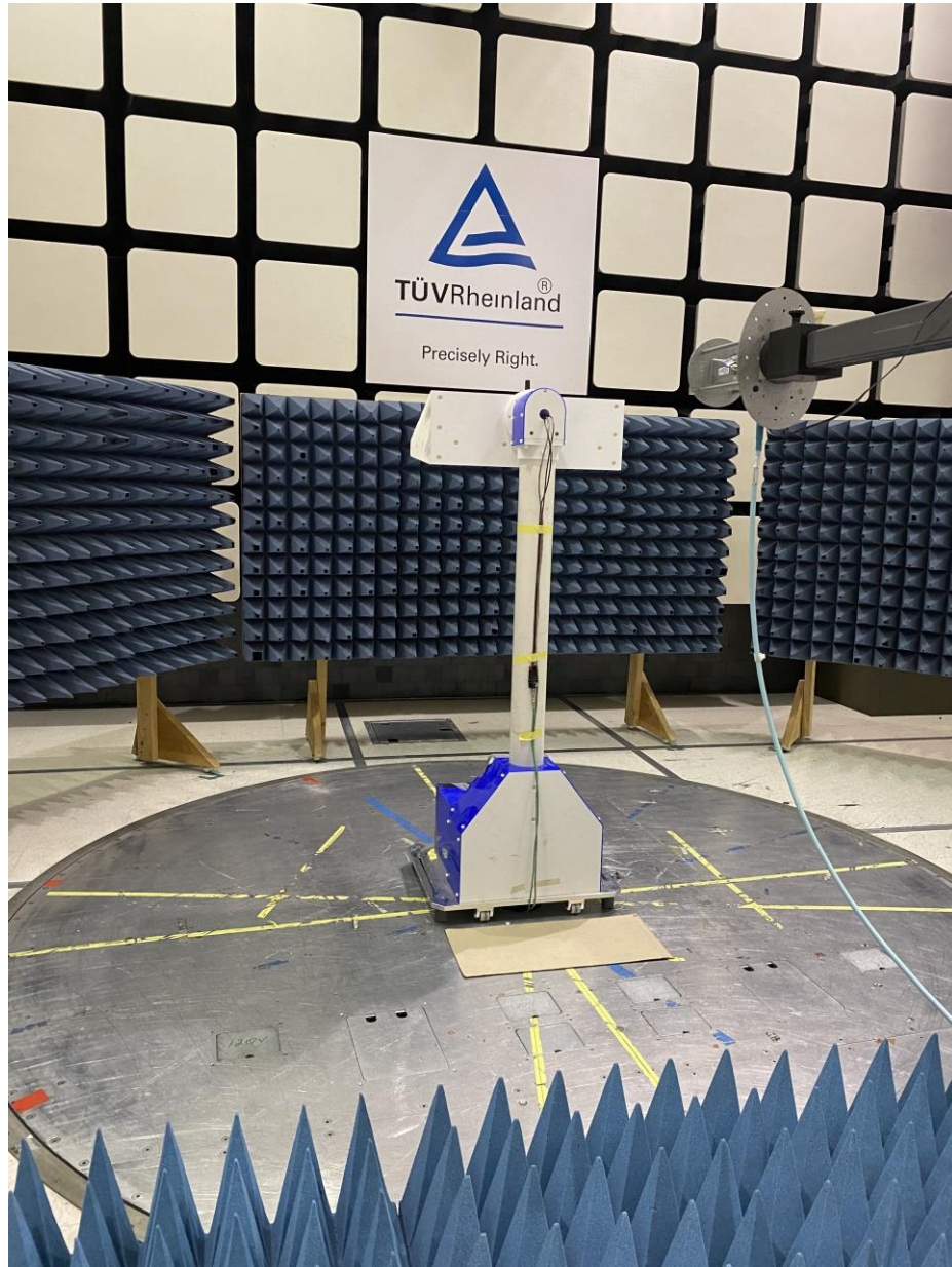
Figure 8: Test Setup for 18 GHz to 26 GHz (Rear View)
