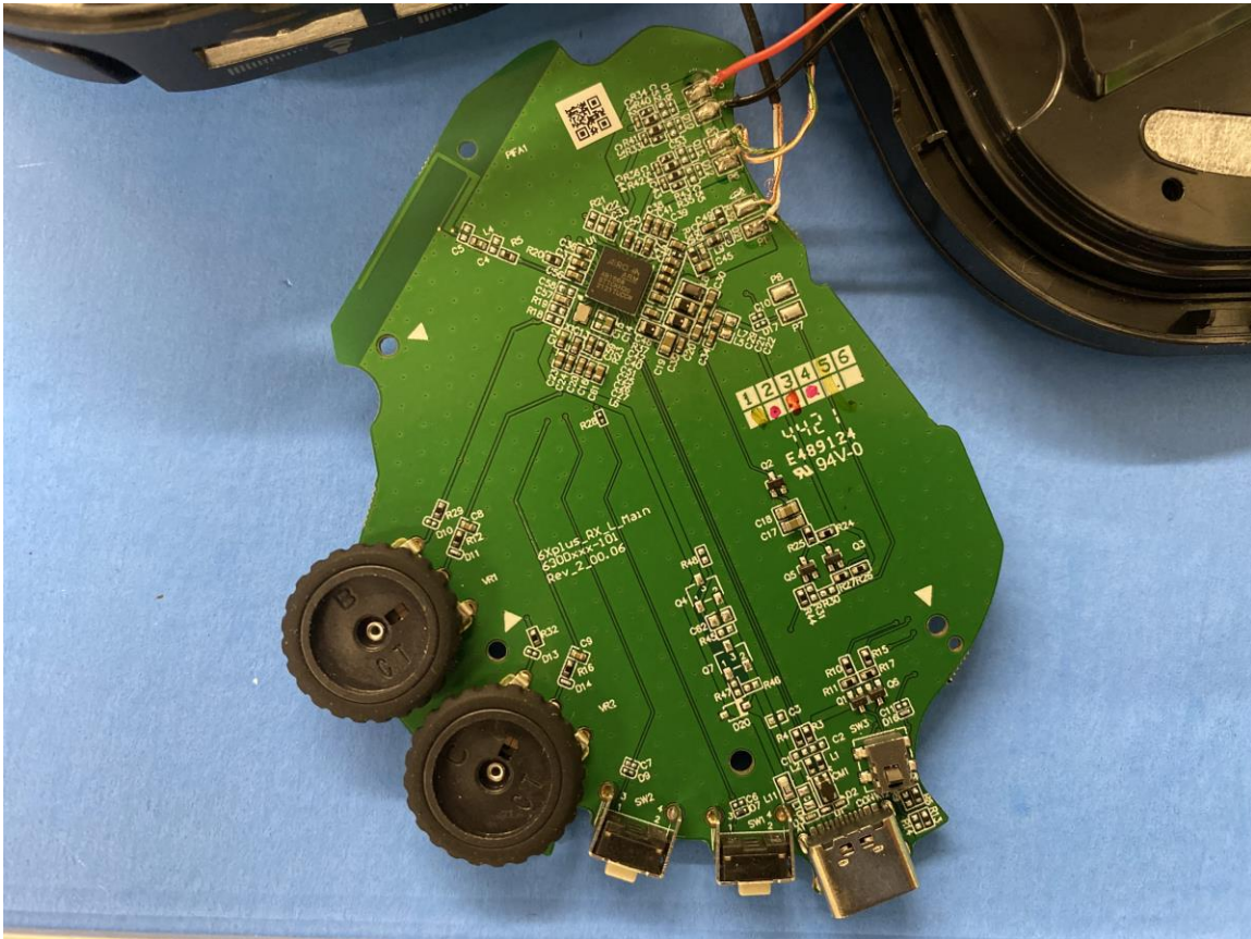
Figure 2: Internal Photo of Stealth600X-USB-RX Main PCB (Top)
