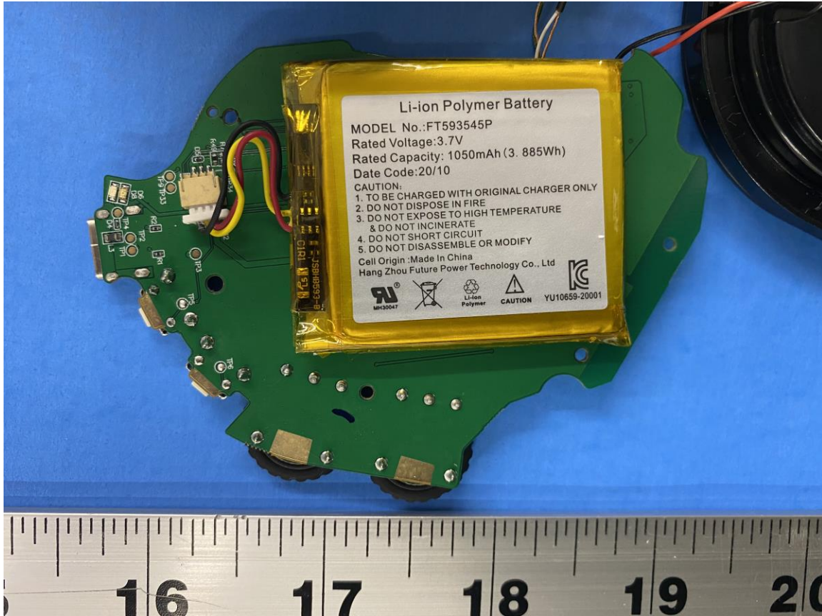
Figure 3: Internal Photo of Stealth600X-USB-RX Main PCB with Battery (Bottom)
