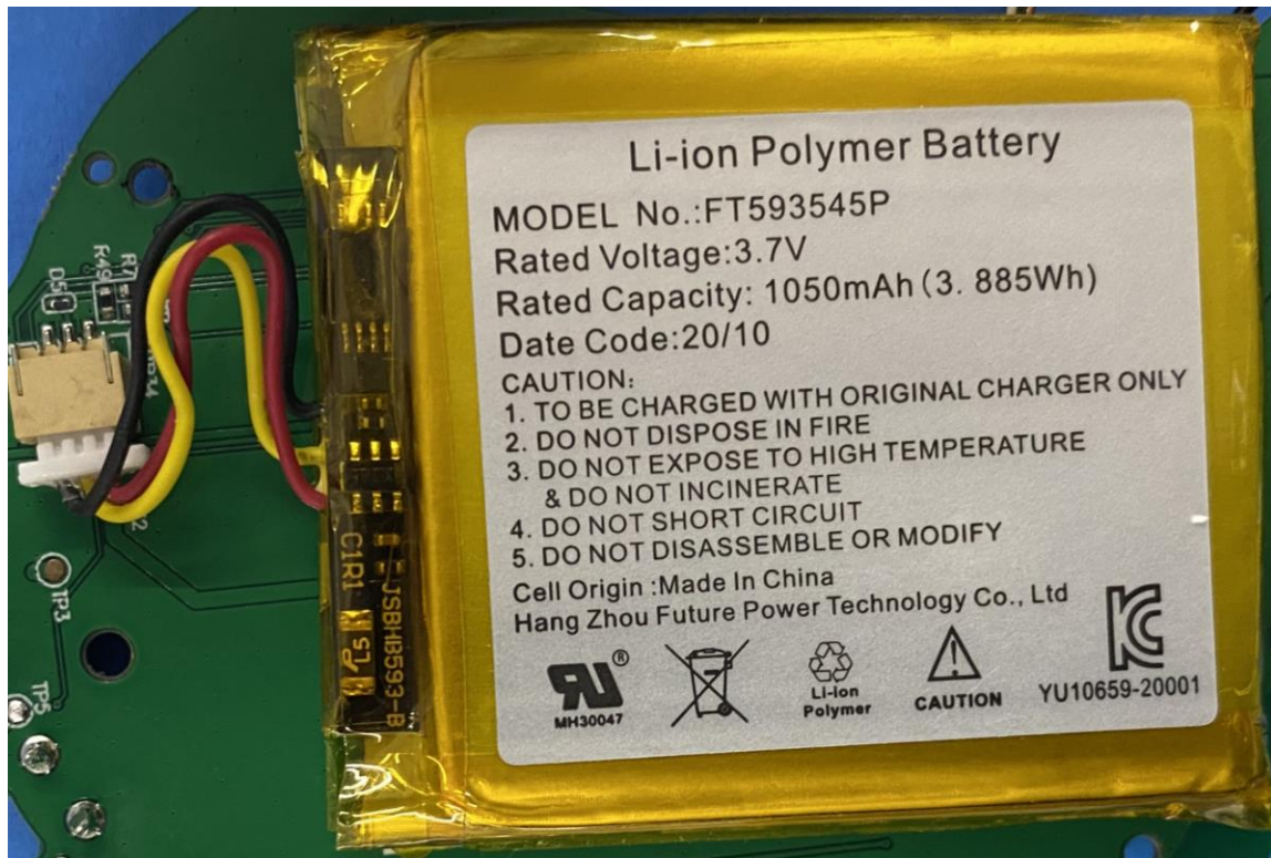
Figure 5: Internal Photo of Stealth600X-USB-RX (1050 mAh Battery, Top)
