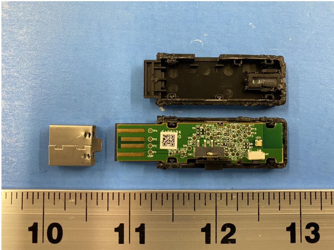
Figure 1: Internal Photo of Stealth 600X Gen 2 MAX TX with Plastic Cover Removed
