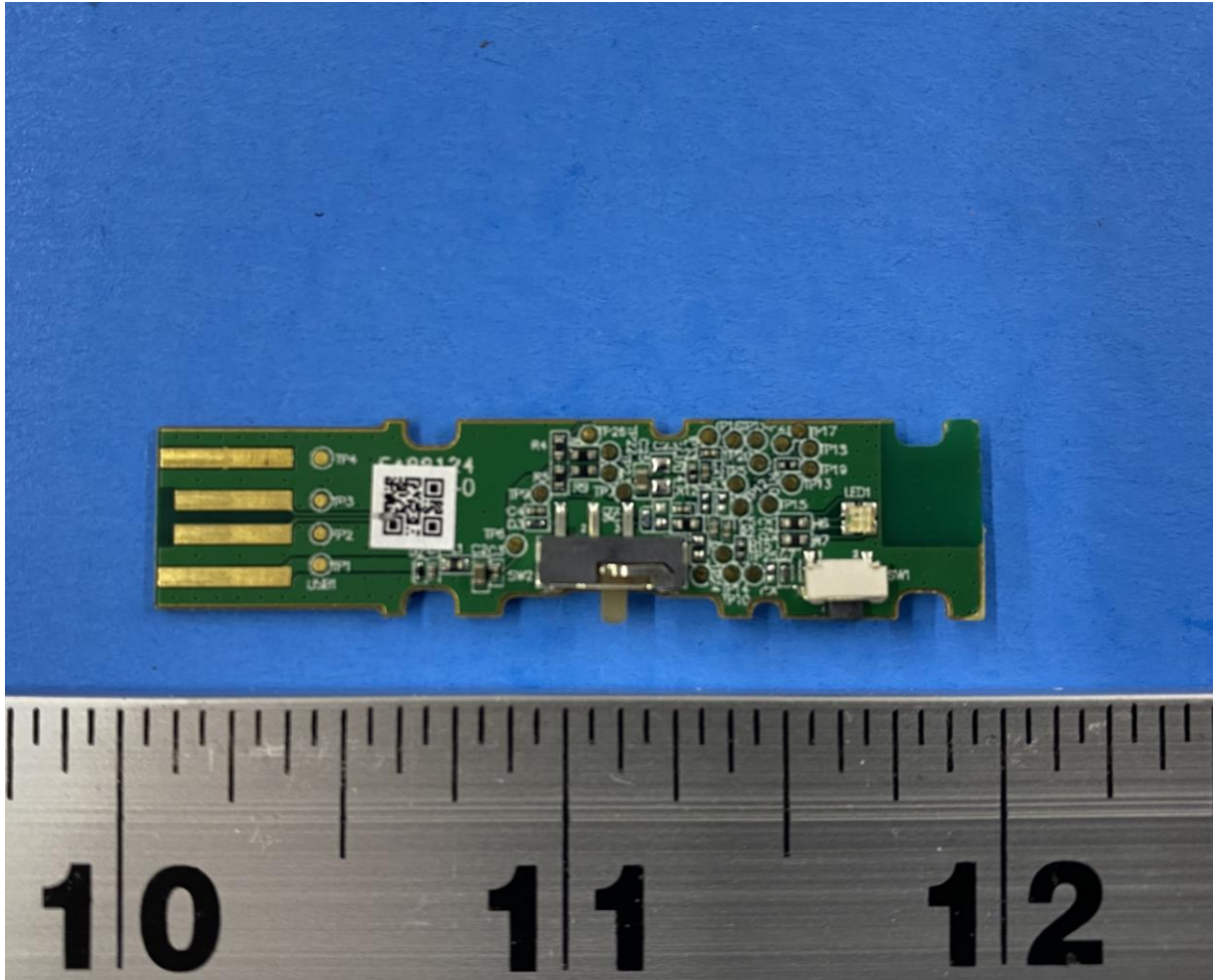
Figure 2: Internal Photo of Stealth 600X Gen 2 MAX TX – Top PCB
