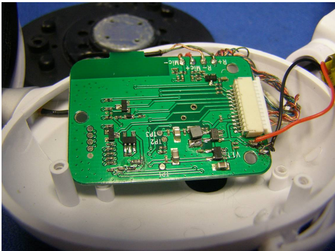
Picture 2 BT board
