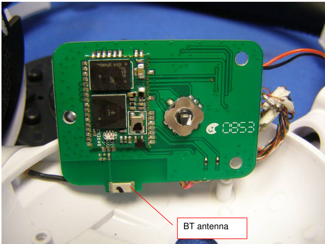
Picture 3 BT board
