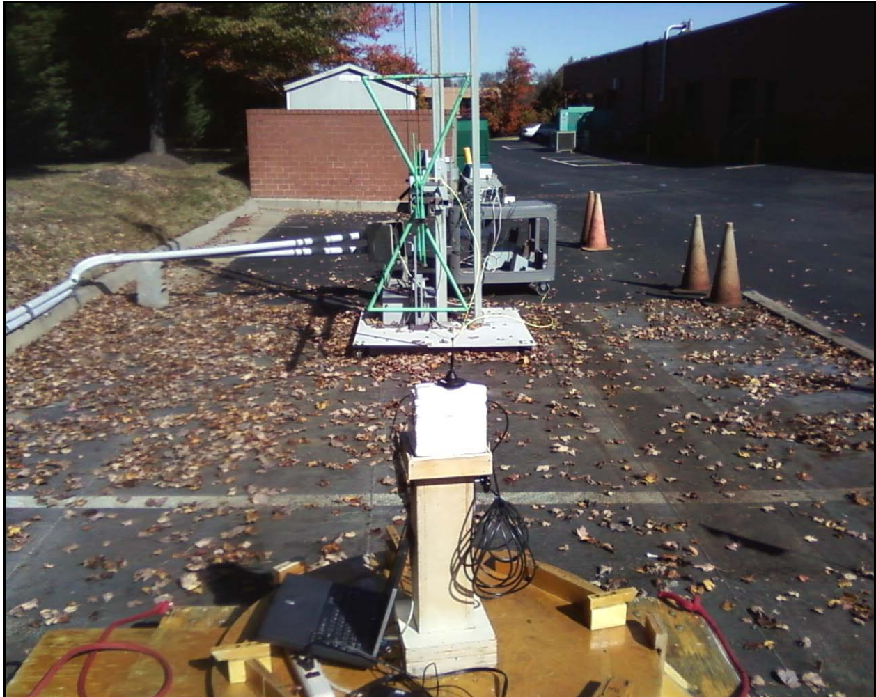
Photograph 2: Radiated Testing – Back View
