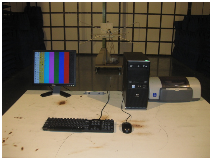
Photo of Radiated Emission Test
