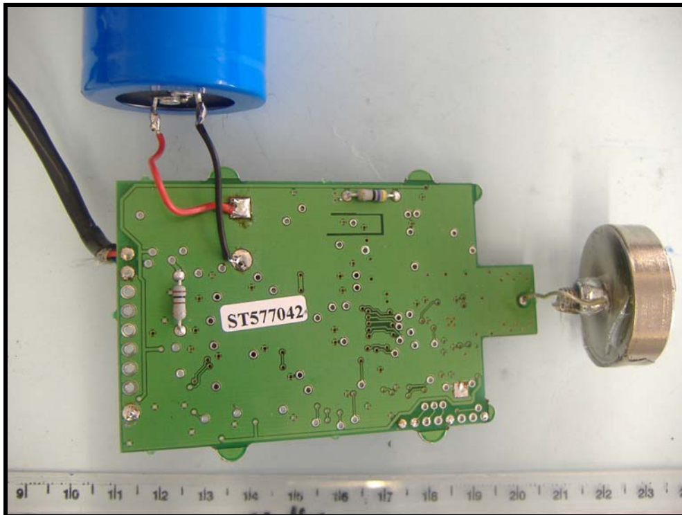
PCB TRACK SIDE
