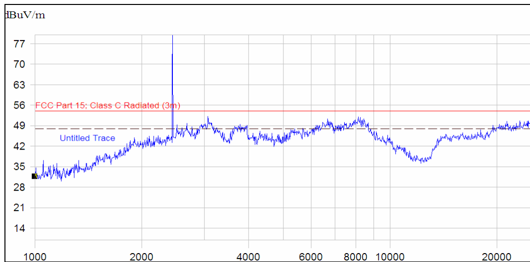
(Plot A.5: Antenna Vertical, 1GHz to 25GHz)
