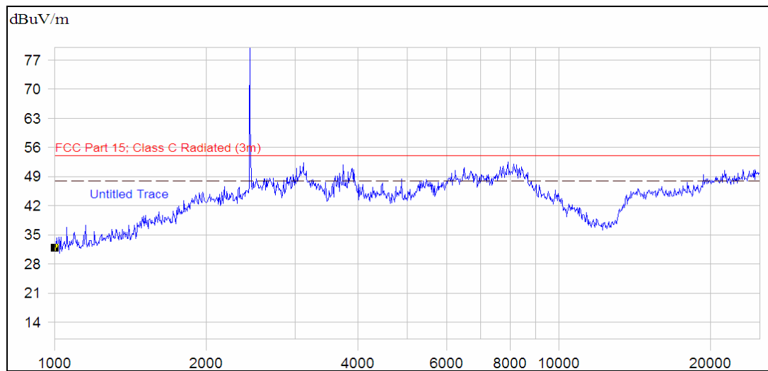
(Plot A.3: Antenna Horizontal, 1GHz to 25GHz)
