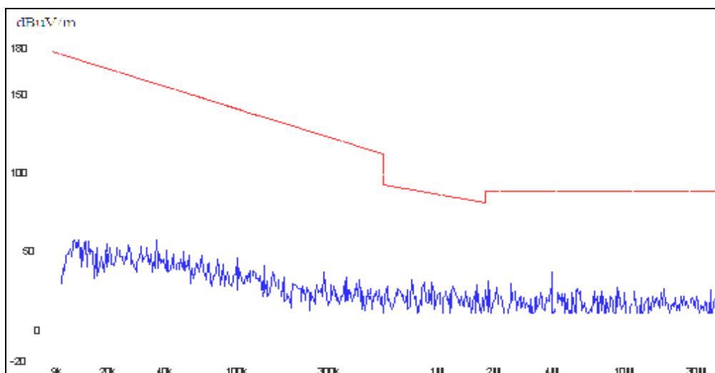
(Plot A.1: 9 kHz to 30MHz)
