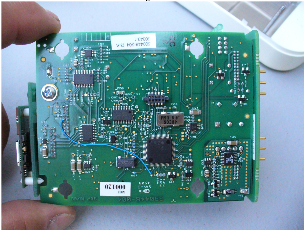
Charger board
