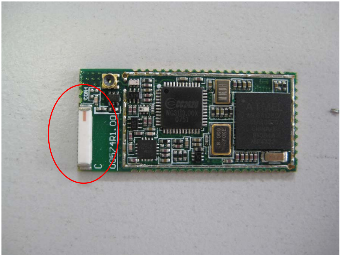
Photograph 1: - 2450AT45A100 (peak gain of 3 dBi)
