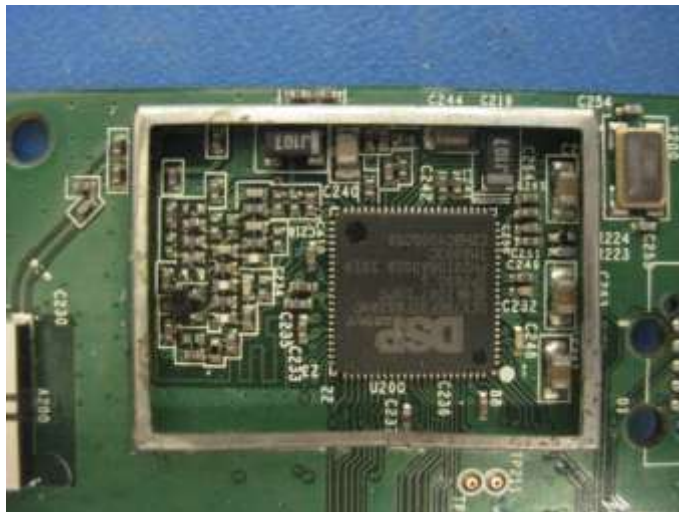
Photograph 6. RF Cover Zoom In
