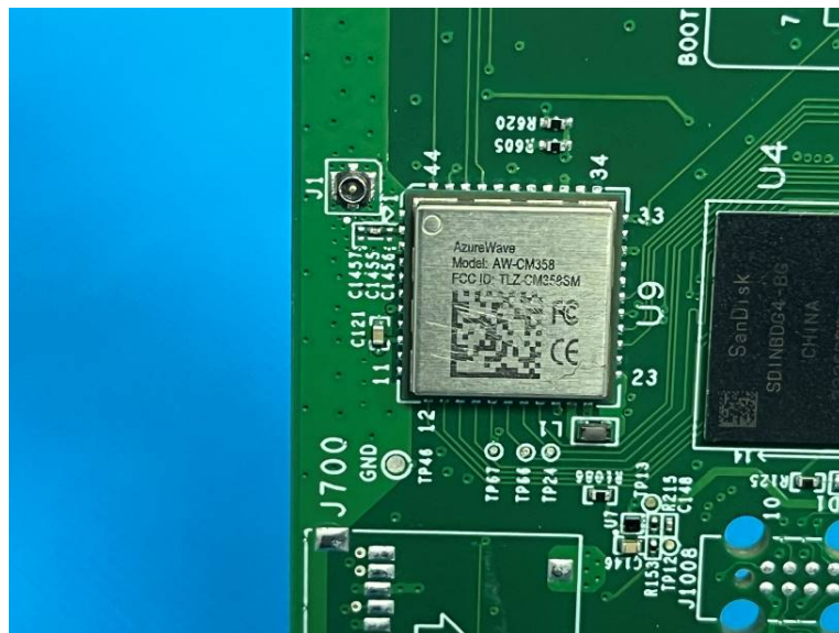
WiFi Module FCC ID: TLZ-CM358SM
