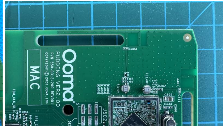
DECT ANT 1
