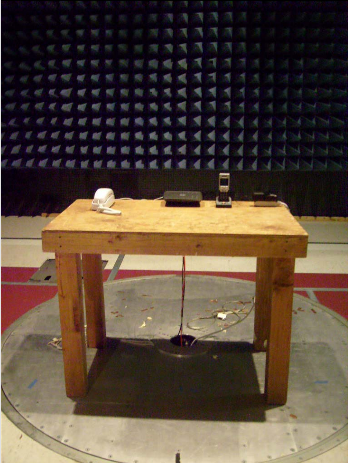
Photograph 2. Radiated Emissions
