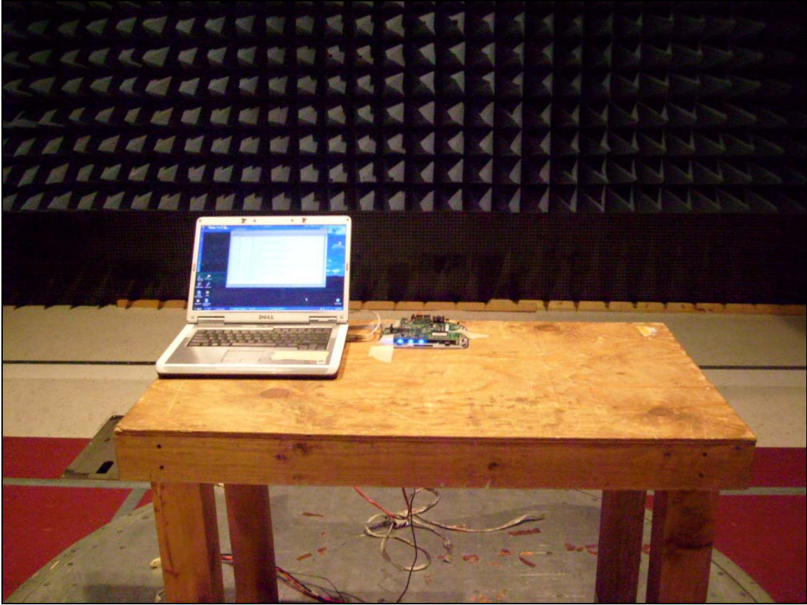
Photograph 3. Harmonics Test Setup
