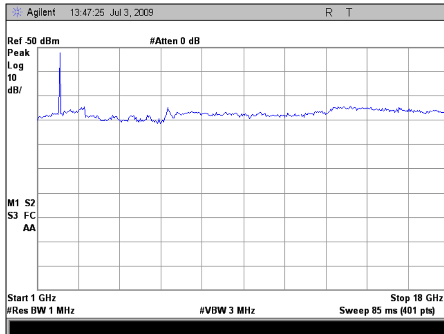
Plot 19. Radiated Harmonic Emissions, Low Channel
