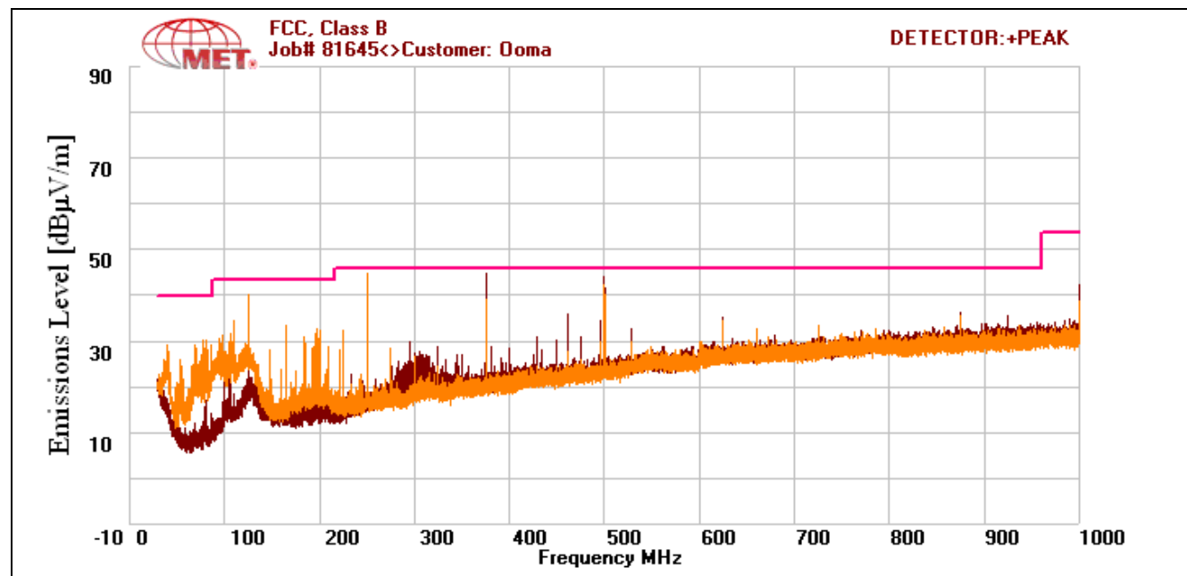
Plot 9. Radiated Emissions Pre-Scan, Ooma - ITE HK-R110-A05, 30 MHz – 1 GHz
