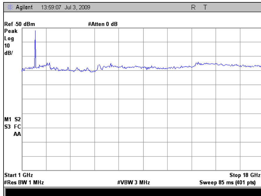
Plot 20. Radiated Harmonic Emissions, Mid Channel
