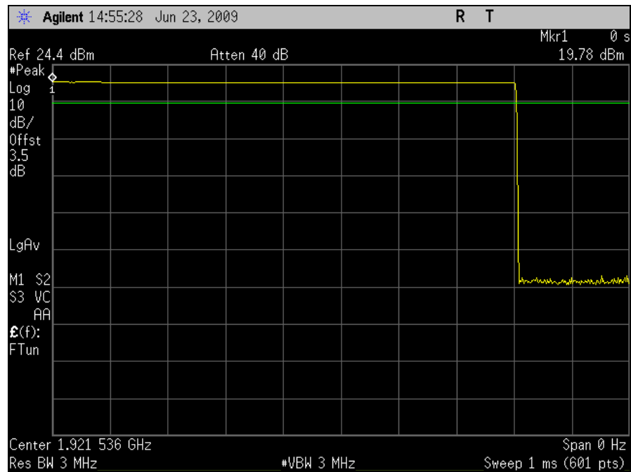
Plot 25. RF Output Power, Low Channel
