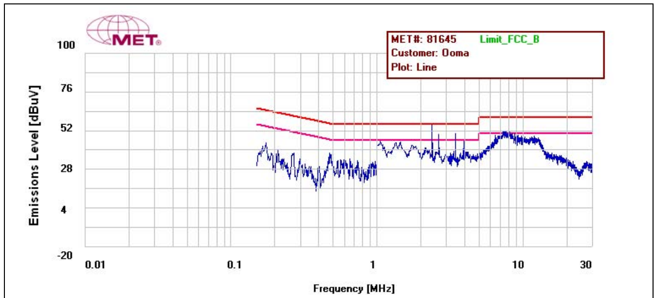
Plot 5. Conducted Emission, Phase Line Plot, Ooma - PSC11A-050
