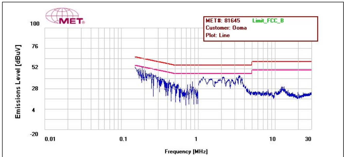
Plot 3. Conducted Emission, Phase Line Plot, Ooma - ITE HK-R110-A05
