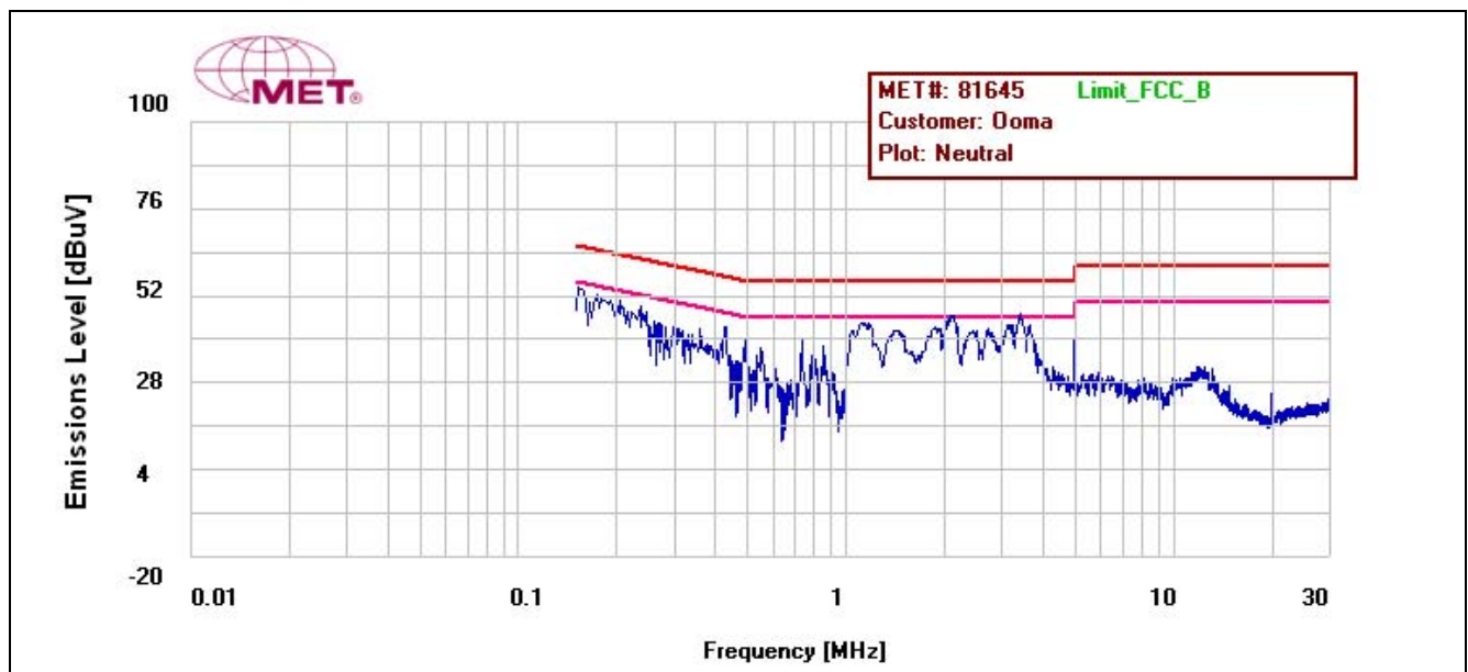
Plot 4. Conducted Emission, Neutral Line Plot, Ooma - ITE HK-R110-A05
