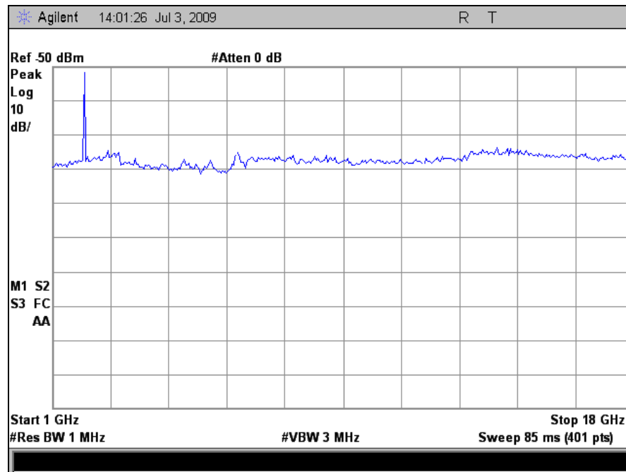
Plot 21. Radiated Harmonic Emissions, High Channel
