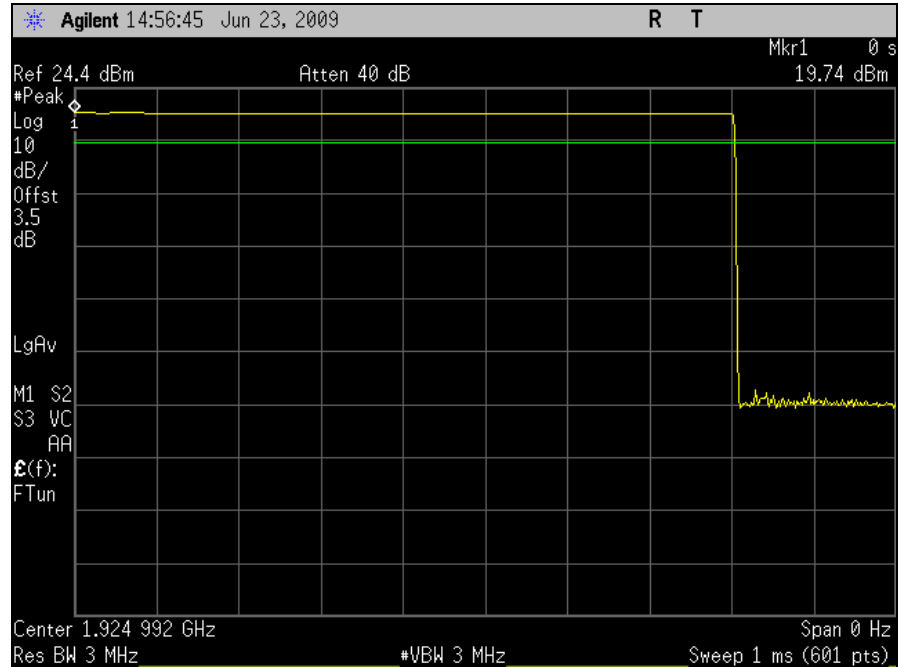
Plot 26. RF Output Power, Mid Channel
