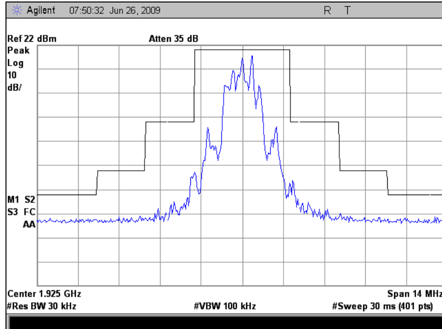
Plot 32. Conducted Spurious Emission, In-Band, Mid Channel
