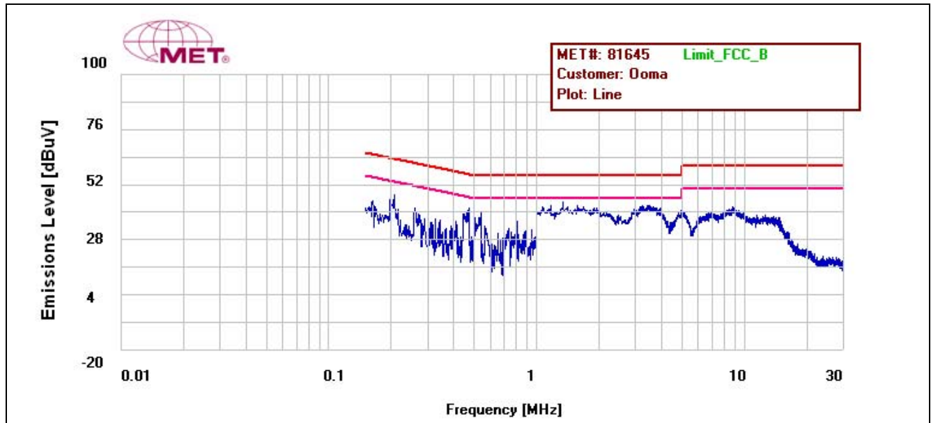
Plot 1. Conducted Emission, Phase Line Plot, Fairway - WRG10F-050A
