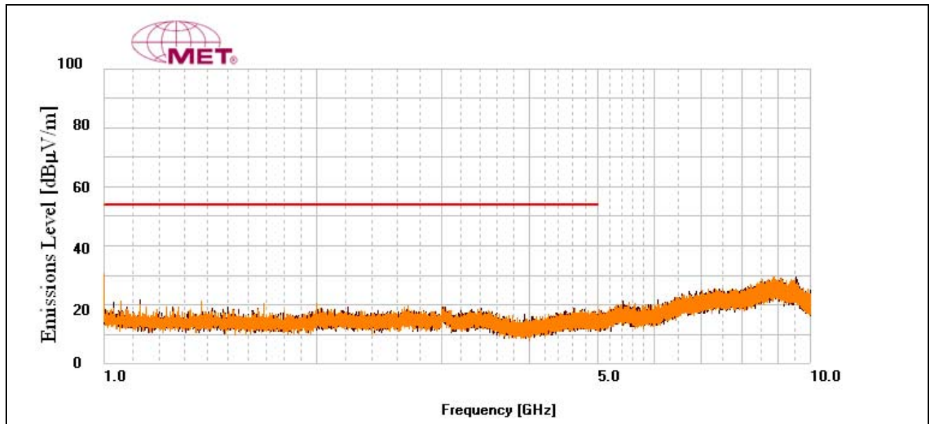
Plot 12. Radiated Emissions Pre-Scan, Ooma PSC11A-050, 1 GHz – 10 GHz
