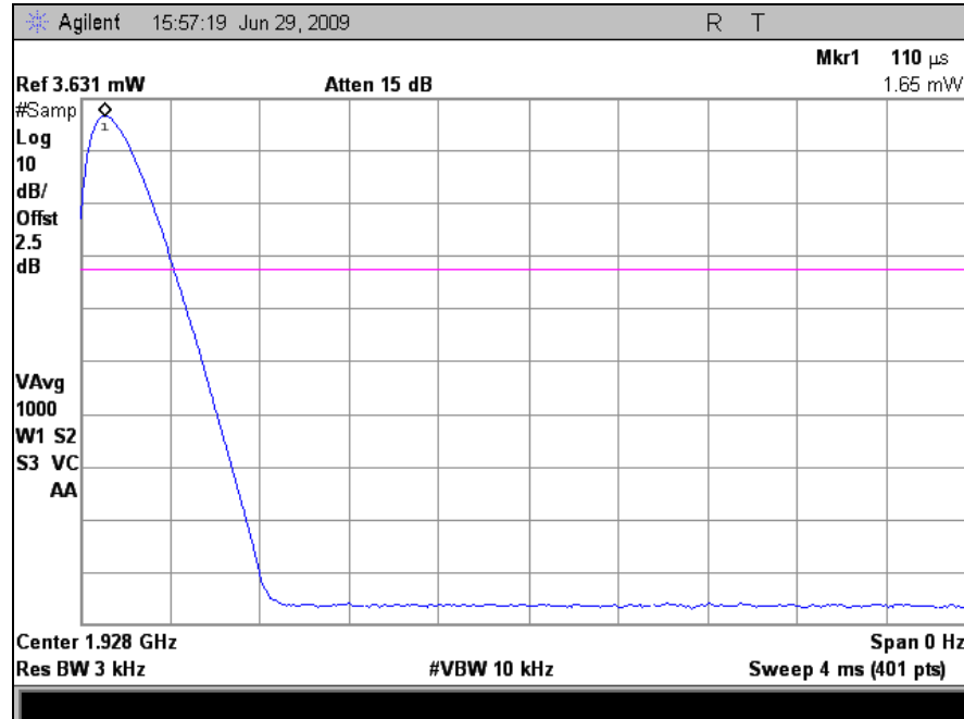
Plot 30. Peak Power Spectral Density, High Channel
