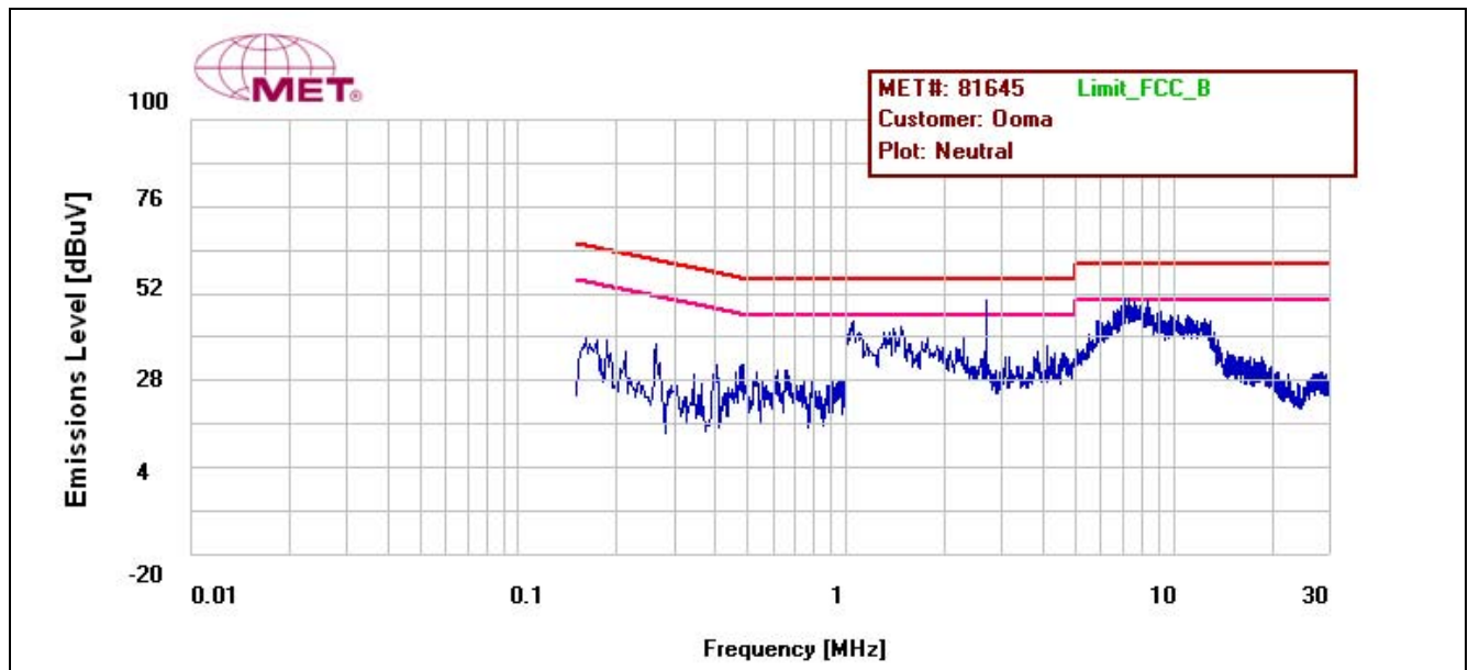
Plot 6. Conducted Emission, Neutral Line Plot, Ooma - PSC11A-050
