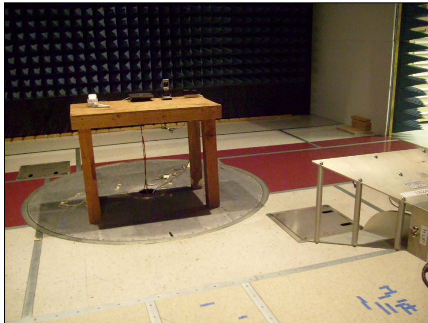
Photograph 5. Radiated Emission, Test Setup, Horn
