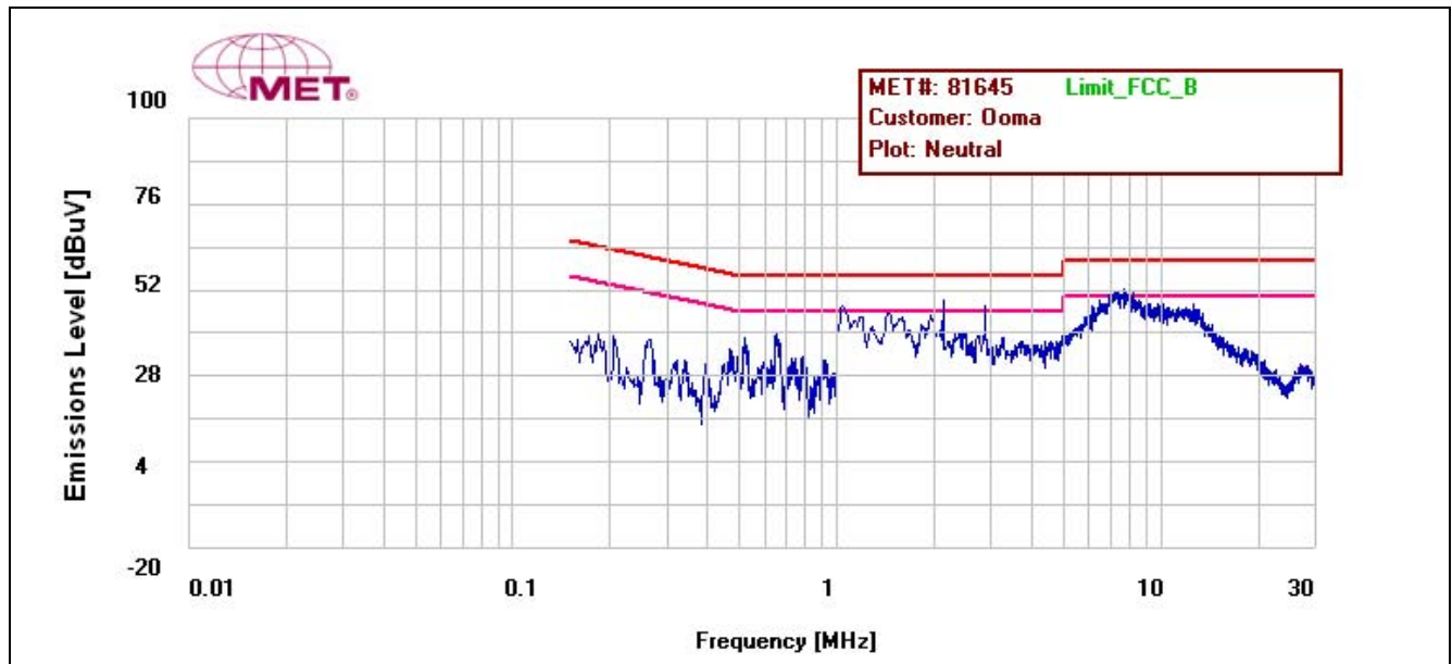
Plot 18. Conducted Emissions, §15.207, Neutral Line, Ooma - PSC11A-050
