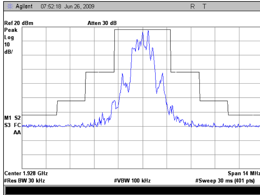
Plot 33. Conducted Spurious Emission, In-Band, High Channel
