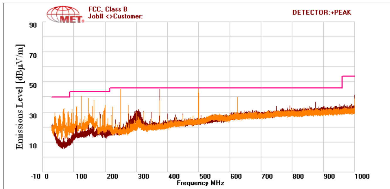
Plot 11. Radiated Emissions Pre-Scan, Ooma PSC11A-050, 30 MHz – 1 GHz
