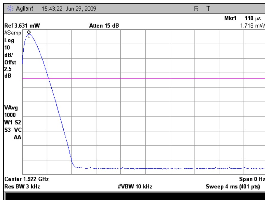
Plot 28. Peak Power Spectral Density, Low Channel
