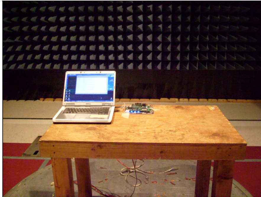
Photograph 7. Radiated Harmonic Emissions, Test Setup
