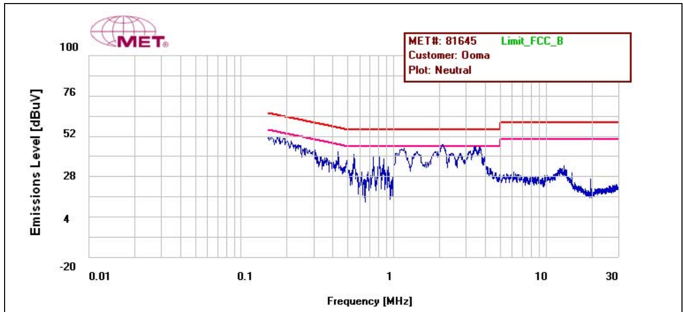
Plot 16. Conducted Emissions, §15.207, Neutral Line, Ooma - ITE HK-R110-A05
