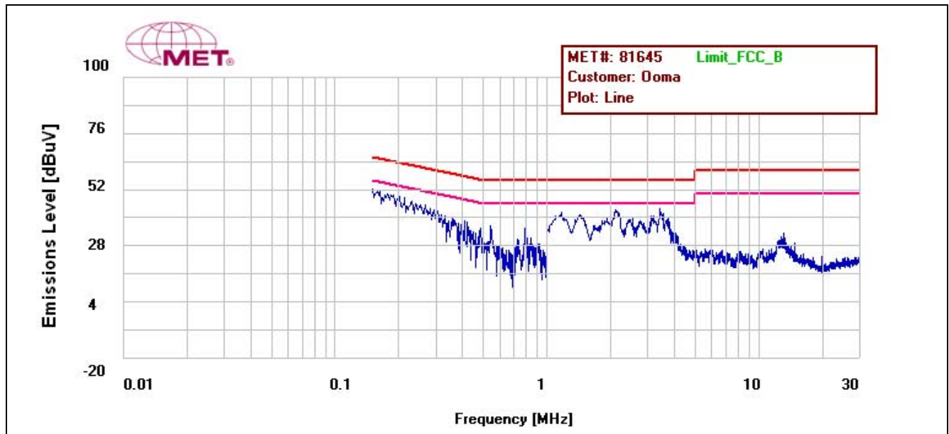
Plot 15. Conducted Emissions, §15.207, Phase Line, Ooma - ITE HK-R110-A05
