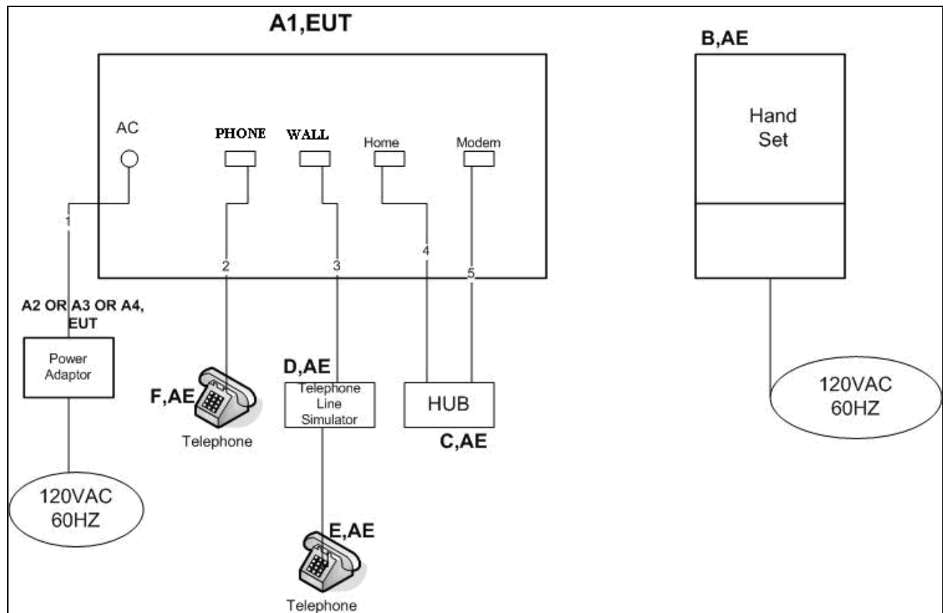
Figure 1. Block Diagram of Test Configuration, FCC Part 15B
