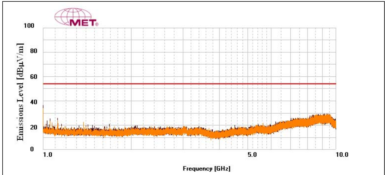
Plot 8. Radiated Emissions Pre-Scan, Fairway-WRG10F-050A, 1 GHz – 10 GHz
