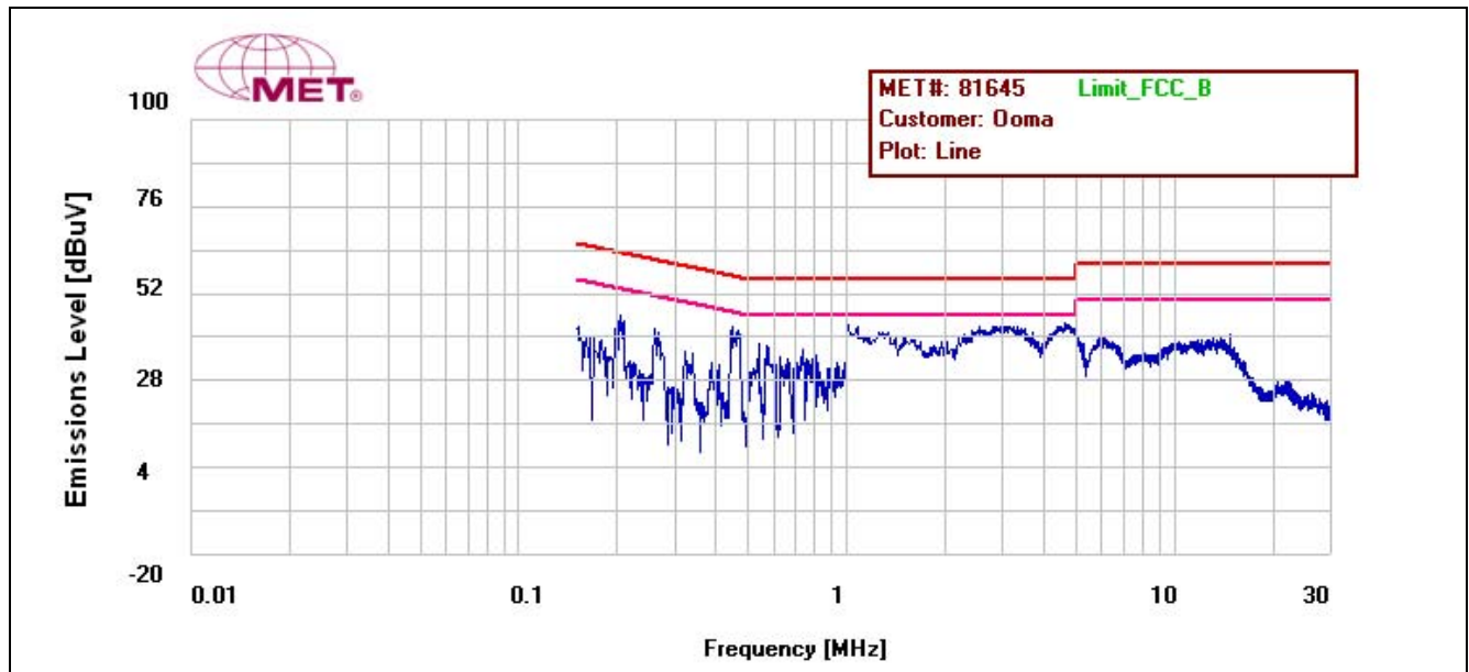
Plot 13. Conducted Emissions, §15.207, Phase Line, Fairway - WRG10F-050A
