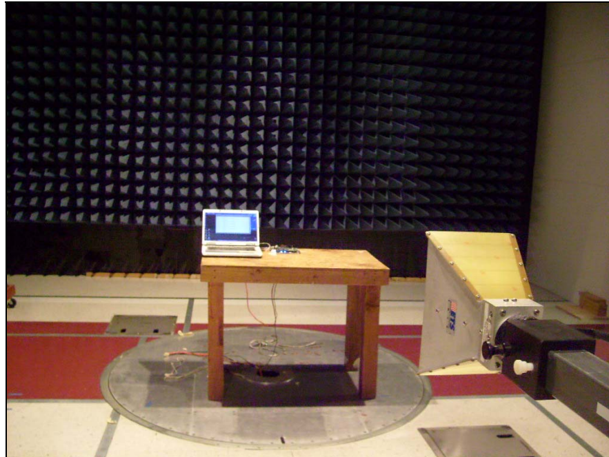
Photograph 8. Radiated Harmonic Emissions, Horn
