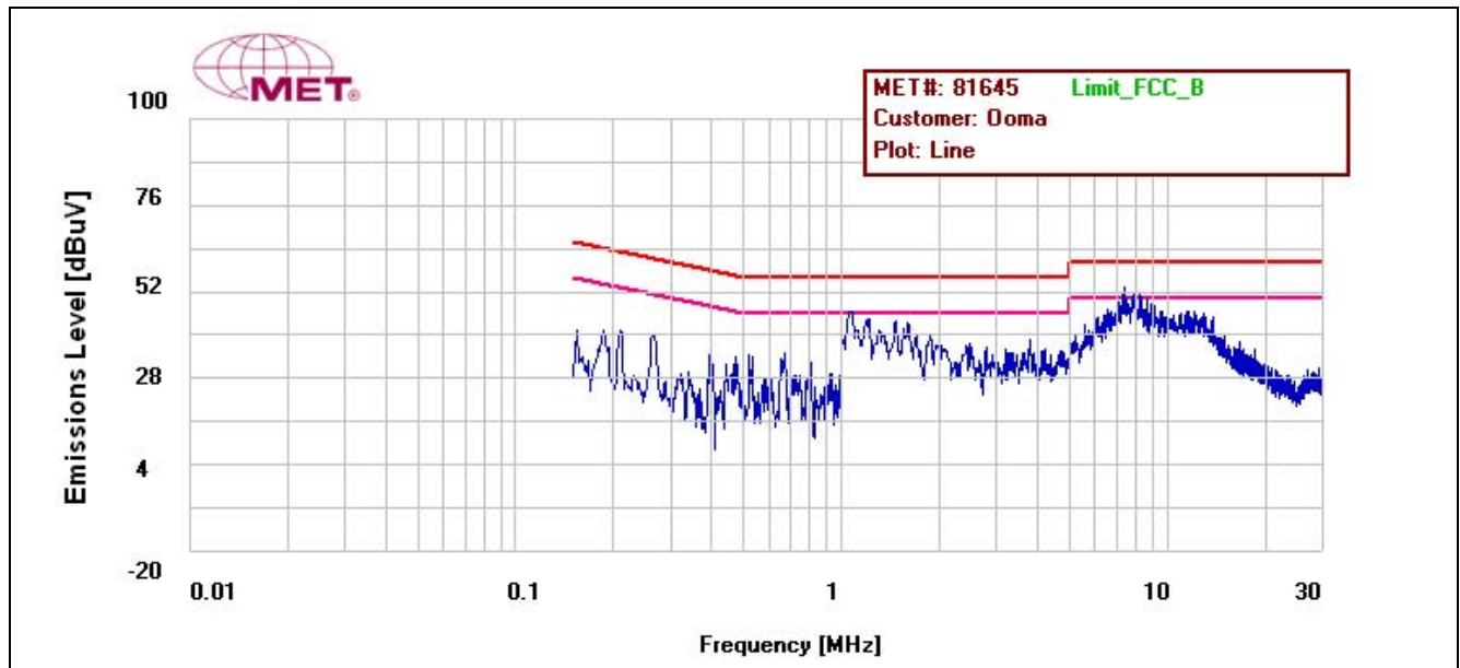
Plot 17. Conducted Emissions, §15.207, Phase Line, Ooma - PSC11A-050
