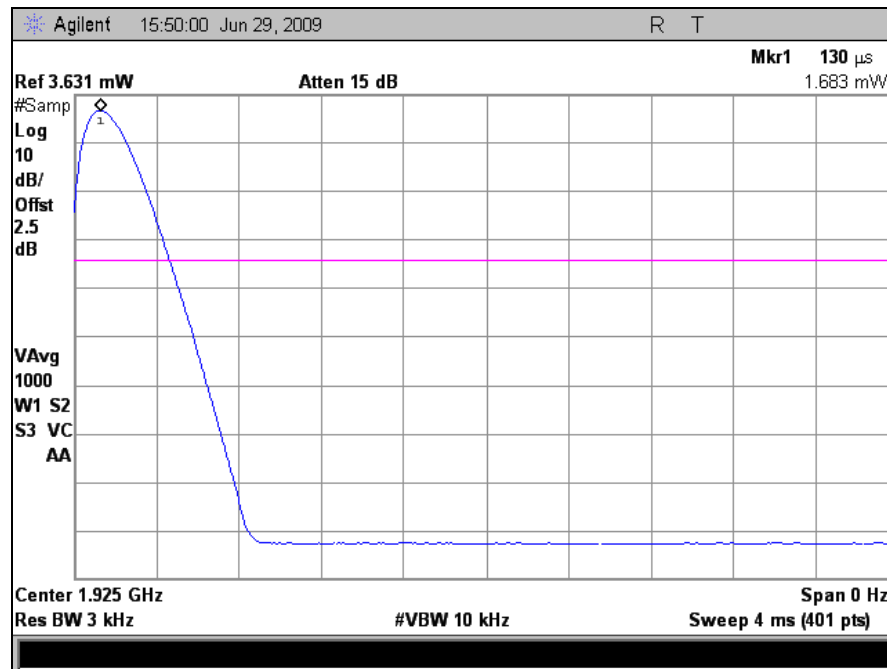
Plot 29. Peak Power Spectral Density, Mid Channel
