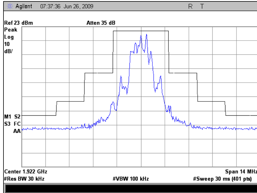
Plot 31. Conducted Spurious Emission, In-Band, Low Channel
