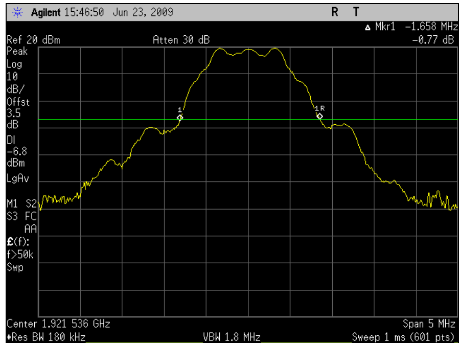
Plot 22. Occupied Bandwidth, Low Channel
