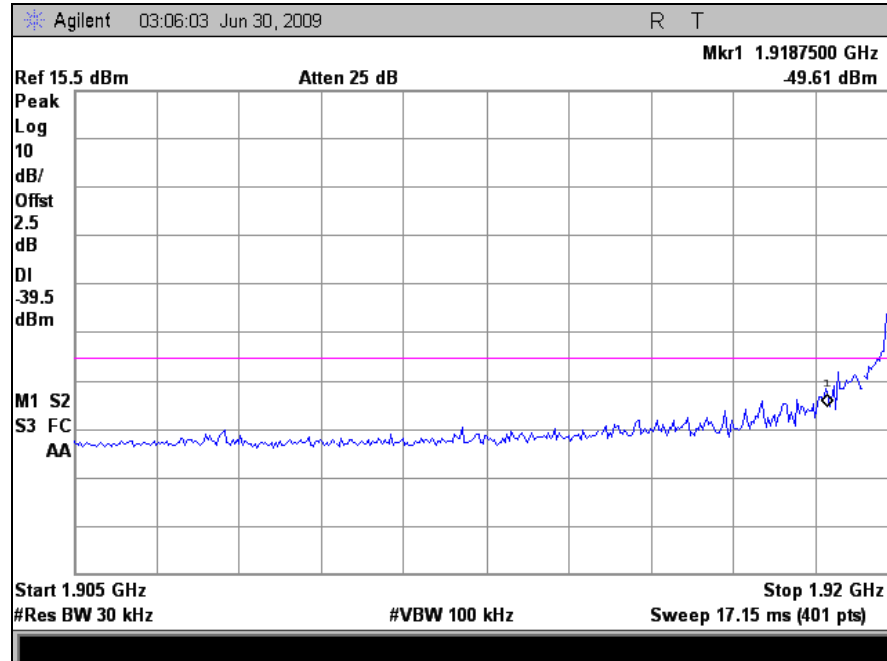
Plot 34. Conducted Spurious Emission, Out-of-Band, Low Channel
