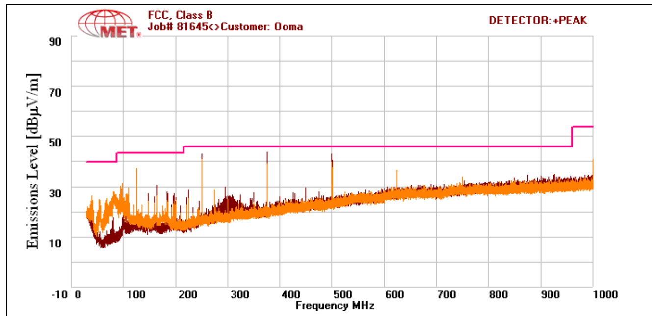
Plot 7. Radiated Emissions Pre-Scan, Fairway-WRG10F-050A, 30 MHz – 1 GHz
