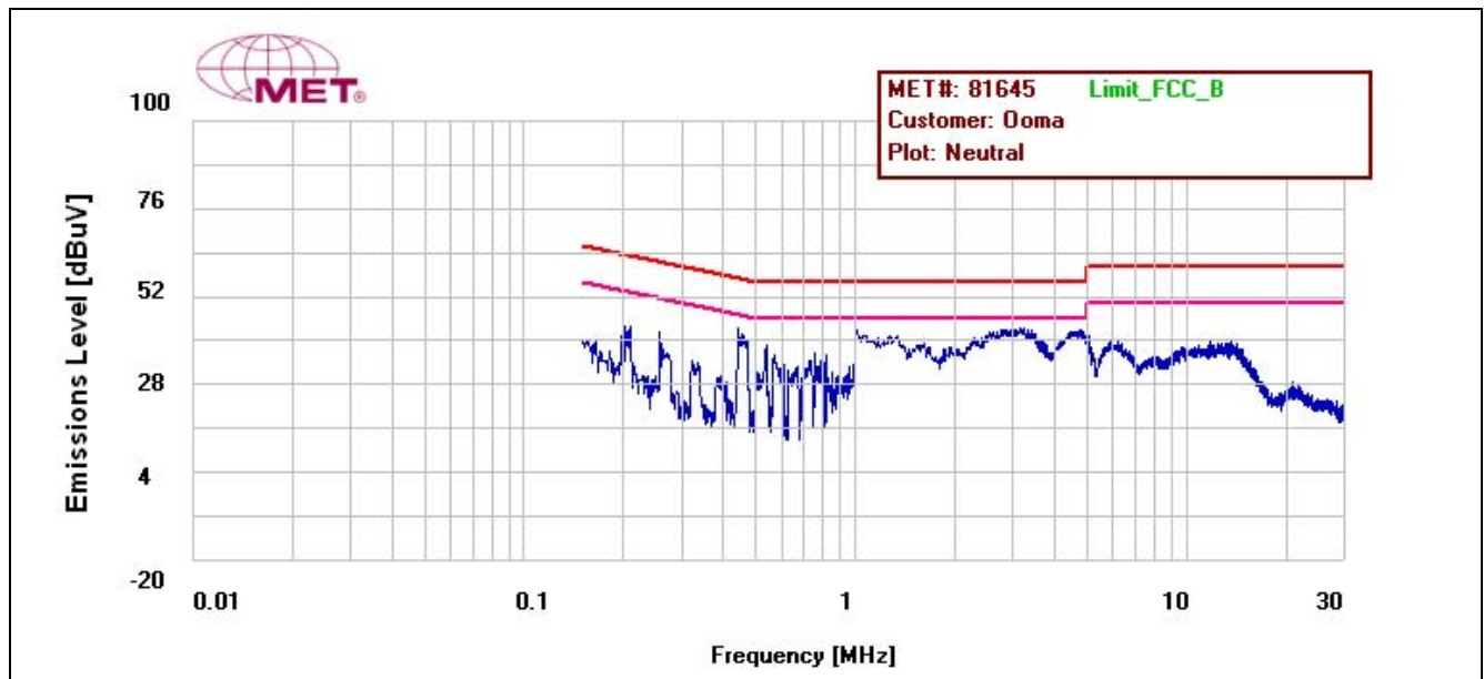
Plot 2. Conducted Emission, Neutral Line Plot, Fairway - WRG10F-050A
