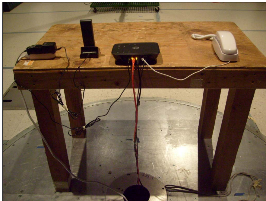
Photograph 3. Radiated Emission, Test Setup, Back View
