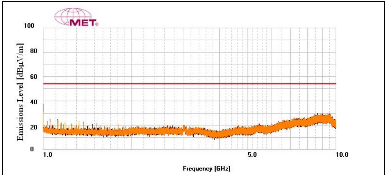
Plot 10. Radiated Emissions Pre-Scan, Ooma - ITE HK-R110-A05, 1 GHz – 10 GHz
