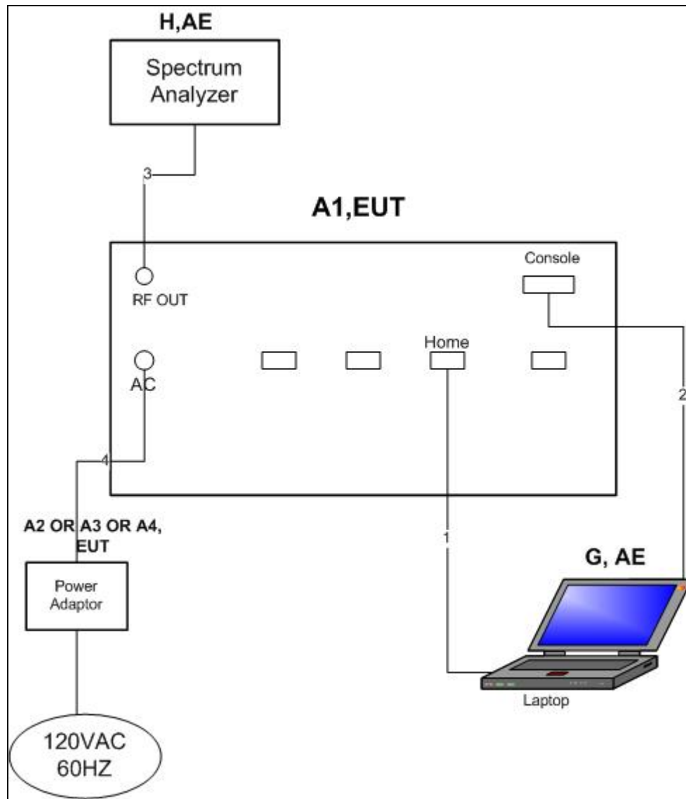
Figure 2. Block Diagram of Test Configuration, FCC Part 15D
