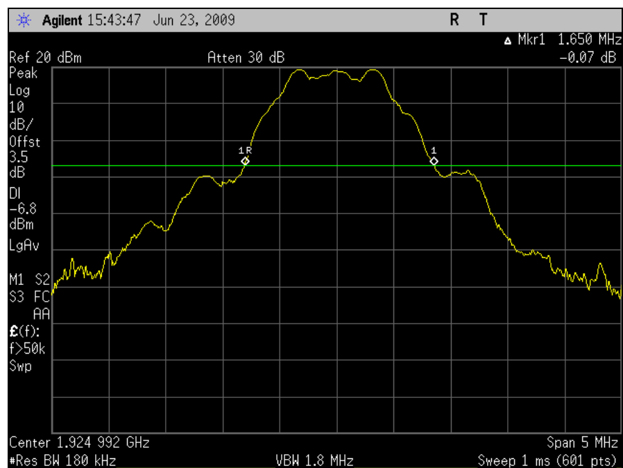
Plot 23. Occupied Bandwidth, Mid Channel
