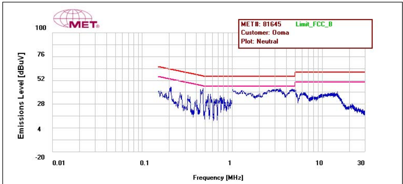
Plot 14. Conducted Emissions, §15.207, Neutral Line, Fairway - WRG10F-050A
