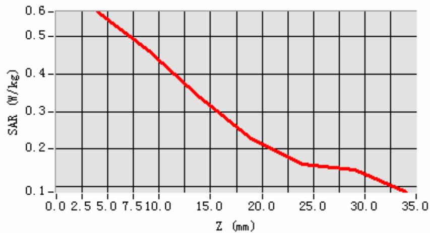
SAR, Z Axis Scan (X = 3, Y = -24)
