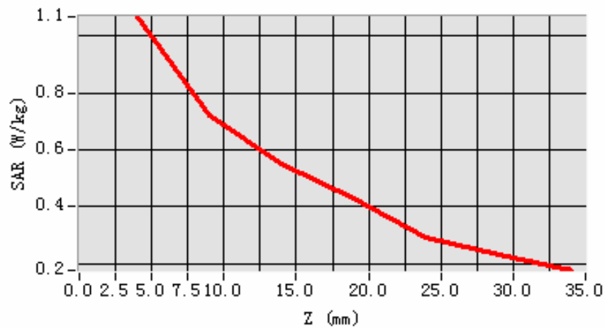
SAR, Z Axis Scan (X = -48, Y = -37)
