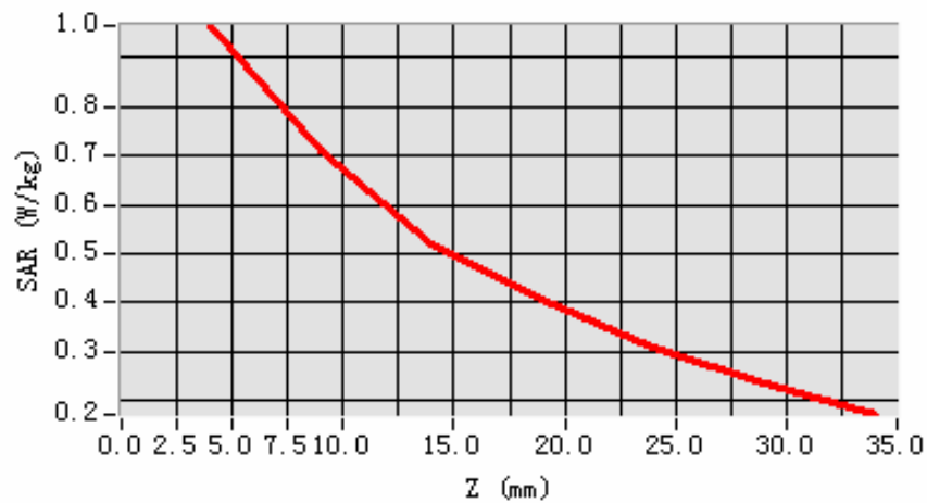
SAR, Z Axis Scan (X = -53, Y = -20)
