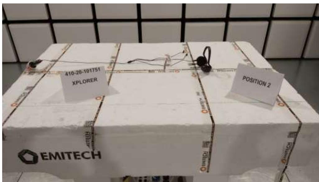
TEST SETUP PHOTO(S) - CHARGING + TX MODE – POSITION 2
