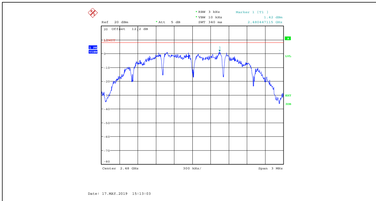
Plot 5.5.4.4. Power Spectral Density, O-QPSK Modulation, Power Setting 12, Channel 26, 2480 MHz
