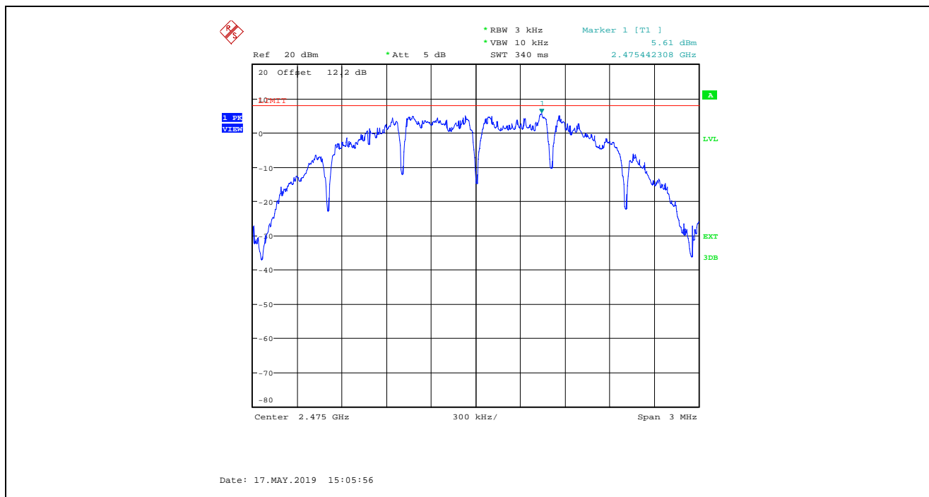
Plot 5.5.4.3. Power Spectral Density, O-QPSK Modulation, Power Setting 15, Channel 25, 2475 MHz
