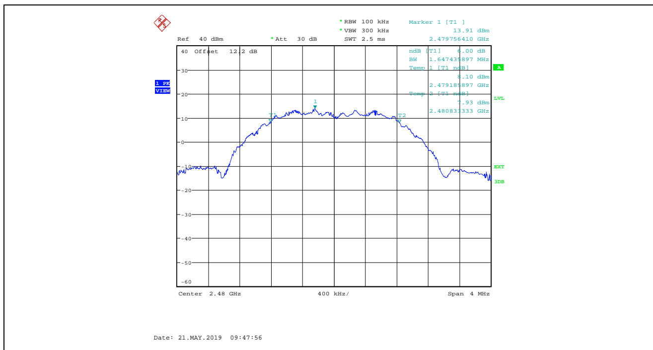
Plot 5.2.4.4. 6 dB Bandwidth, O-QPSK Modulation, Power Setting at 12, Channel 26, 2480 MHz
