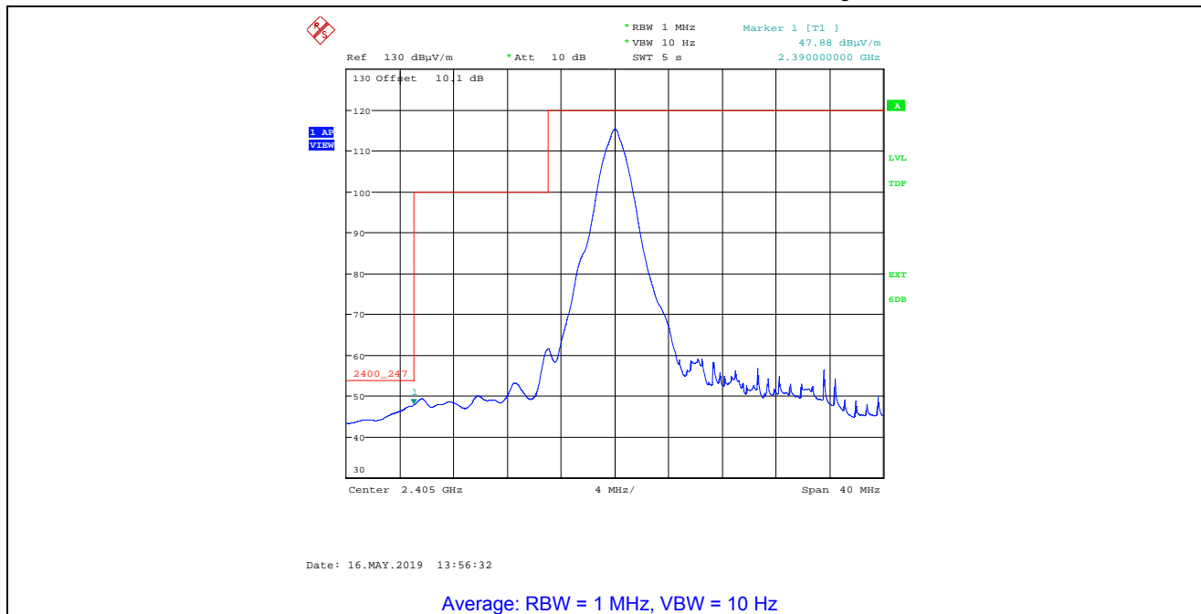
Plot 5.4.4.2.2. Band-Edge Radiated Emissions, Lower Band- edge Rx Antenna in Vertical Polarization, O-QPSK Modulation, Power Setting 15, Ch 11, 2405 MHz
