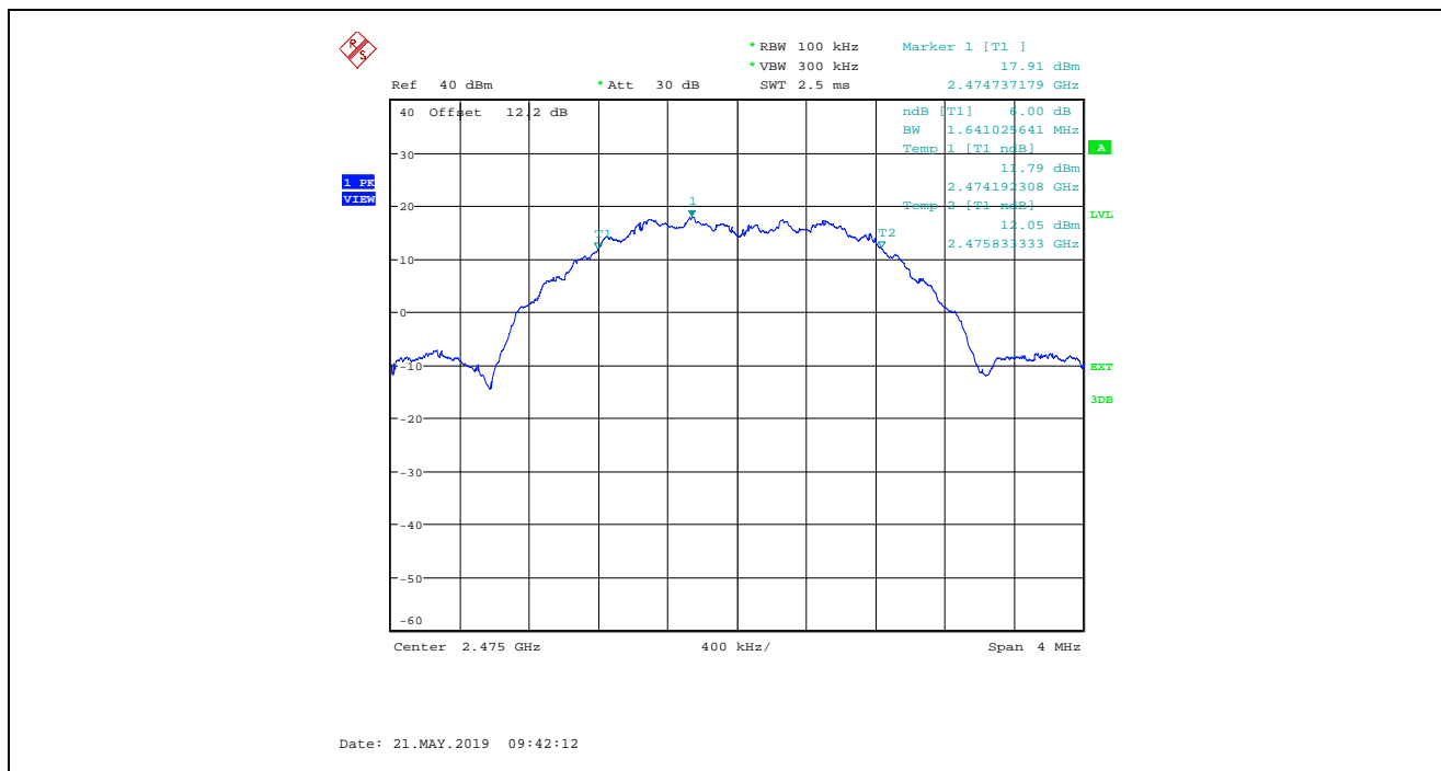
Plot 5.2.4.3. 6 dB Bandwidth, O-QPSK Modulation, Power Setting at 15, Channel 25, 2475 MHz
