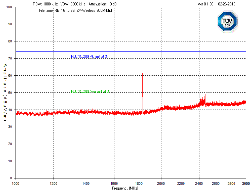
Graph 45 Test Results – Tx Spurious emission 1GHz – 3GHz: Mid Channel ZX Wireless Thermostat (900MHz) – Vertical Polarization
