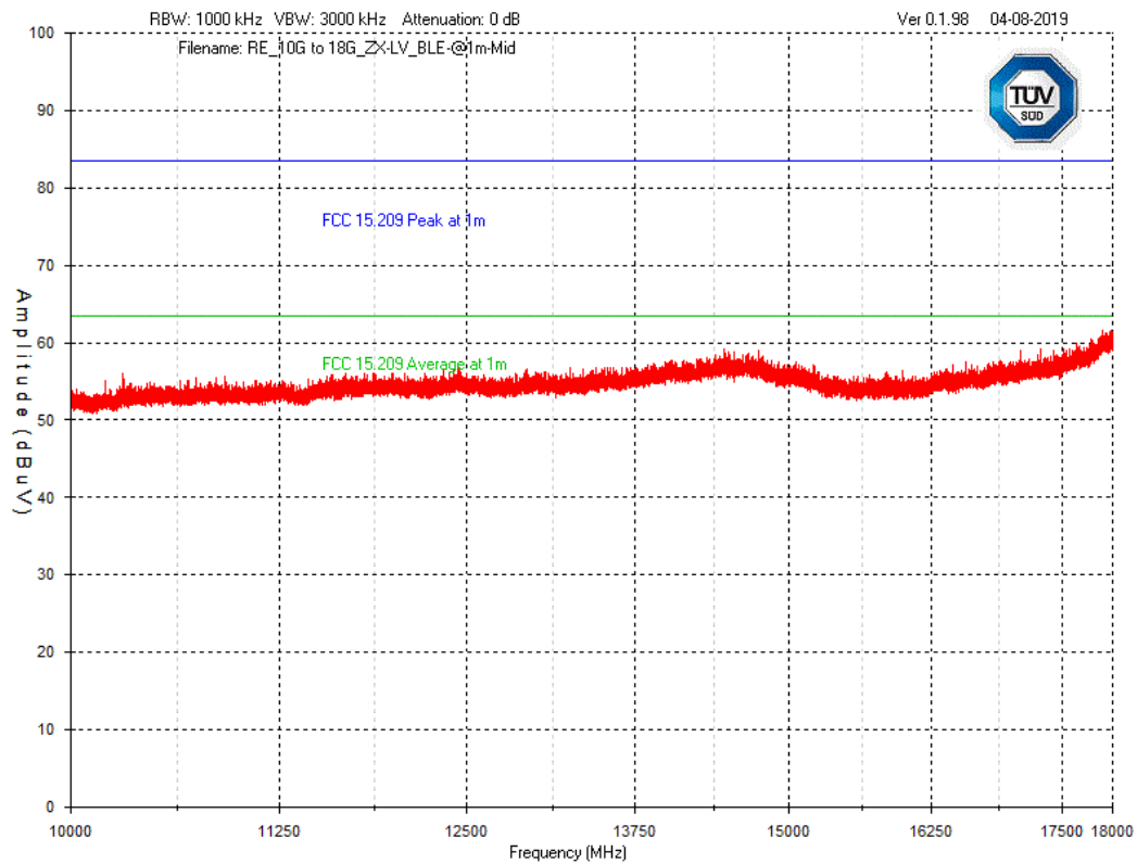
Graph 52 Test Results – Tx Spurious emission 10GHz – 18GHz: Mid Channel ZX Low Voltage Thermostat (2.4GHz) – Horizontal Polarization
