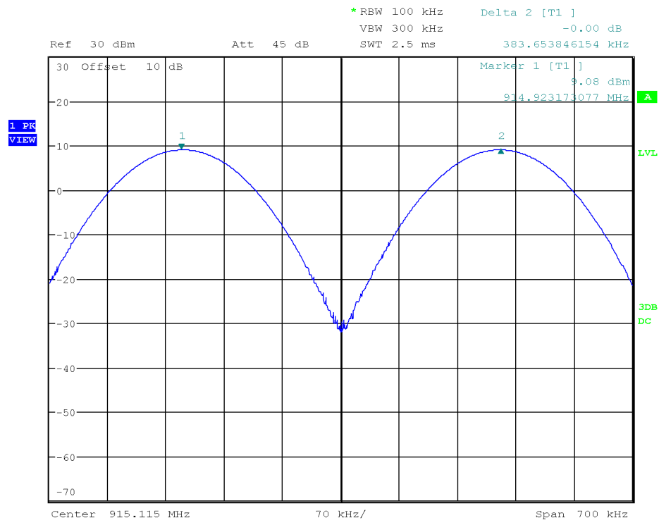
Graph 13: Channel Separation – ZX
