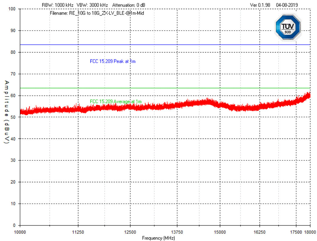
Graph 53 Test Results – Tx Spurious emission 10GHz – 18GHz: Mid Channel ZX Low Voltage Thermostat (2.4GHz) – Vertical Polarization
