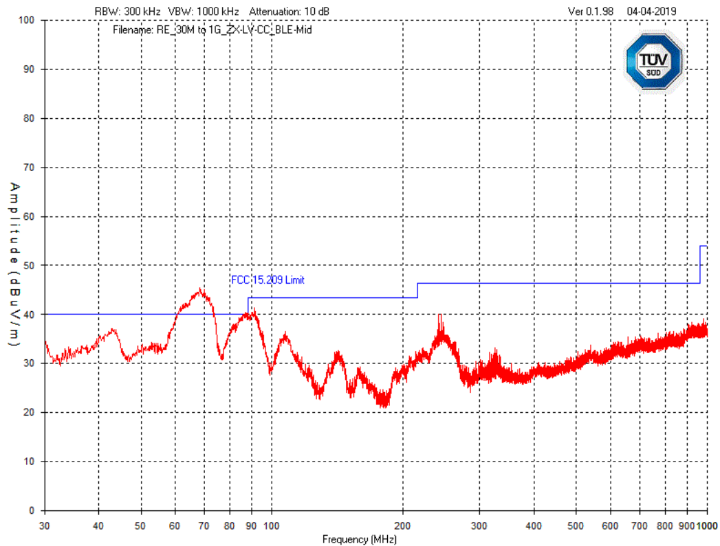
Graph 42 Test Results – Tx Spurious emission 30MHz – 1GHz: Mid Channel ZX Low Voltage Thermostat(2.4GHz) – Vertical Polarization
