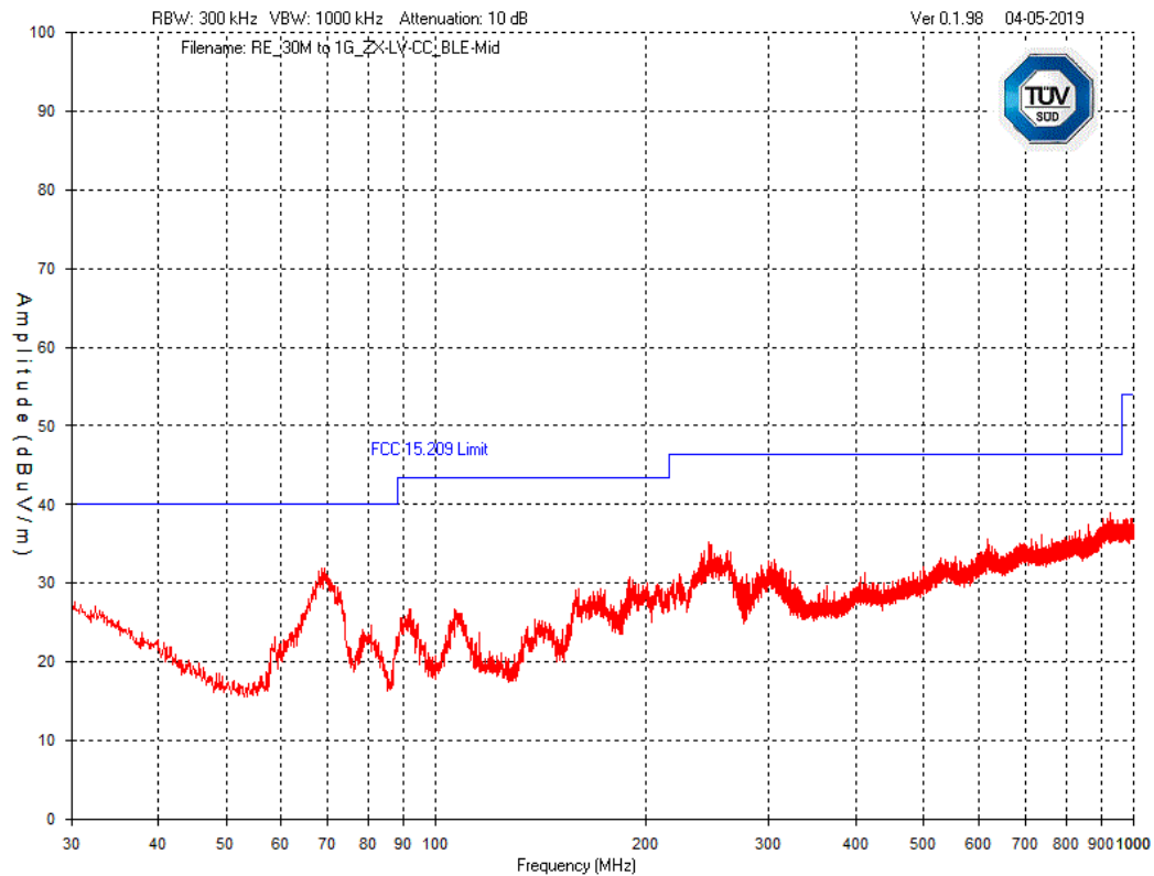
Graph 43 Test Results – Tx Spurious emission 30MHz – 1GHz: Mid Channel ZX Low Voltage Thermostat(2.4GHz) – Horizontal Polarization
