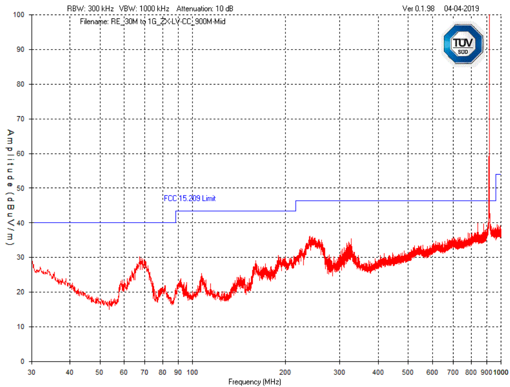
Graph 40 Test Results – Tx Spurious emission 30MHz – 1GHz: Mid Channel ZX Low Voltage Thermostat (900MHz) – Horizontal Polarization
