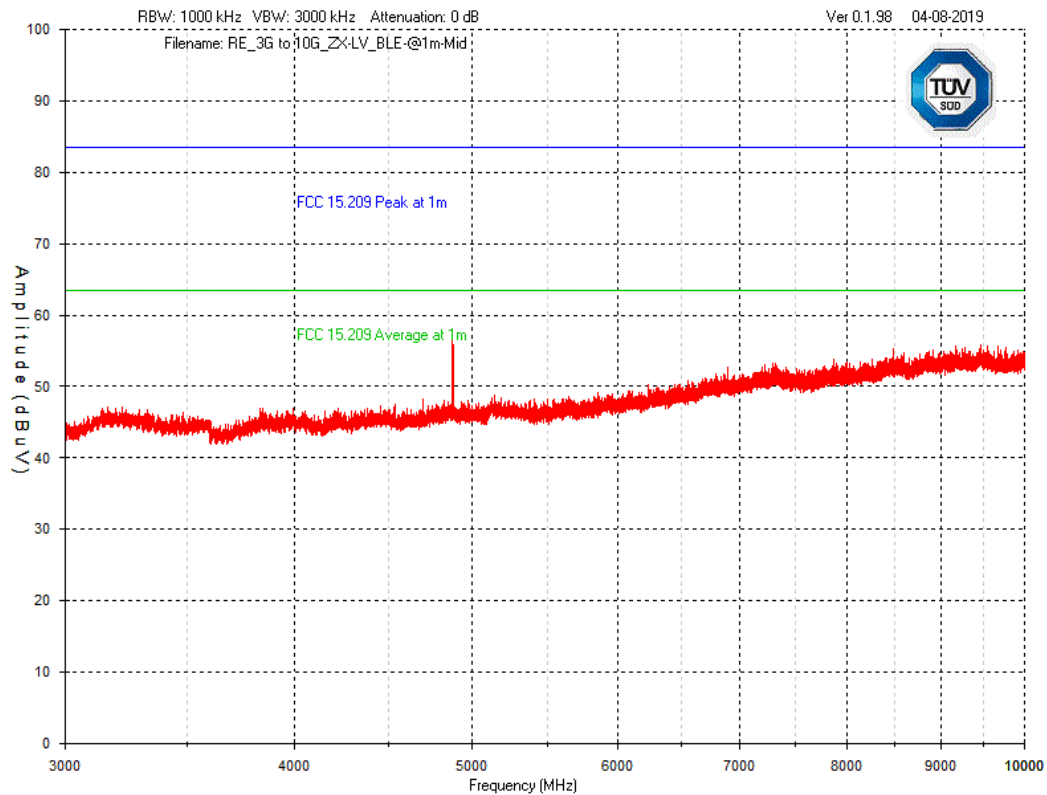
Graph 50 Test Results – Tx Spurious emission 3GHz – 10GHz: Mid Channel ZX Low Voltage Thermostat (2.4GHz) – Horizontal Polarization
