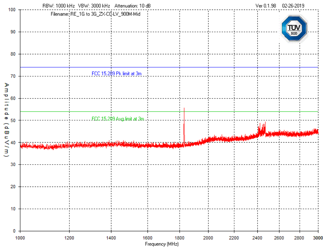
Graph 44 Test Results – Tx Spurious emission 1GHz – 3GHz: Mid Channel ZX Low Voltage Thermostat (900MHz) – Horizontal Polarization
