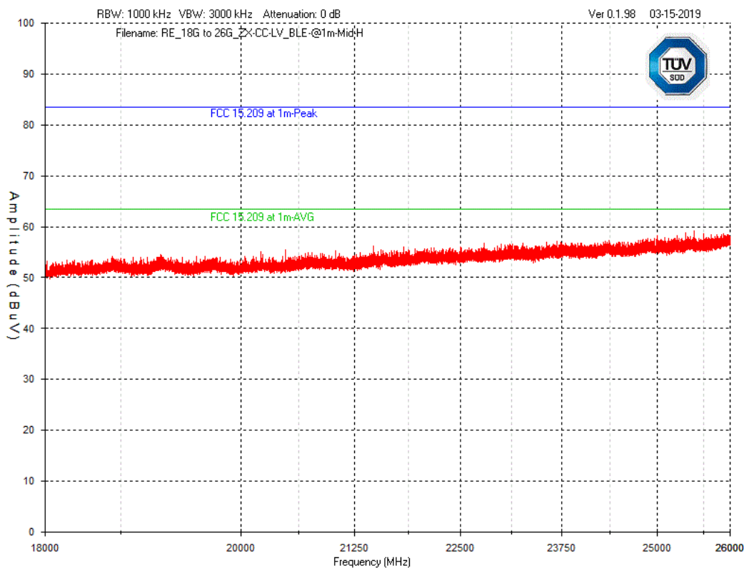
Graph 54 Test Results – Tx Spurious emission 18GHz – 26GHz: Mid Channel ZX Low Voltage Thermostat (2.4GHz) – Horizontal Polarization
