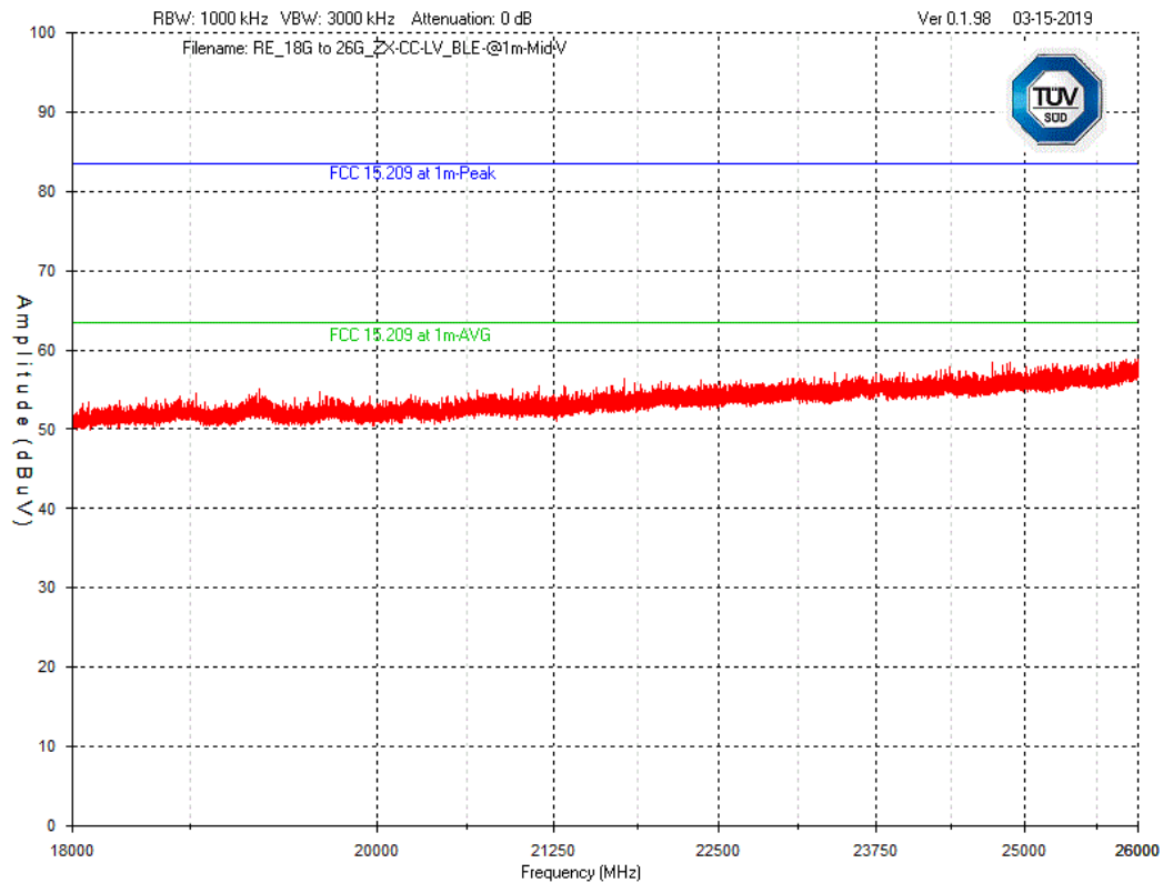
Graph 55 Test Results – Tx Spurious emission 18GHz – 26GHz: Mid Channel ZX Low Voltage Thermostat (2.4GHz) – Vertical Polarization
