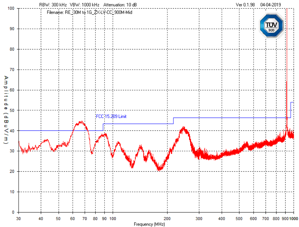
Graph 41 Test Results – Tx Spurious emission 30MHz – 1GHz: Mid Channel ZX Low Voltage Thermostat (900MHz) – Vertical Polarization
