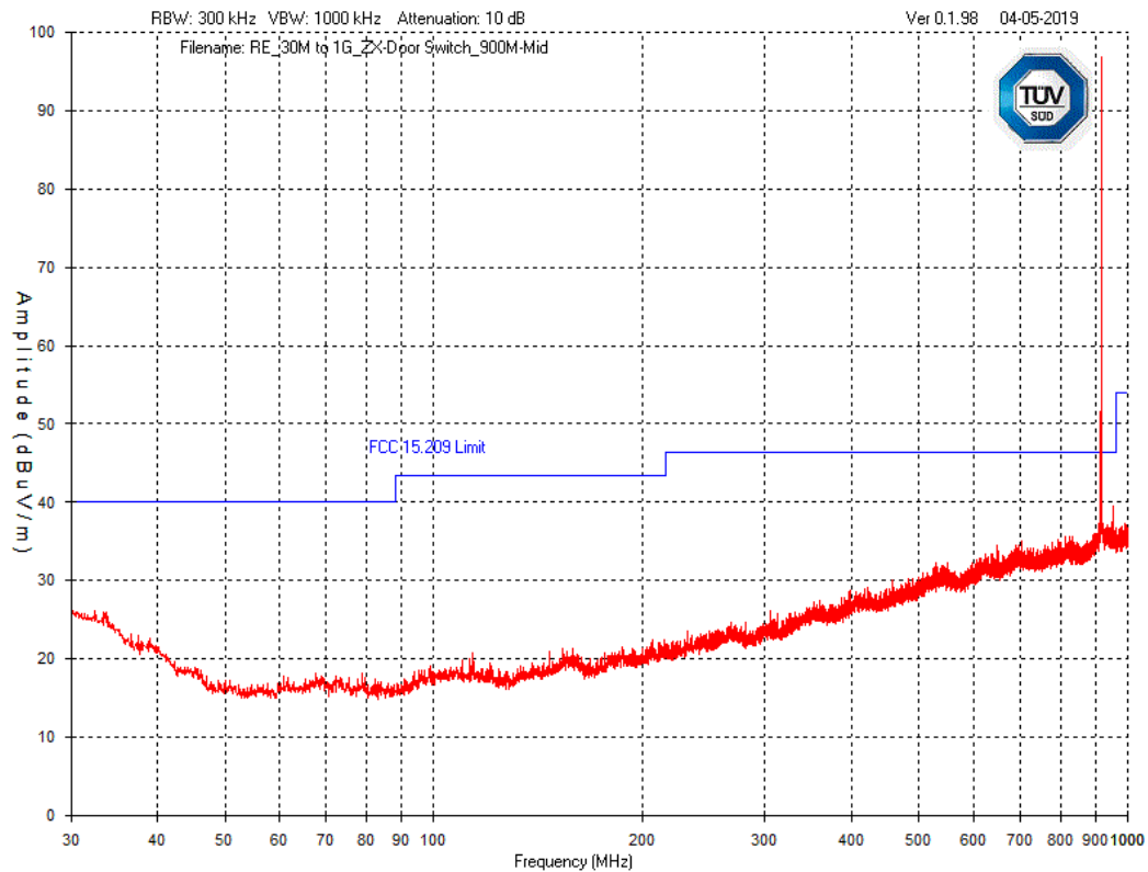
Graph 20 Test Results – Tx Spurious emission 30MHz to 1GHz – Mid Channel – Horizontal Polarization
