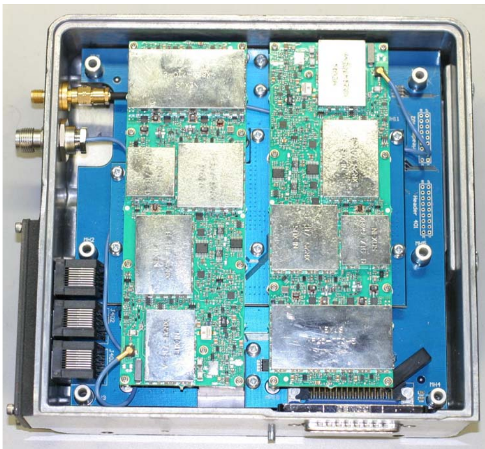
Figure 10 Internal with Carrier/Daughter and Transceiver Boards
