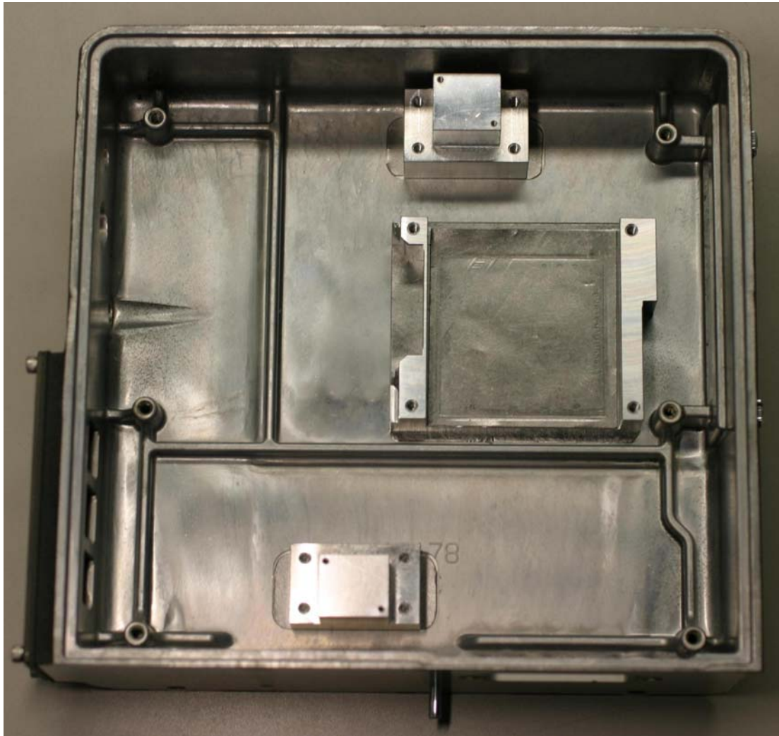
Figure 8 Internal Base showing Heatsinking
