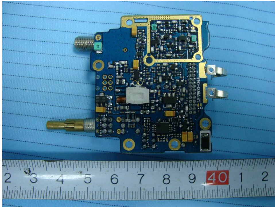
EUT – RF Board Components Bottom View
