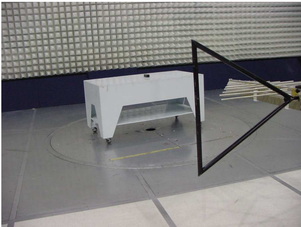
Test Setup Photos – Radiated Emissions
