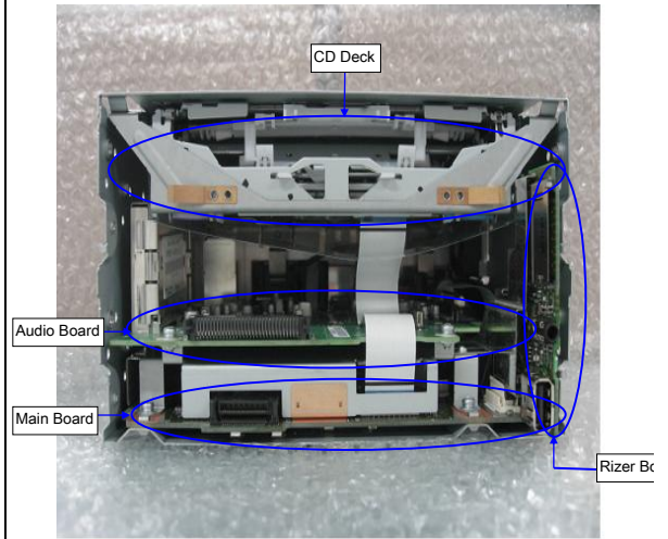
NA08A01 Board Positional View
