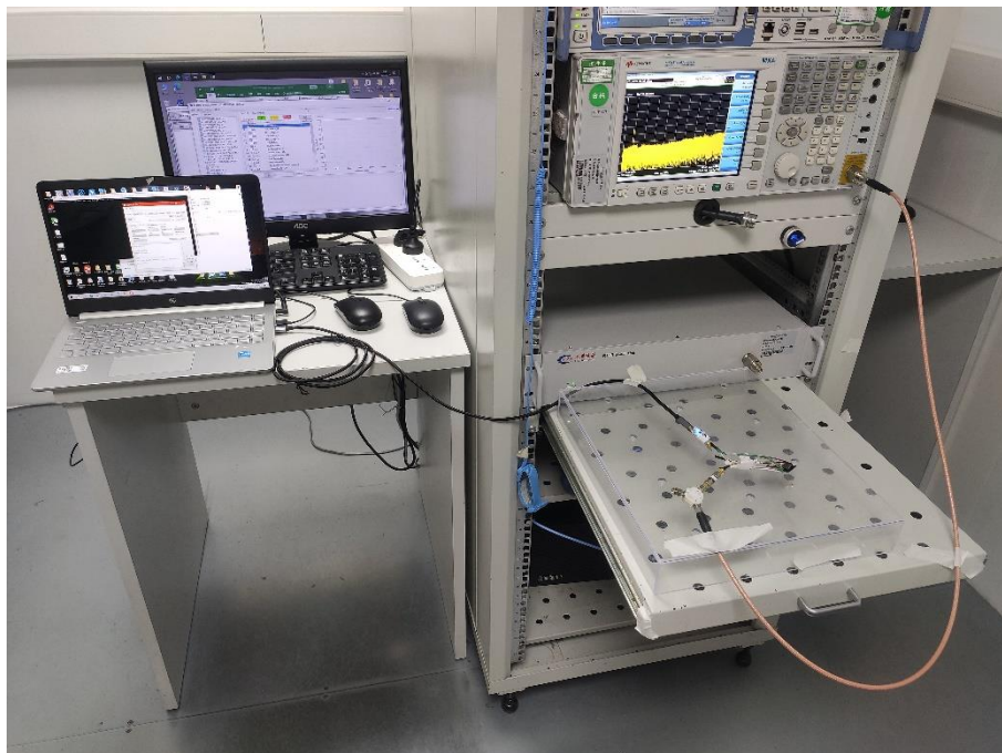
Conducted Test-RFID
