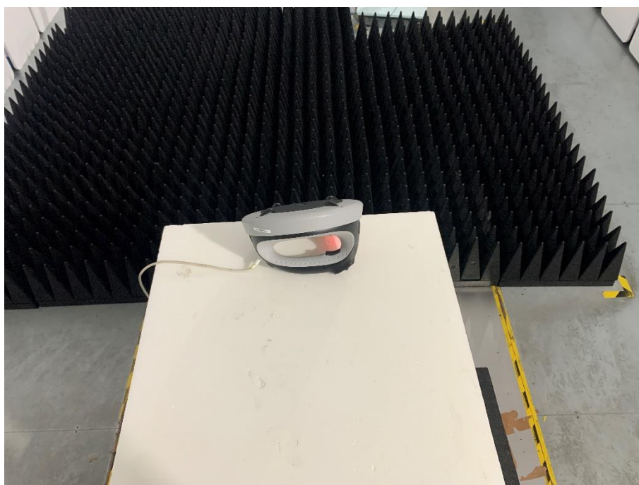
Close-up-BT/RFID
