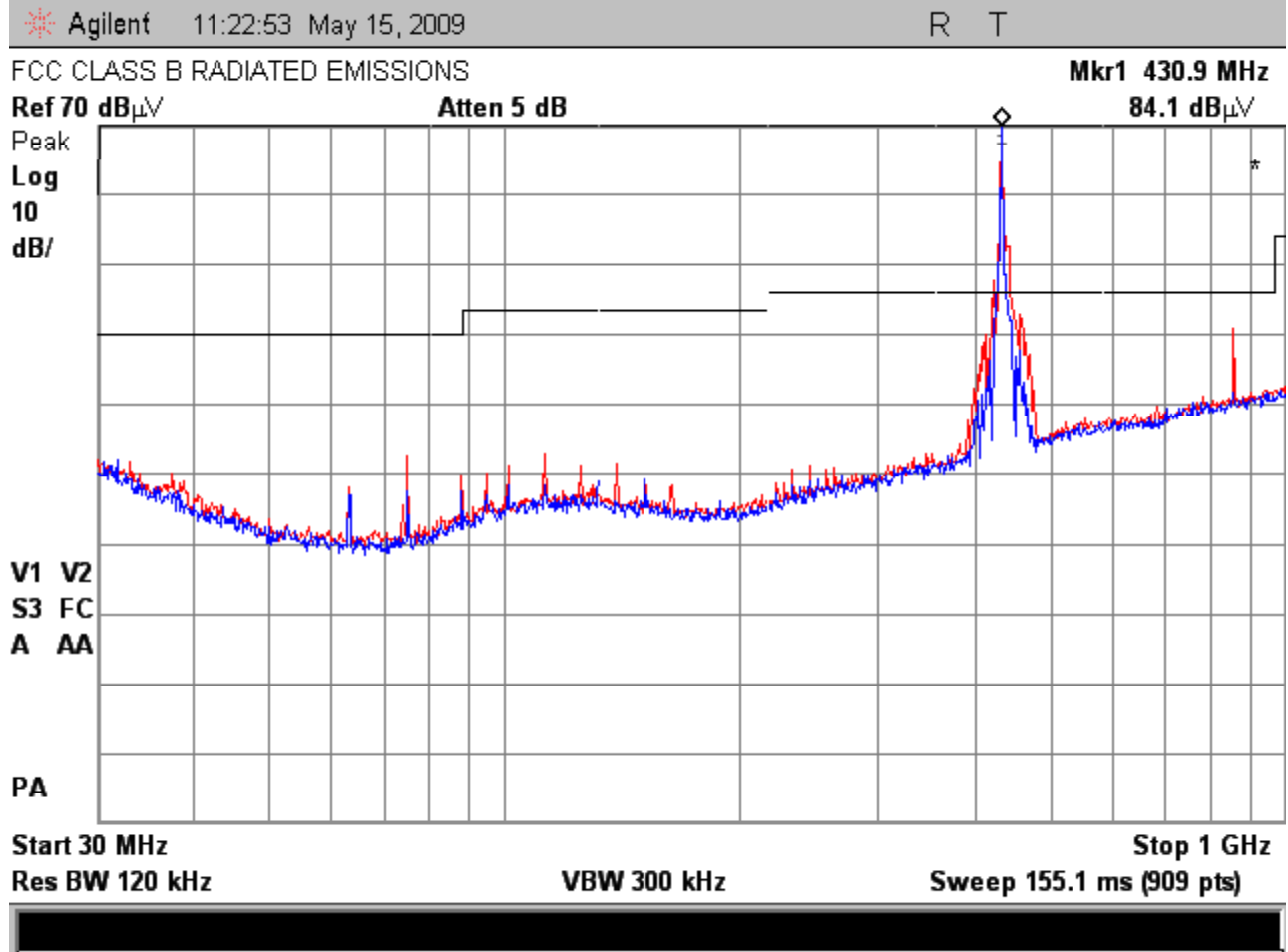
Figure 6.2-1 – Peak Detector Radiated Emissions 30 MHz to 1000 MHz
