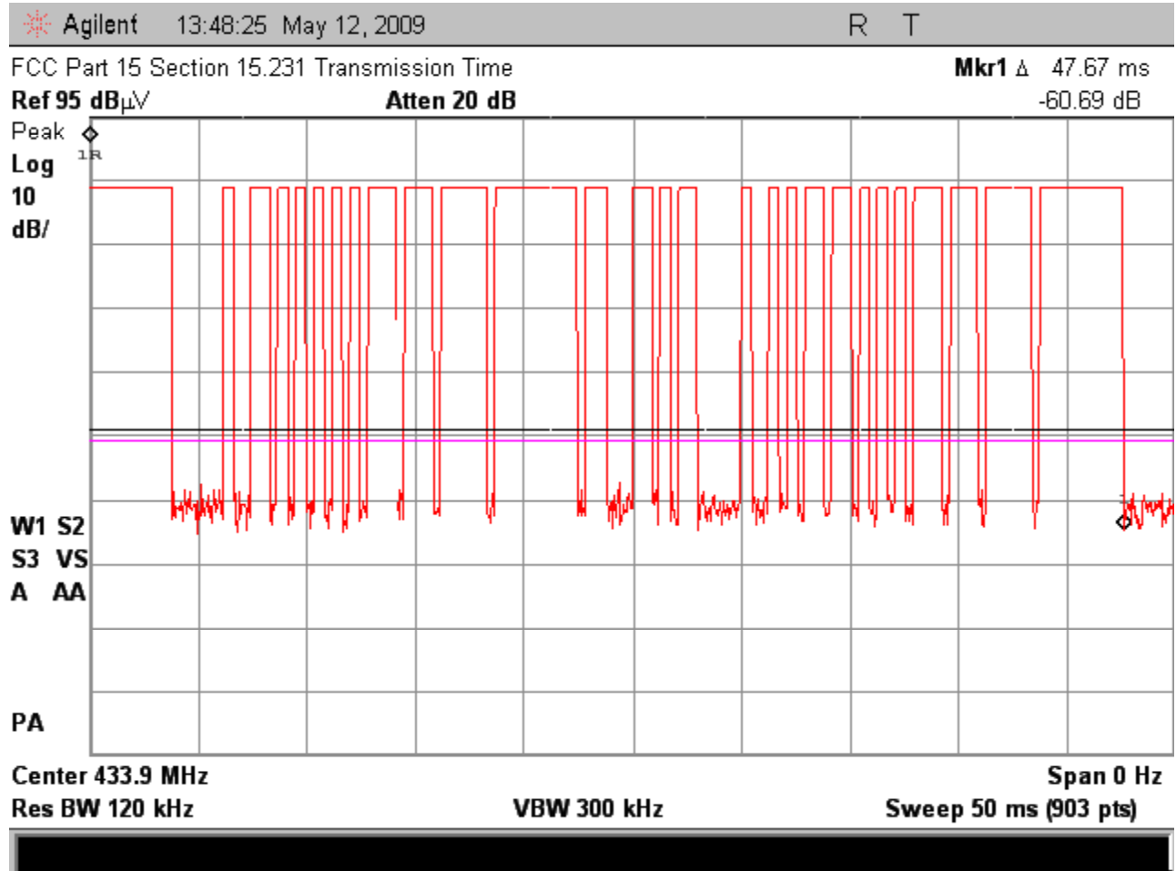
Figure 7.2-4 – Zoomed Plot of the Rain Detect Transmission Event
