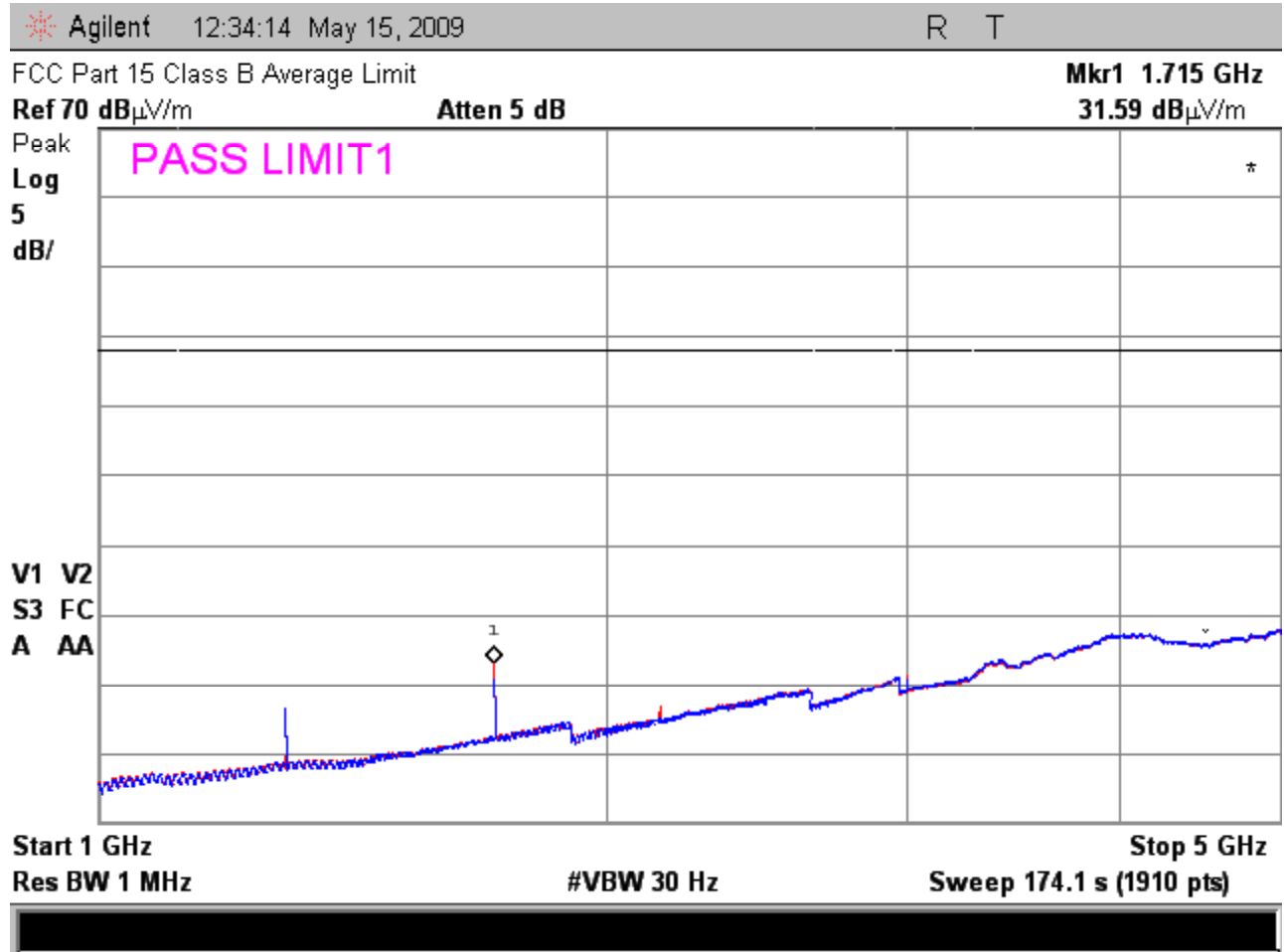
Figure 6.2-3 – Average Detector Radiated Emissions 1 – 5 GHz
