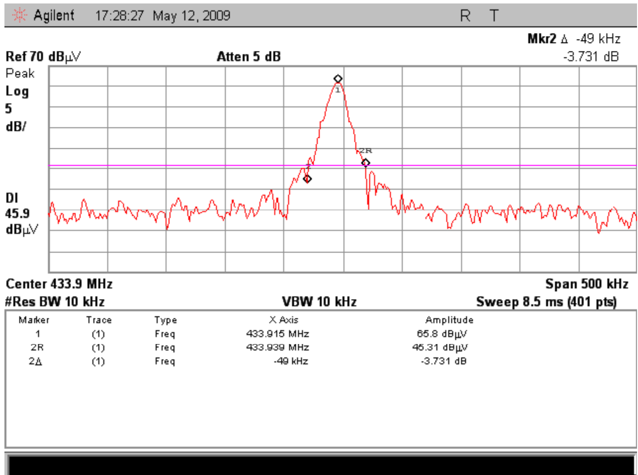
Figure 8.2-1 – 20 dB Bandwidth
