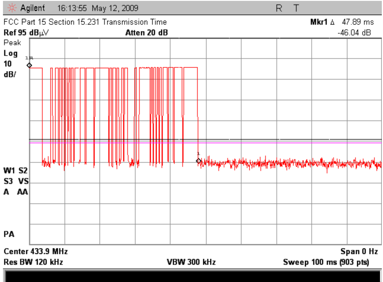
Figure 7.2-3 – Zoomed Plot of the Initial Set-up Transmission Event
