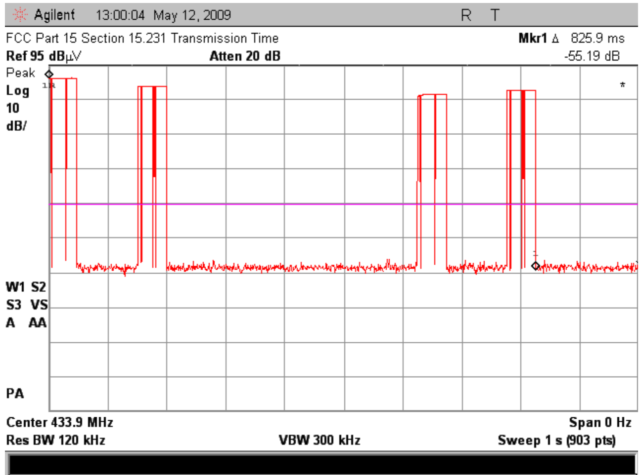
Figure 7.2-1 – Plot of the Rain Detect Transmission Event
