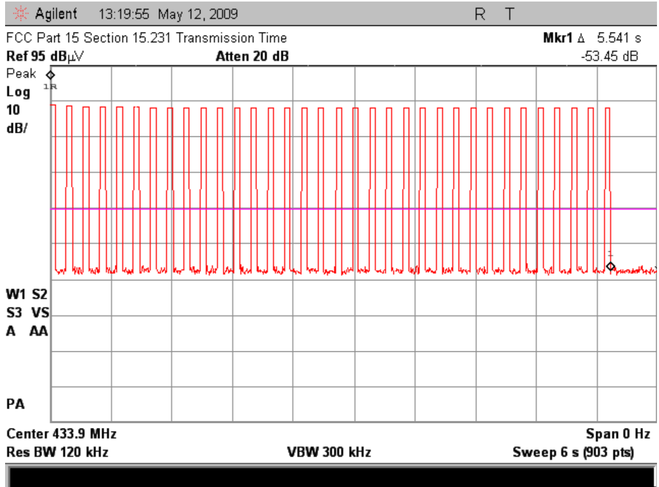
Figure 7.2-2 – Plot of the Initial Set-up Transmission Event
