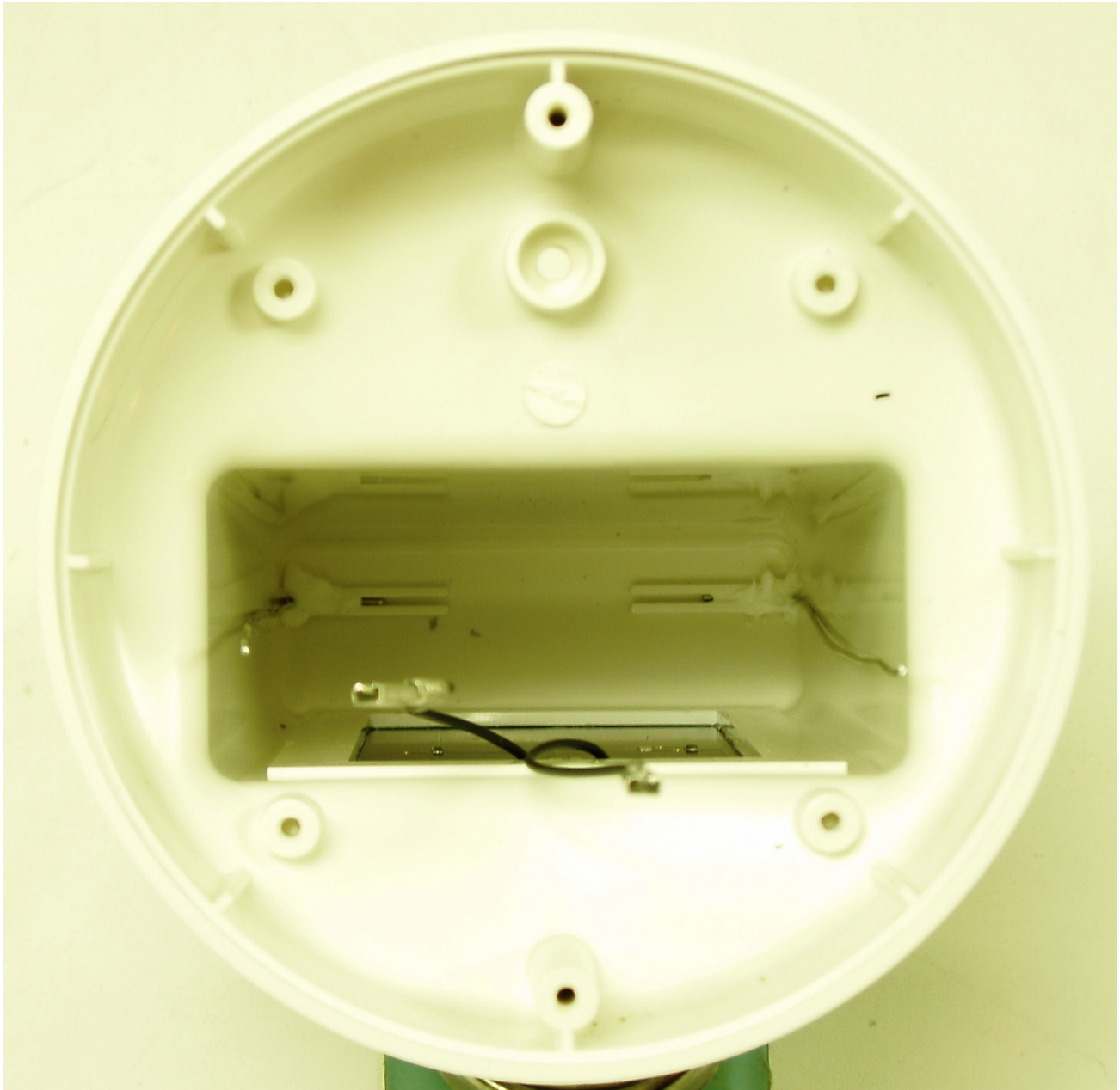
Photo 3 – View of the Internal Antennas
