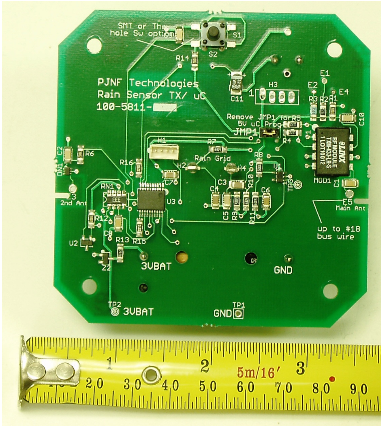
Photo 1 – Top Side of the Circuit Board
