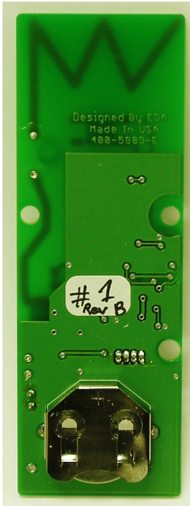
Photo 2 – Bottom Side of the Circuit Board
