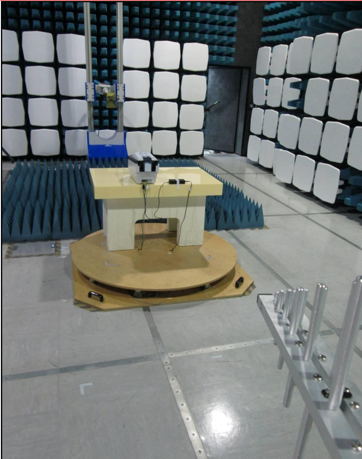
PHT\12247063JD01\002 - Test Configuration Photograph - Radiated Emissions 002
