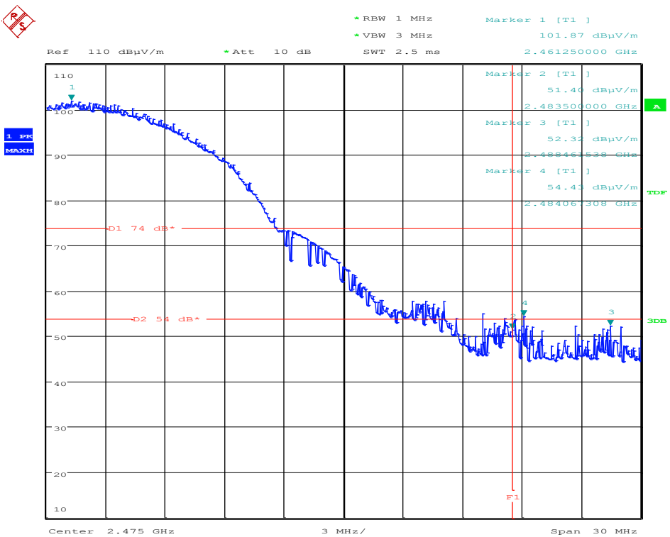
Upper Bandedge – Peak Detector
