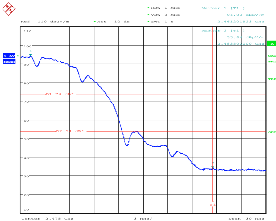
Upper Bandedge – Average Detector
