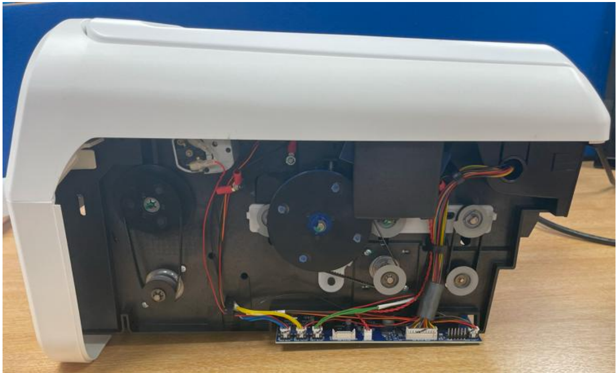
Figure 7: Magicard K Right side
