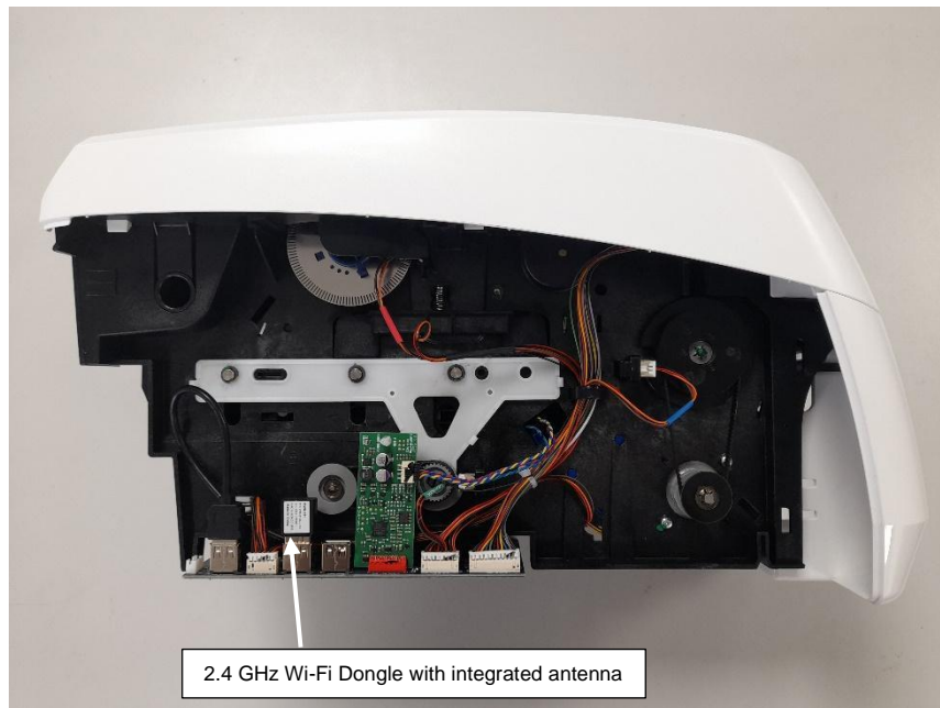
Figure 1: Magocard 600 Left side
