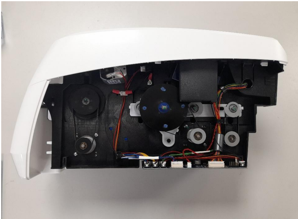
Figure 5: Magicard 600 Right side
