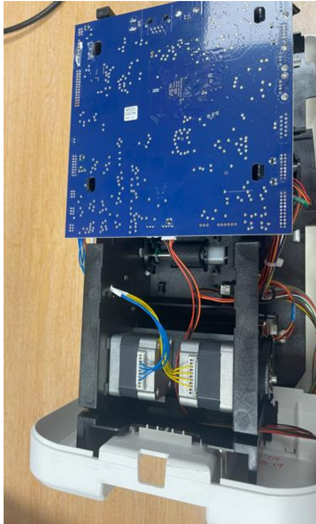
Figure 13: Magicard D Underside
