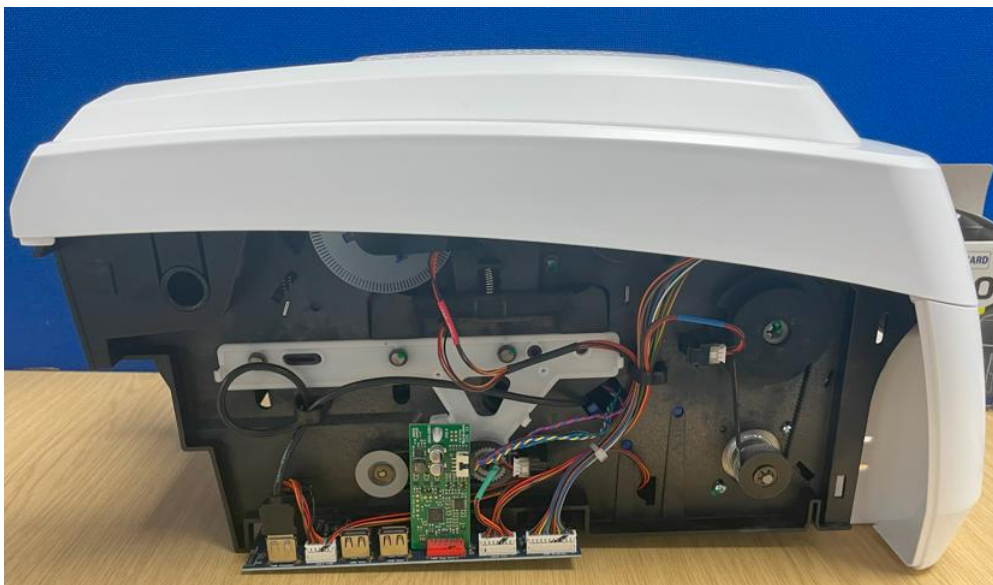
Figure 2: Magocard 300 Left side
