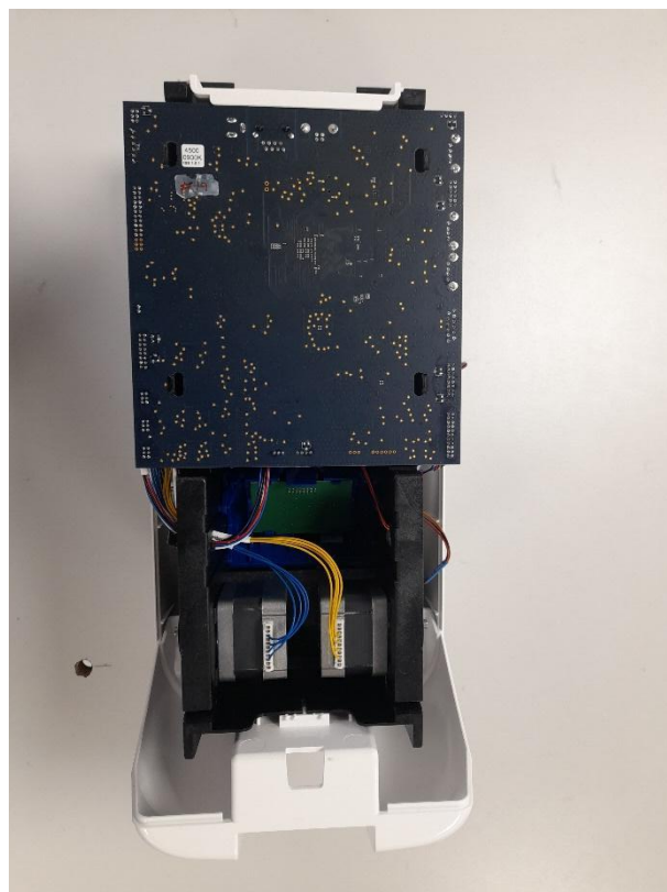
Figure 10: Magicard 600 Underside
