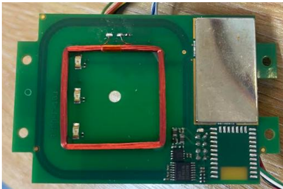
Figure 15: Underside of Elatec Smart Code Encoder PCB (PCB removed from product)
