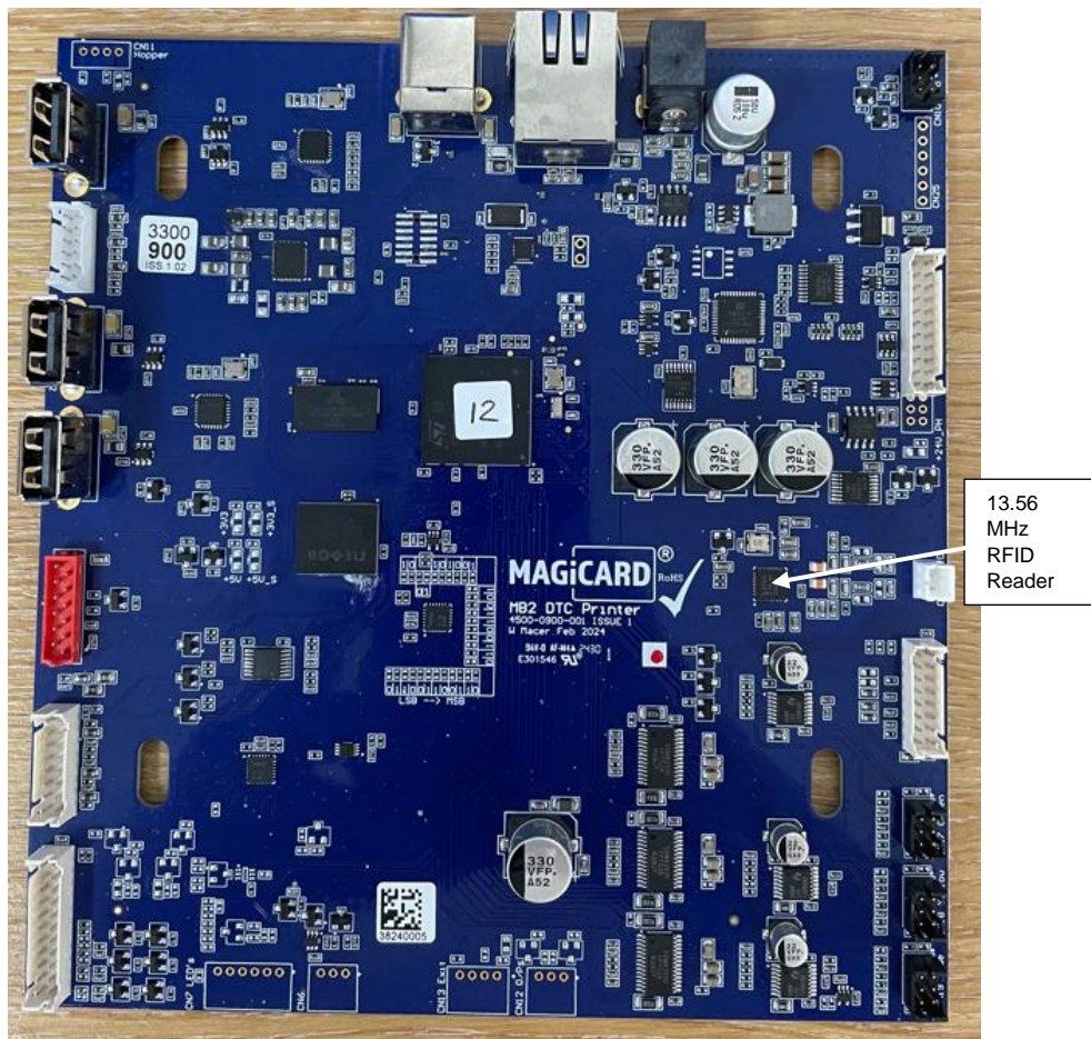
Figure 14: Top Side of Main PCB (PCB removed from product)
