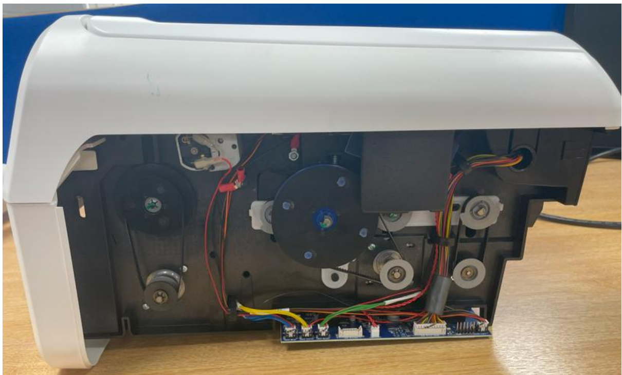
Figure 8: Magicard D Right side
