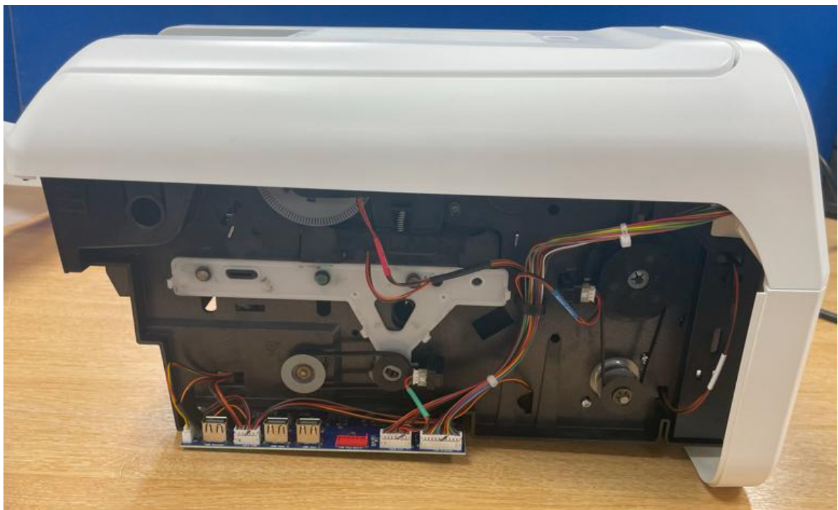
Figure 4: Magicard D Left side
