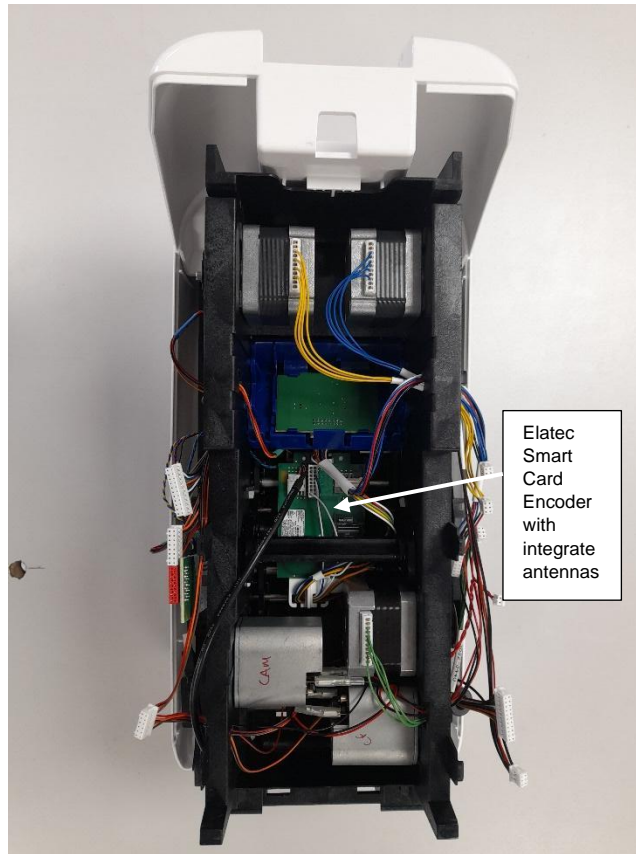
Figure 9: Magicard 600 Underside (main PCB removed) (View Representative of all models)
