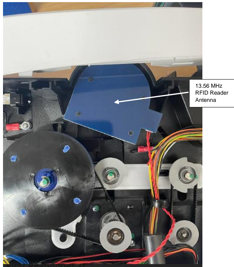
Figure 16: Close-Up view of view of RFID Antenna installed in product
